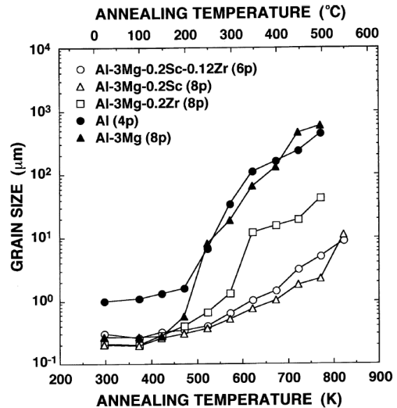
Fig. 2 Grain size versus annealing temperature for samples annealed for one hour after ECAP through 4, 6 or 8 passes (p) [19].
