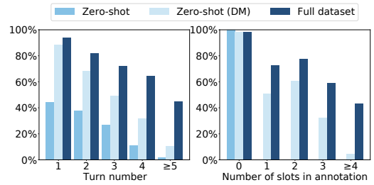
Figure 3: Breakdown of accuracy by turn number and number of slots of the TRADE model on the “Restaurant” domain. “Zero-shot” results are trained by withholding in-domain data, and “Zero-shot (DM)” is our data synthesis based on the Dialogue Model. “Full dataset” refers to training with all domains.
