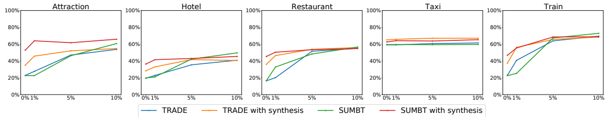
Figure 4: Accuracy plots for the few-shot MultiWOZ experiments. X axis indicates the percentage of real target domain data included in training. Y axis indicates joint accuracy.
