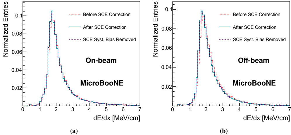
Figure 24. distribution for stopping muons in both (a) on-beam and (b) off-beam events, looking both before and after the SCE calibration described in the text is applied; these distributions are also shown after accounting for the estimated systematic bias in the measurement.
