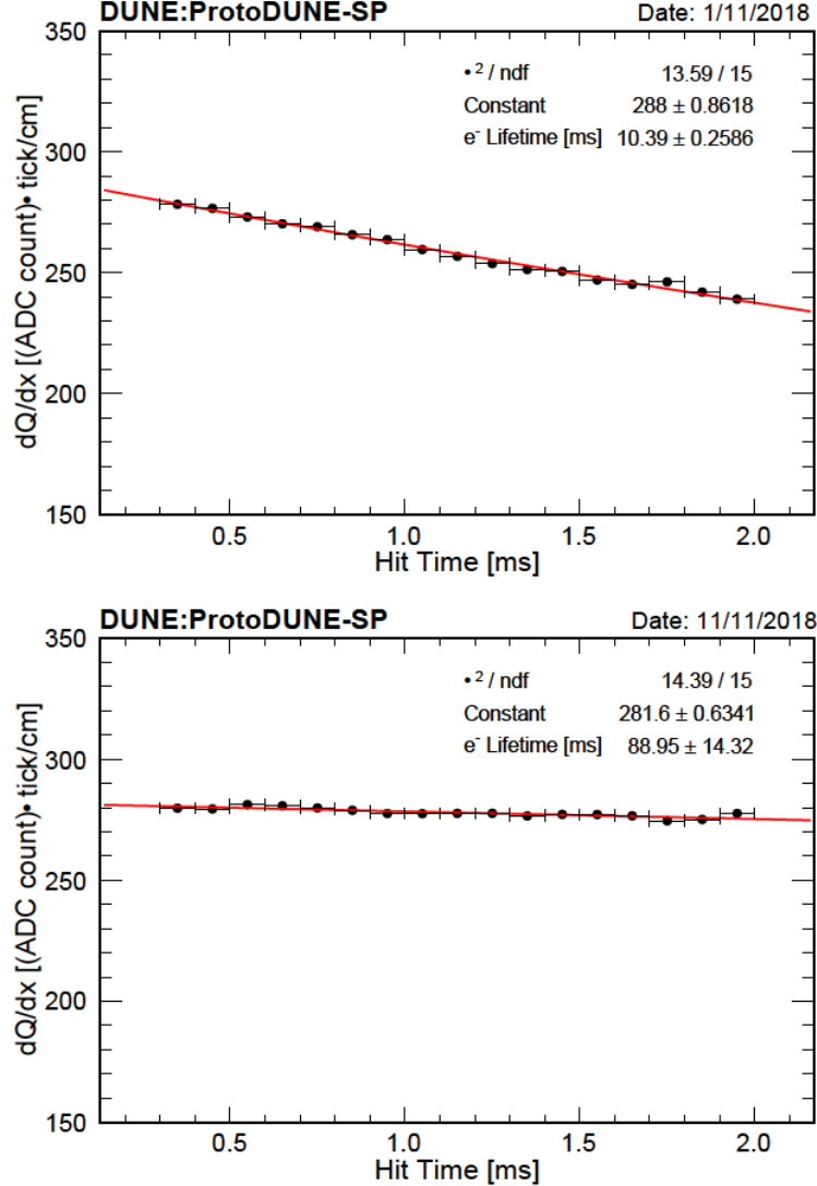
Figure 53. Plot the MPV of the dQ/dx distribution as a function of the hit time, fit to an exponential decay function on November 1st, 2018 during a period of lower purity (top) and on November 11th, 2018 during a period of higher purity (bottom). Only statistical errors are included.
