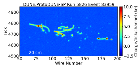
(a) A 0.5 GeV/ electron candidate.
