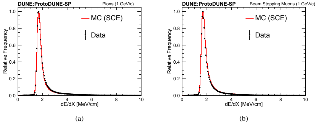
Figure 62. Pion (a) and stopping muon (b) distributions for the ProtoDUNE-SP beam data after applying the calibration derived using cosmic-ray muons. The distribution for replica selections on a beam Monte Carlo sample with space charge effect simulated is also shown. The histograms are normalized such that the maximum frequency is one.
