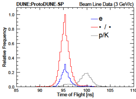
(c) Nominal beam momentum = 3 GeV/c.
