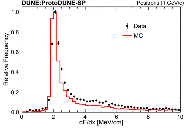
Figure 66. at the beginning of the shower. The histograms are normalized such that the maximum frequency is one.
