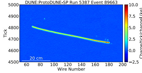
(e) A 1 GeV/ stopping proton candidate.
