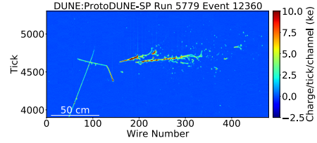
(f) A 2 GeV/ pion charge exchange candidate.
