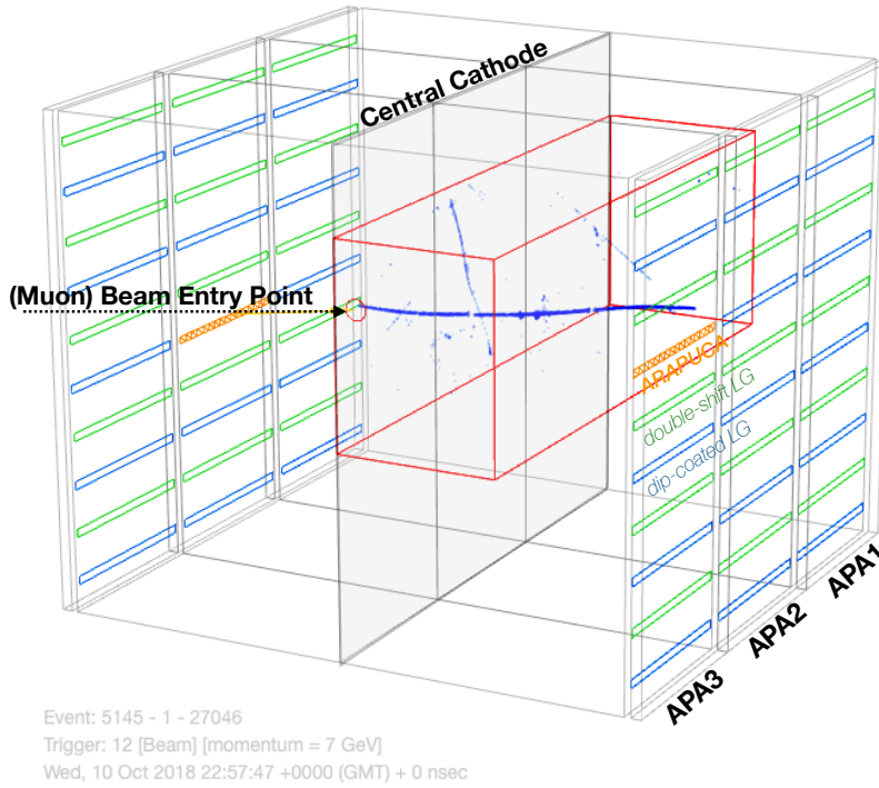
Figure 39. 3D event display made with the Wire-Cell BEE display [54] showing data from a 7 GeV/ beam muon crossing the whole TPC volume, fully reconstructed by the LArTPC. Only tracks inside a predefined sub-volume (red box) are shown. The beam muon track enters near the cathode and propagates along the beam direction about 10 downward and 11 toward the anode plane. Ten bars are located in each APA frame. The dip-coated bars are indicated in blue, the double-shift bars in green and the segmented ARAPUCA bar in orange.
