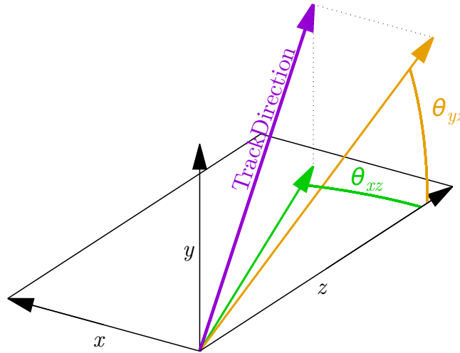
Figure 27. The definitions of the track direction angles and .
