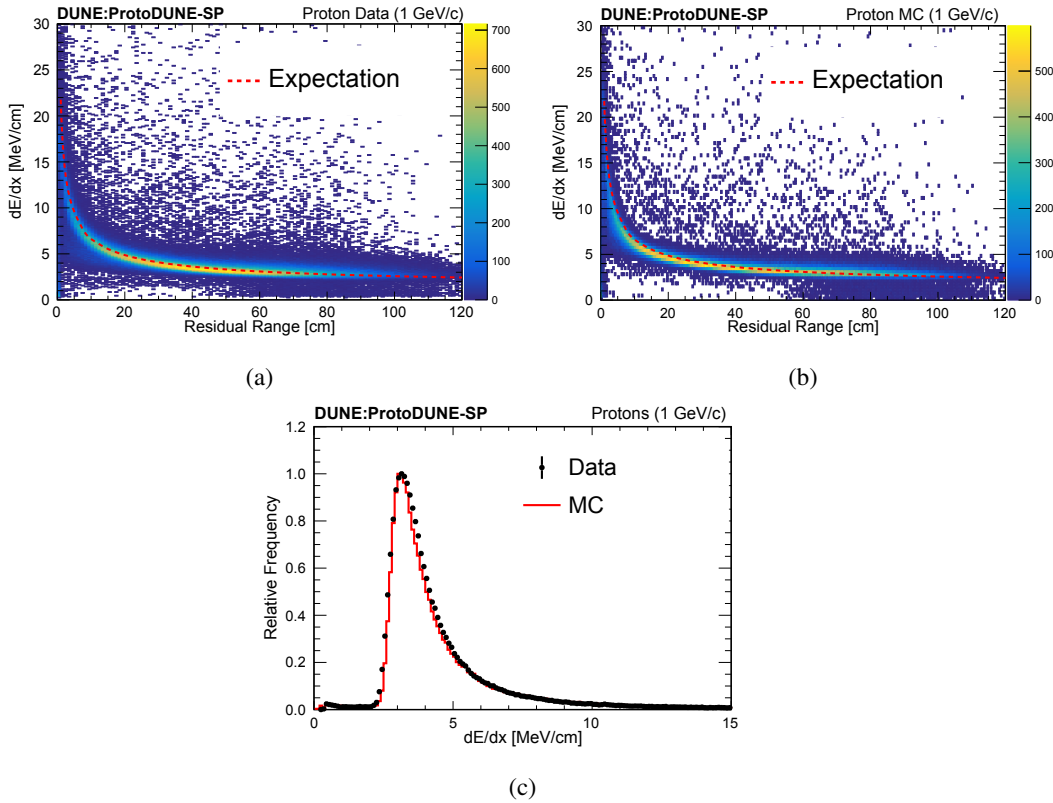
Figure 65. Stopping proton versus residual range distributions for the ProtoDUNE-SP beam data (a) and MC (b), the expected most probable values are shown in red. The distributions after the SCE corrections of data and MC are shown in (c). The histograms in (c) are normalized such that the maximum frequency is one.
