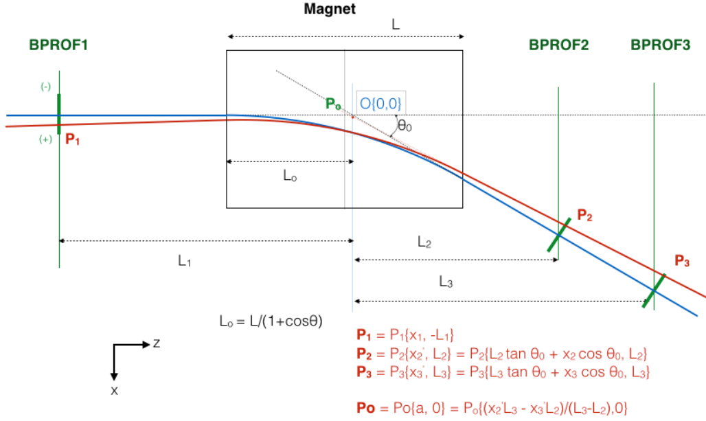
Figure 10. A schematic diagram showing the method by which momentum is reconstructed for a given beam particle (red), as discussed in the text. Taken from [30]. The direction of the x -axis is opposite to the convention used in this paper.
