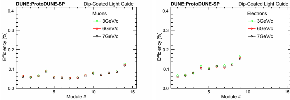
Figure 43. Efficiency measurements of 14 dip-coated light-guide modules (PDS beam side), as determined from beam muons (left) and beam electrons (right) data at different momenta (only modules 1–9 in APA3, and 2 at the shorter distance from the shower and higher photon counting are displayed).
