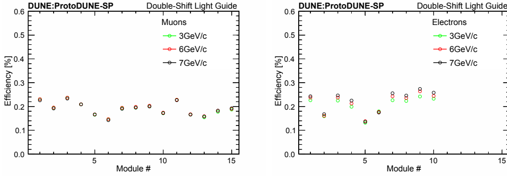
Figure 42. Efficiency measurements of 15 double-shift light-guide modules (PDS beam side), as determined from beam muons (left) and beam electrons (right) data at different momenta (only modules 1–10 in APA3, and 2 at the shorter distance from the shower and higher photon counting are displayed).
