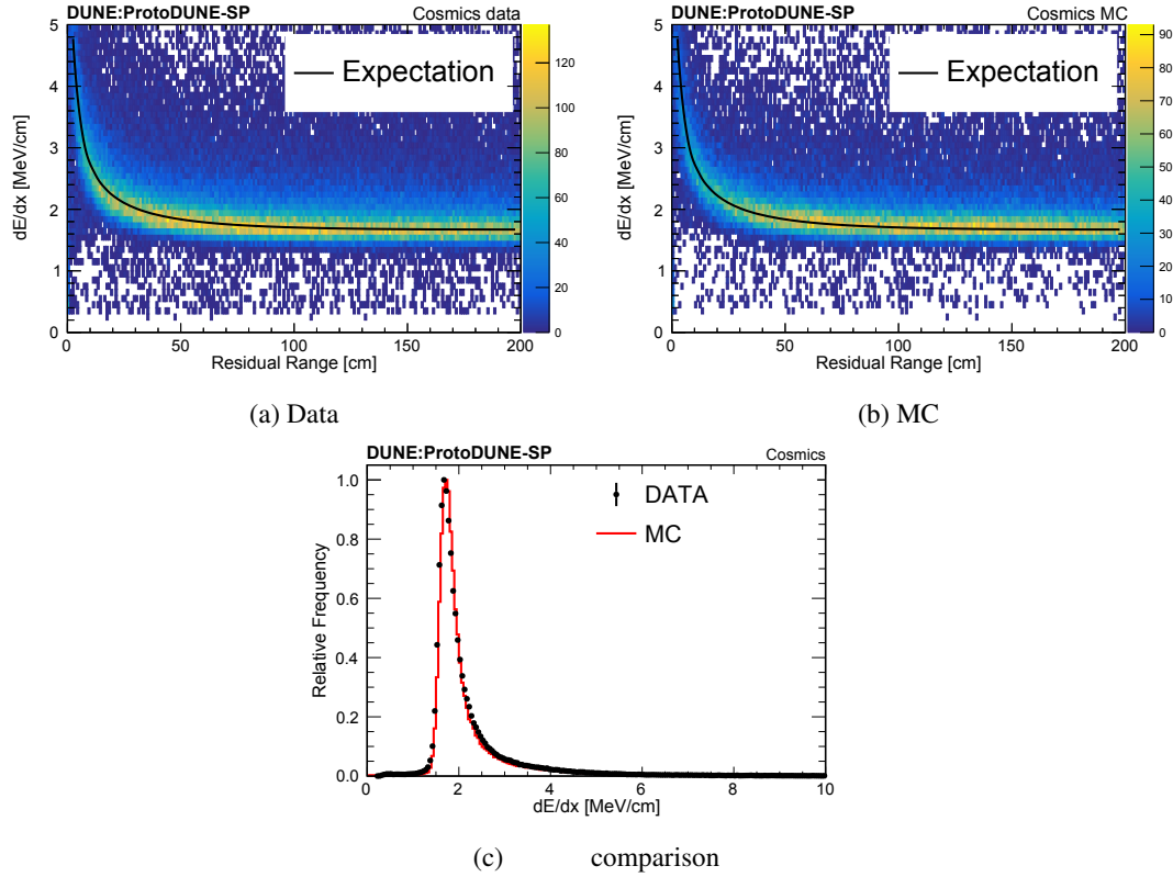
Figure 60. Stopping muon distributions for the ProtoDUNE-SP cosmic-ray data and MC. The black curves in (a) and (b) are the predicted most probable values (using the Landau-Vavilov function) of versus residual range and (c) is the distribution for the stopping muon sample. The histograms in (c) are normalized such that the maximum frequency is one.
