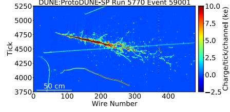
(b) A 6 GeV/ electron candidate.
