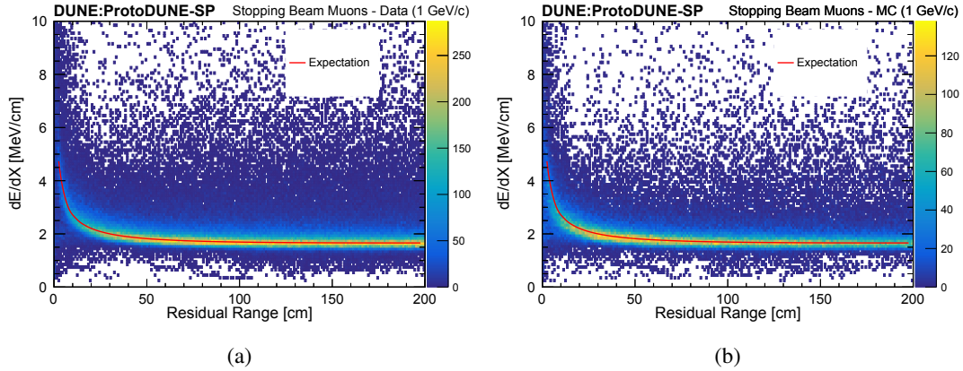
Figure 63. vs residual range for selected stopping muons in the 1 GeV/ beam after applying the calibration derived using cosmic-ray muons, in data (a) and MC (b). The expected most probable value of is plotted as a function of residual range for both.
