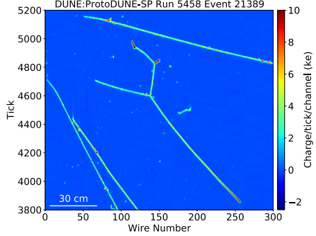
(c) A 1 GeV/ pion candidate.
