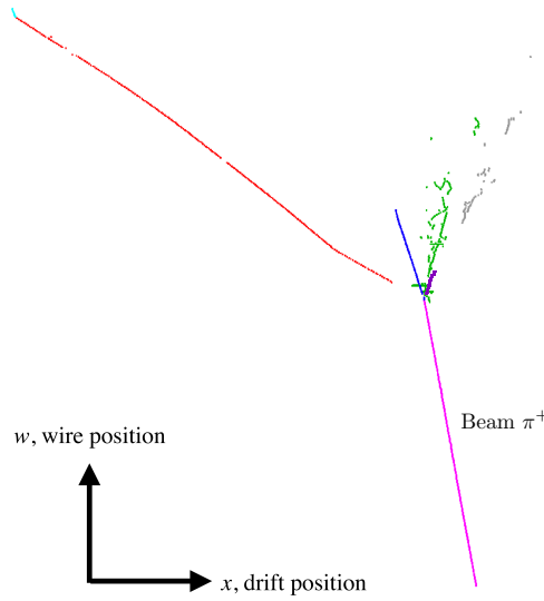
Figure 26. A reconstructed, simulated test-beam interaction showing the incoming beam track in magenta and a number of secondary particles created at the interaction vertex. The different colors represent different reconstructed particles.
