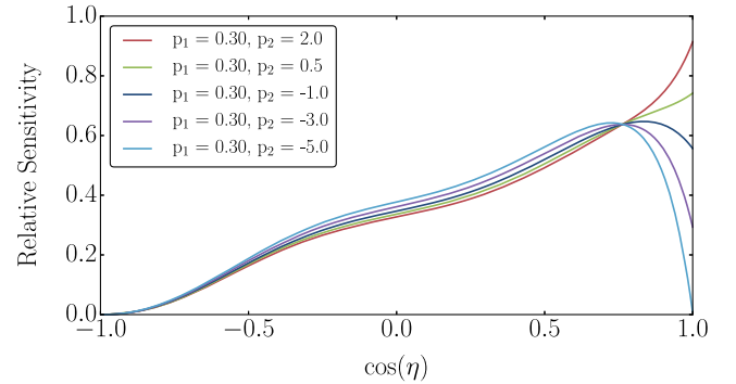
FIG. 12. DOM angular efficiency variations. Different allowed angular acceptance curves are shown as a function of the incident photon angle.
