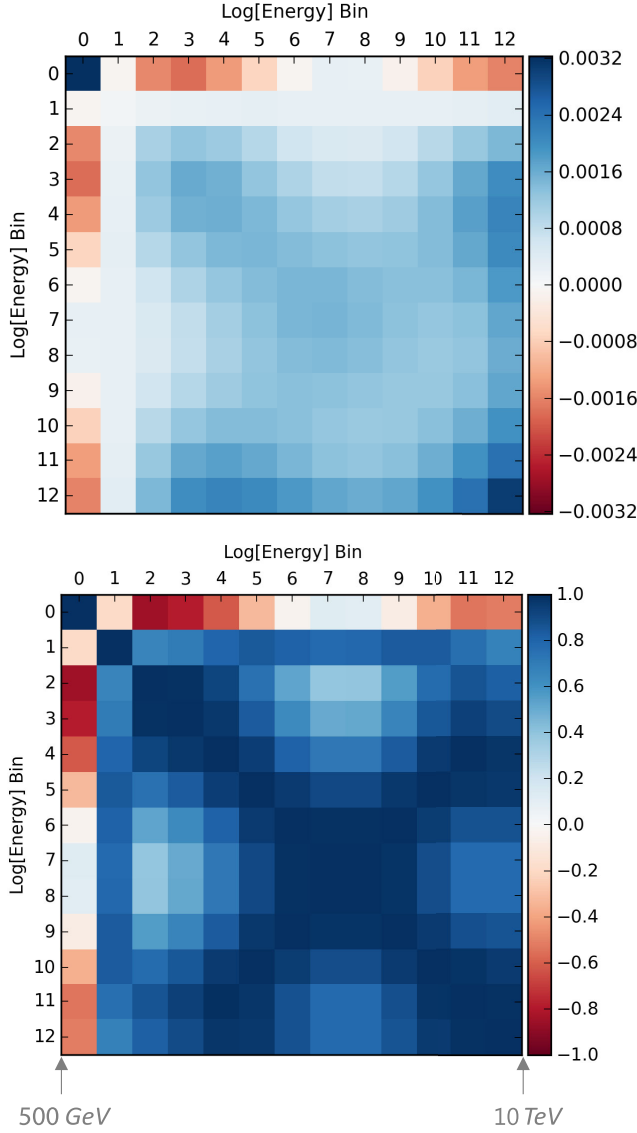
FIG. 11. Energy distribution ice uncertainty covariance (top) and correlation matrix (bottom). The color scale shows the covariance and correlation between energy bins.
