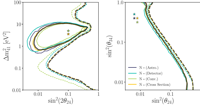
FIG. 25. Effect of removing a systemic category on the frequentist results. Each color line corresponds to the analysis performed without a single systematic group and the star of the same color is the corresponding best-fit point. Left: analysis I; right: analysis II. The solid (dashed) lines show the 90% C.L. (99% C.L.). The solid black lines represent the frequentist result using all years.
