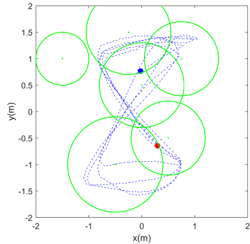
Fig. 3: Projected x-y trajectory of the GT-MAB in the designated workspace. Virtual beacon ranges are plotted as green circles and the GT-MAB trajectory is shown in dotted blue. Starting and ending positions of the GT-MAB are given by the blue and red dots.
