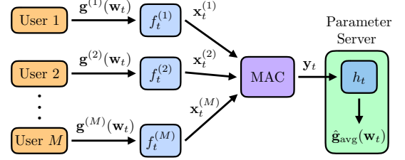
Fig. 1: FL over a MAC. At each iteration, users send their local gradients \mathbf{g}^{(m)}(\mathbf{w}_t) through a MAC. The PS aggregates the gradients, updates the model and sends the updated model back to users for subsequent iteration.
