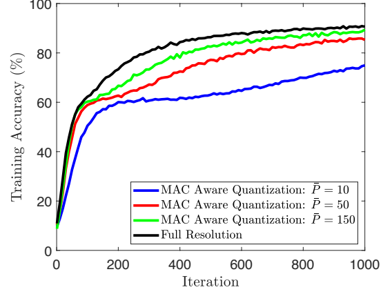
Fig. 5: Training accuracy comparison for MAC aware gradient quantization with total power per iteration \bar{P} = 10, 50, 150 , and P_1 = 0.8\bar{P} and P_2 = 0.2\bar{P} .
