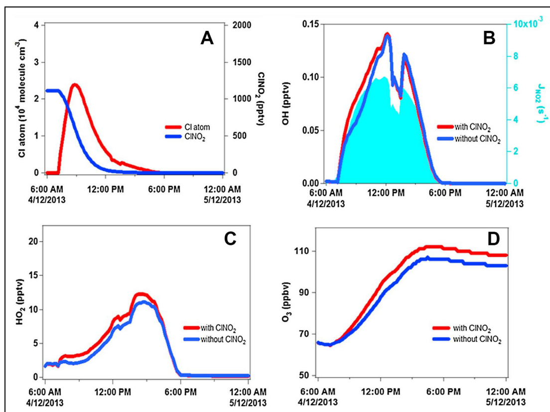
Figure 11. Model-simulated concentrations/mixing ratios of (a) \text{ClNO}_2 and \text{Cl} , (b) \text{OH} , (c) \text{HO}_2 , and (d) ozone during the day following plume sampling from the Mt. Tai Mao Shan site (957 m a.s.l) in Hong Kong, with and without the inclusion of \text{ClNO}_2 chemistry. The measured photolysis rate constant of \text{NO}_2 is shown by the light blue shading. The model was initiated with the measured concentrations of \text{ClNO}_2 and other relevant chemical constituents at 06:00. Adapted from Wang et al. (2016). DOI: https://doi.org/10.1525/elementa.2020.034.f11
