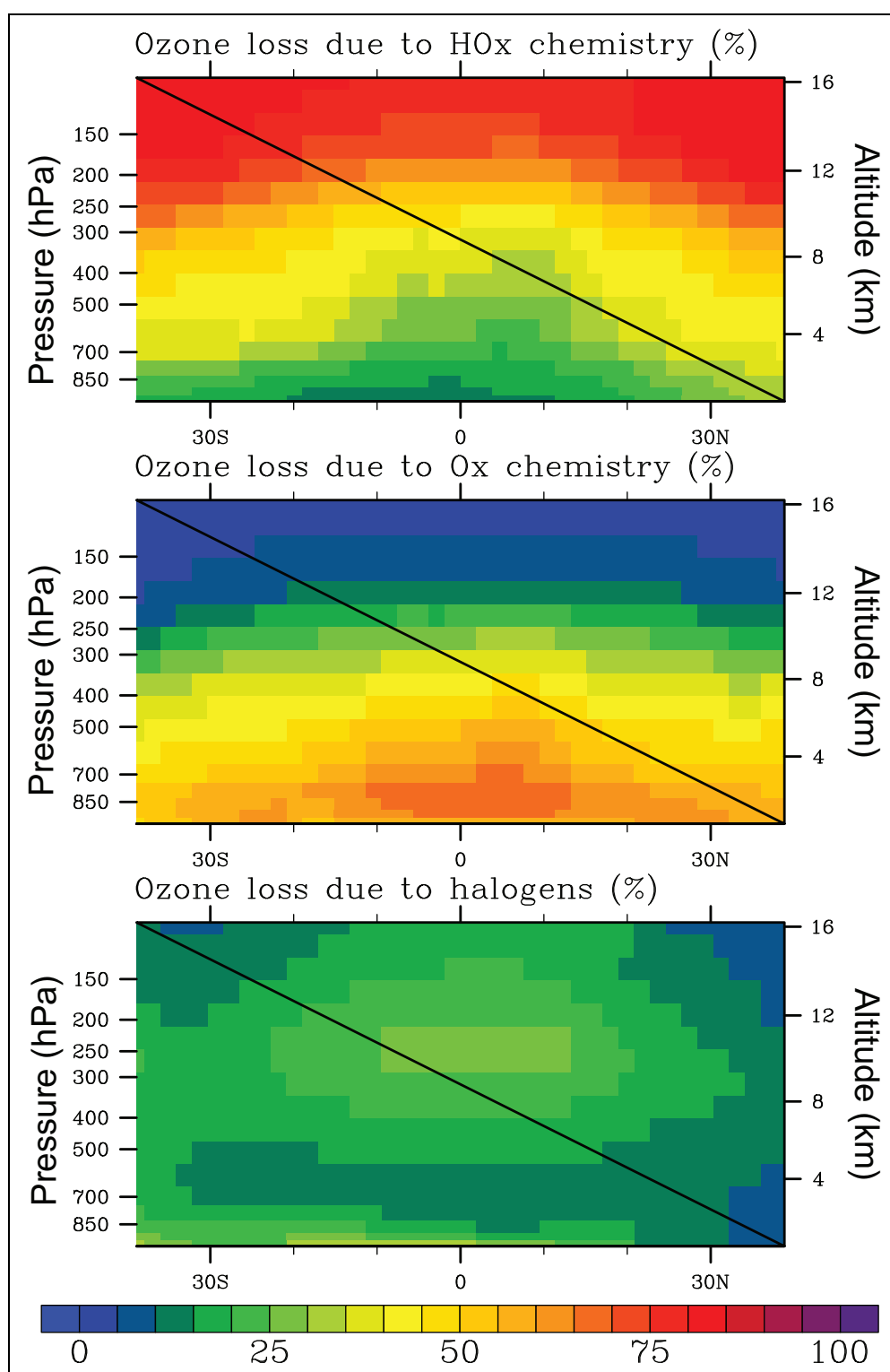
Figure 14. Percentage contribution to chemical ozone loss from HO x , O 3 , and halogen photochemistry between 40°N and 40°S. Approximately 70% of the halogen-mediated ozone loss is calculated to be driven by iodine photochemistry. Adapted from Saiz-Lopez et al. (2012). DOI: https://doi.org/10.1525/elementa.2020.034.f14
