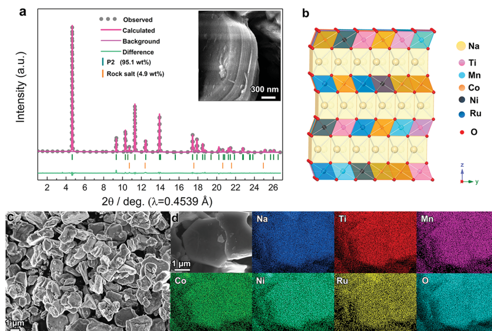
Figure 2. XRD and SEM of P2-TMCNR material. (a) SXR D and Rietveld refinement of the P2-TMCNR sample, inset in (a) shows the high magnification side view of particles. (b) The crystal structure of P2-TMCNR was drawn based on the refined model. (c) Low magnification SEM image of the P2-TMCNR sample. (d) EDS mapping of the P2-TMCNR sample and the corresponding SEM image.
