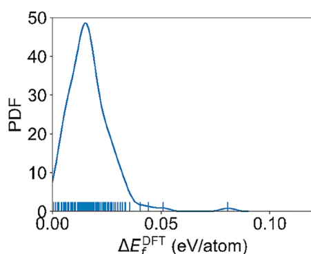
Figure 5. Probability distribution function (PDF) of DFT-calculated formation energy above the ground state (GS), i.e., \Delta E_f = E_f - E_f^{GS} for low-energy orderings of TMs and Na found by simulated annealing.
