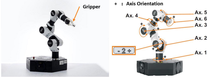
FIGURE 11: THE E.DO ROBOTIC ARM AND POSITIVE ORIENTATIONS OF SIX JOINTS.
