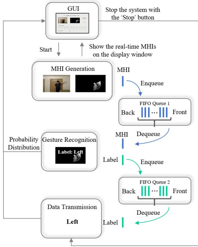
FIGURE 4: THE MULTI-THREADING MODEL OF THE REAL-TIME HRC SYSTEM.
