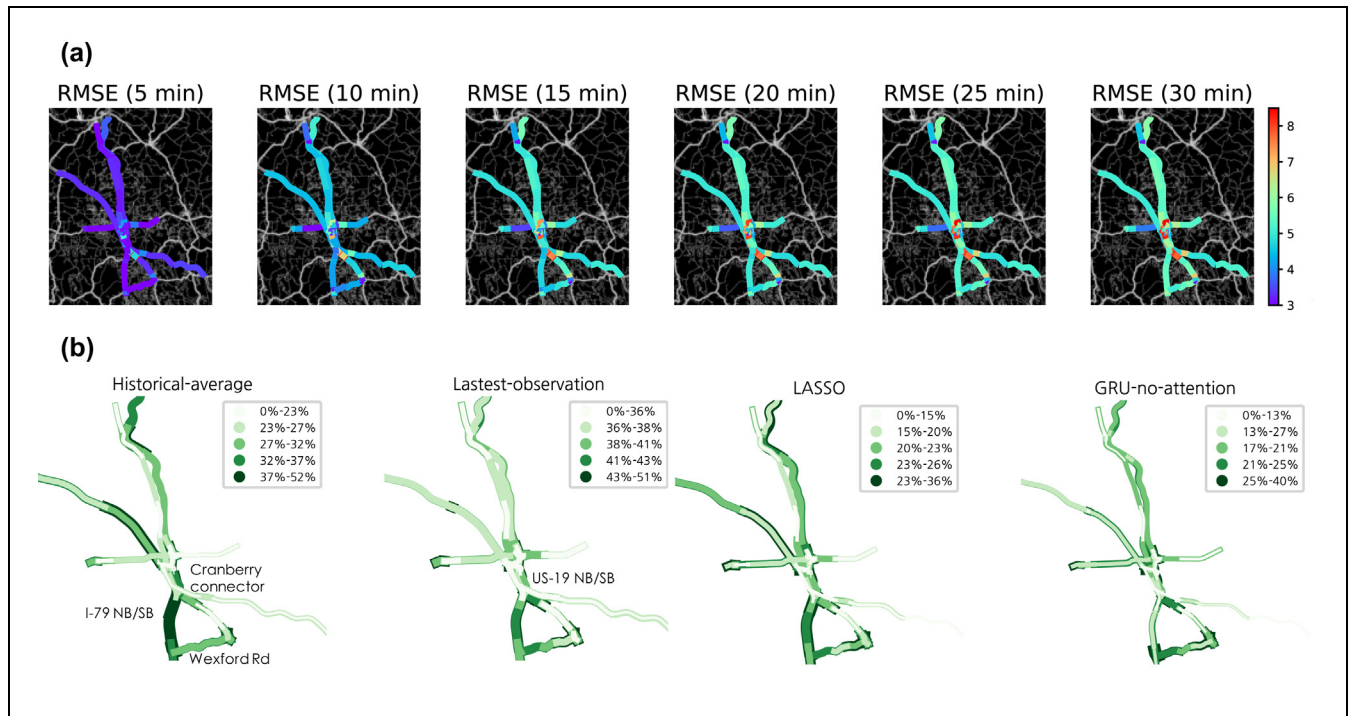
Figure 6. Visualization of traffic speed prediction model performances: (a) speed prediction performance of encoder-decoder-attention with 5–30 min prediction horizon, and (b) percentage improvement of the model against other baselines for 30-min ahead speed prediction.
