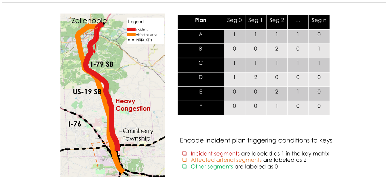
Figure 5. Encoding scheme of incident plan attributes and keys.
