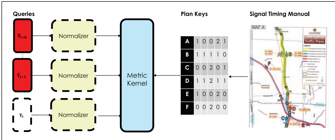
Figure 4. Plan associator architecture.
