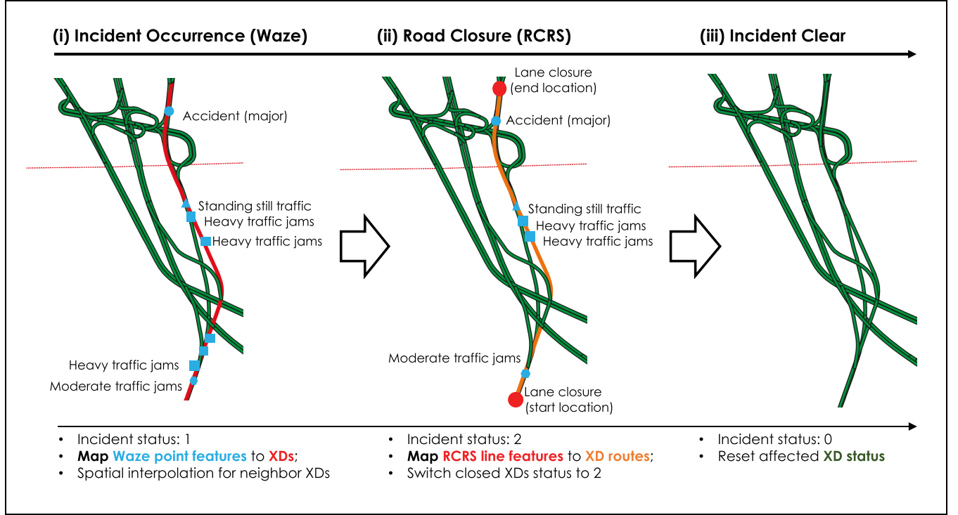
Figure 2. Workflow for integration of multi-source incidents.
