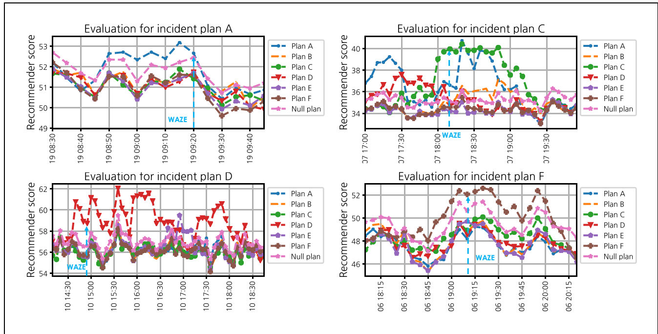
Figure 7. Visualization of plan recommender model performances.
