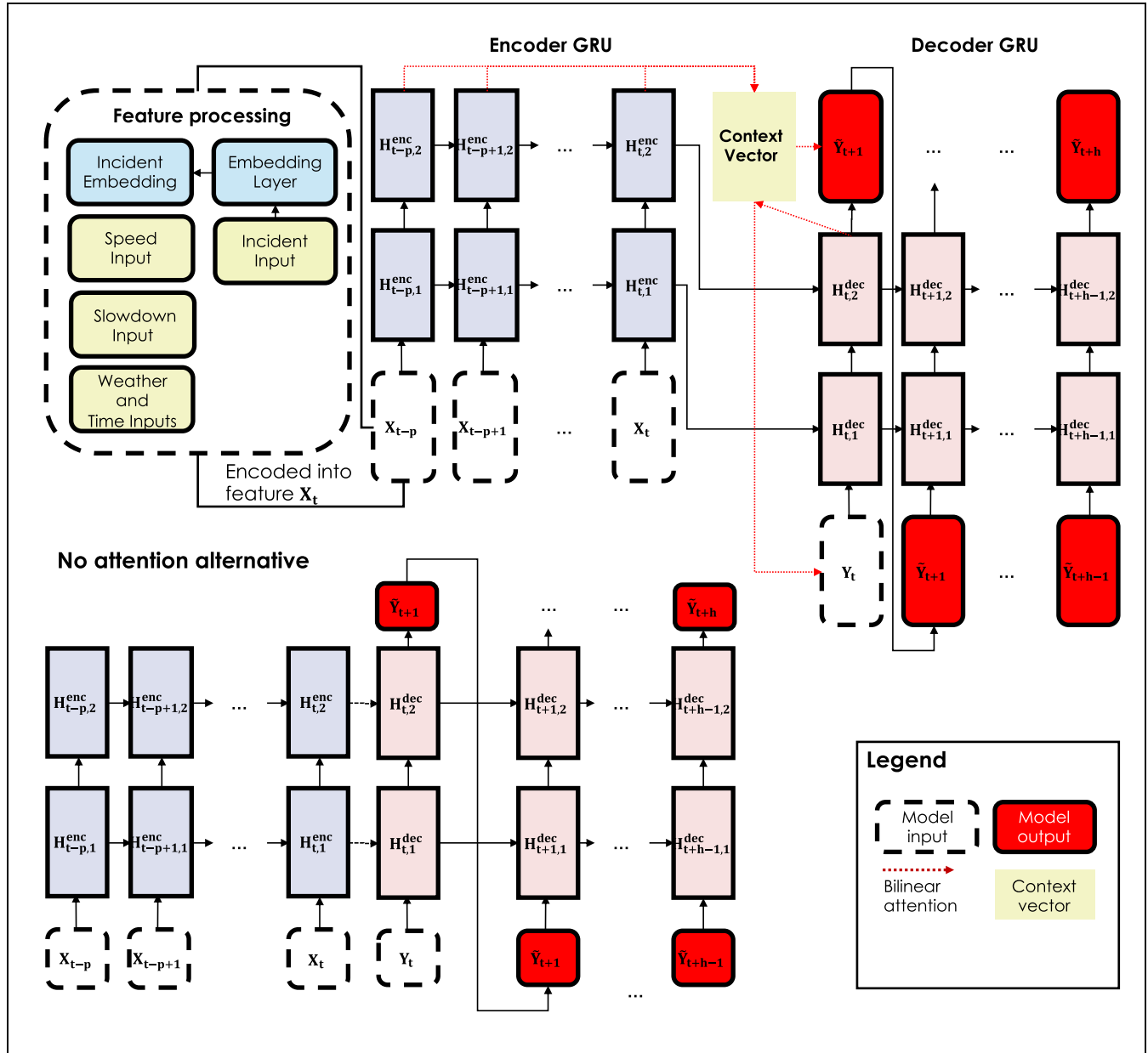
Figure 3. Traffic predictor architecture.
