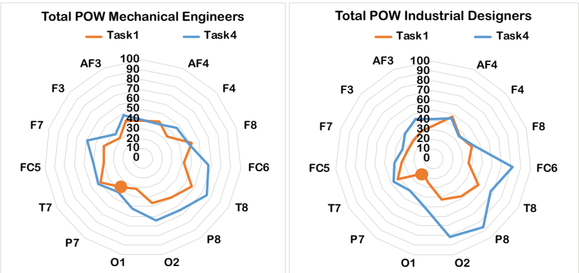
Figure 7. Transformed power (Pow) of the two tasks per domain. The solid circles indicate channels and task where there are significant differences across domains.
