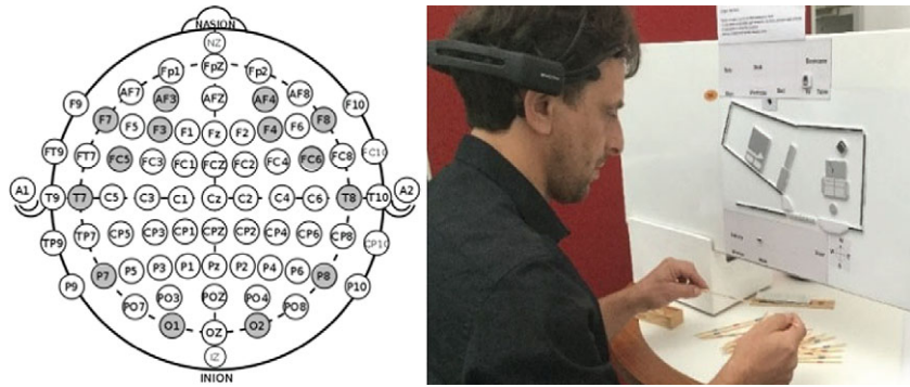
Figure 3. Emotiv Epoc+ electrodes highlighted in grey against the 10–10 I.S. layout and experiment setup using the headset.
