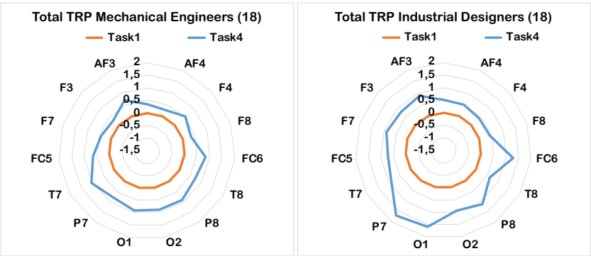
Figure 5. Radar plot of task-related power (TRP) for the 14 electrodes by taking the problem-solving Task 1 as the reference period for Task 4 for the industrial designers and mechanical engineers. The electrode labels are distributed such that all the electrodes on the left hemisphere are on the left and all those on the right hemisphere are on the right. Their labelling uses the standard 10–10 I.S.
