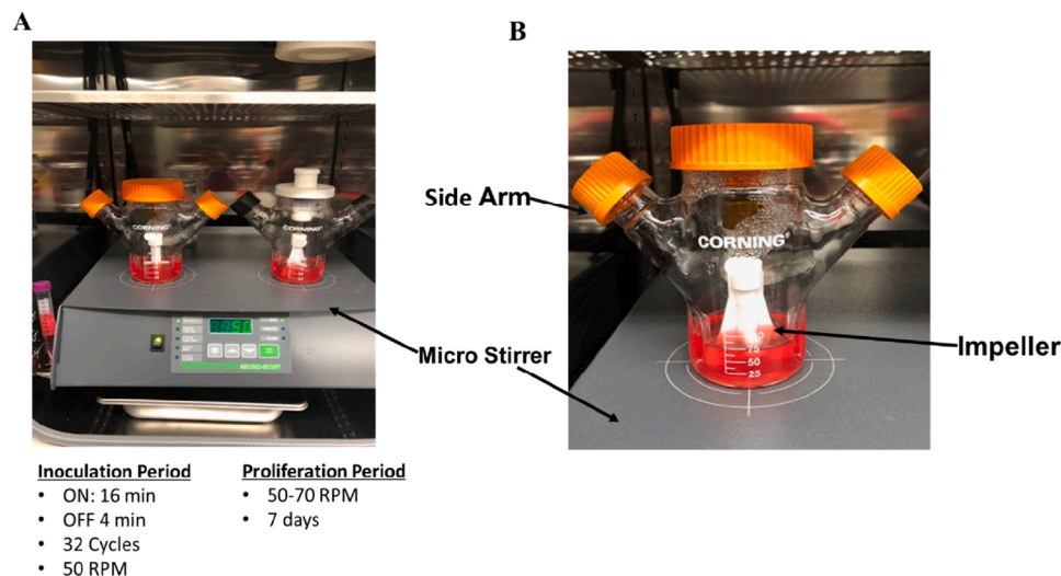
Fig. 1. Illustration of the microcarrier-based spinner flask platform for human mesenchymal stem cell (hMSC) expansion. (A) Spinner flask set-up on a programmable multi-position magnetic stirrer. (B) Zoom-in image of spinner flask and impeller. Intermittent agitation was used during inoculation period to maximize cell attachment to microcarriers. The spinner flasks were operated at 50-70 rpm.
