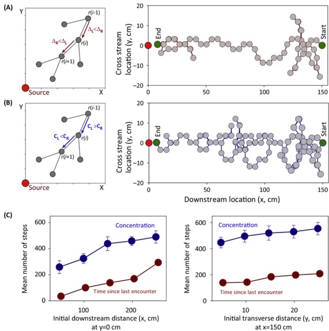
Figure 2 Computer Simulations of Search Strategies in A Simulated Odor Plume Using Time or Concentration with Paired Sensors. (A) Search strategy based on the ability of bursting olfactory receptor neurons (bORNs) to code time since the last odor stimulus encounter. The searcher or ‘animal’ compares the time since the last odor arrival detected by the left and right sensors and steers in the direction of the shorter interval. (B) Search strategy based on the ability of tonically active ORNs (tORNs) to code stimulus intensity. The searcher in this case compares the concentration detected by the left and right sensors and steers in the direction of the higher concentration. The left panel in each case illustrates the respective search strategy. The right panel in each case depicts the respective search trajectory from the downstream starting point (x = 150 cm, y = 0 cm) to the end (x = 0 cm, y = 0 cm) with decisions made at every dot. Searchers that exit the plume backtrack to their previous position. (C) Plots of the mean number of steps required to reach the source (left panel) or the midline (right panel) of the plume using concentration (blue) or time since last encounter (red). Note in both instances that using time is significantly faster than using concentration. Plotted are the mean and SE. Reproduced from [32].
