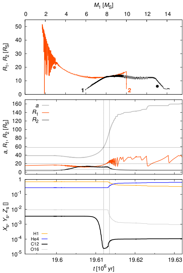
Fig. 19. Stellar evolution of a binary corresponding to \beta Lyr A. The component radii R_1 , R_2 vs. the primary mass M_1 are plotted (top), with observed values indicated by full circles, together with the distance a and R_1 , R_2 vs. time t (middle); see horizontal dashed lines, and surface abundances X , Y , A_{\text{C12}} , A_{\text{O16}} vs. time t (bottom). At t = 19.613 \times 10^6 yr, the mass ratio q corresponds to the observed one.
