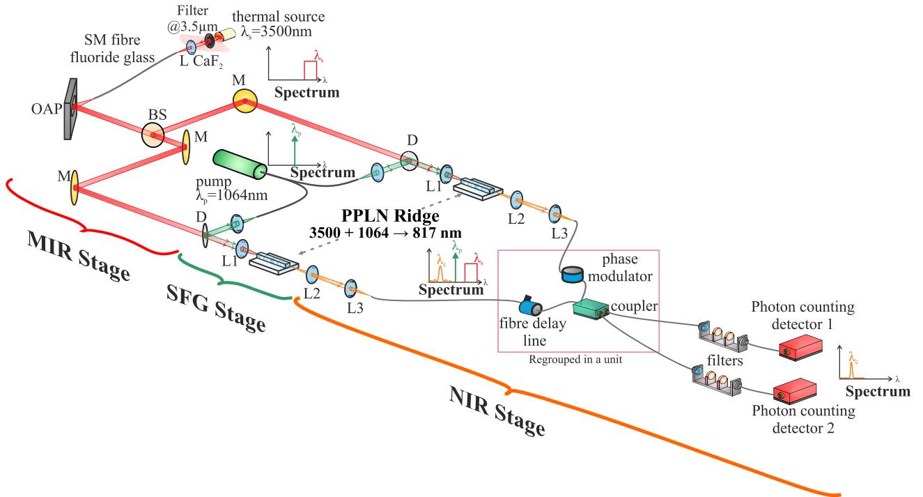
Figure 2. Diagram of the interferometric bench. L \text{CaF}_2 : \text{CaF}_2 lens. OAP: off-axis parabola. D: dichroic mirror (HR@1064 nm and AR@3.5 \mu\text{m} ). L1: off-axis parabola (a lens is shown for visibility reasons). L2, L3: microscope objectives. M: mirror. BS: beamsplitter.
