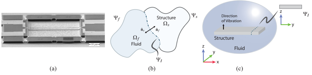
FIG. 1. (a) Scanning electron microscope image of a nanomechanical beam. Schematic of (b) a general fluid-structure interaction problem and (c) a beam immersed in a fluid.
