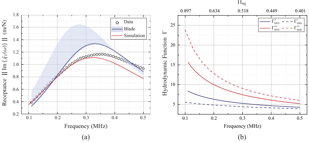
FIG. 6. Results for 60- \mu\text{m} NEMS beam in water. (a) Magnitude of the imaginary part of receptance ||\text{Im}\{\hat{\chi}_1(\omega)\}|| , versus frequency for data, blade approximation, and simulation. The shading indicates the uncertainty cloud of the cylinder model which was obtained by evaluating the receptance for the beam density range 2600 \text{ kg/m}^3 \leq \rho_s \leq 3400 \text{ kg/m}^3 . (b) Real, \Gamma'(\omega) , and imaginary, \Gamma''(\omega) , part of hydrodynamic function versus frequency (lower axis) and dimensionless squeeze number (upper axis), \Pi_{\text{sq}} , for blade approximation and simulation.
