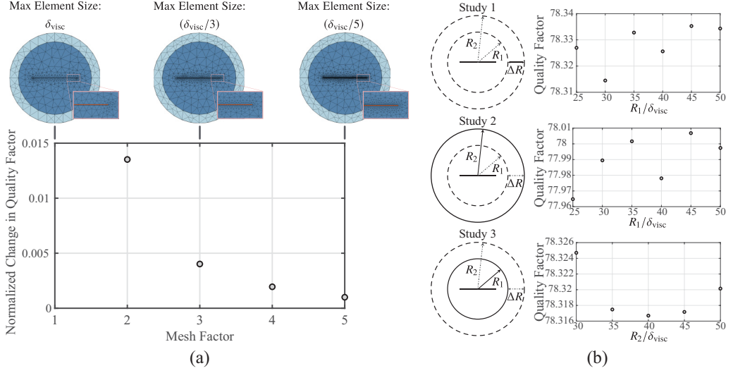
FIG. 13. (a) Normalized change in quality factor, (Q_j - Q_{j-1})/Q_{j-1} , versus mesh factor found from mesh refinement study. (b) Results from Studies 1–3 of convergence study that analyzed FEM's dependence on fluid domain size. Results plot computed quality factor, Q , versus normalized radius length.
