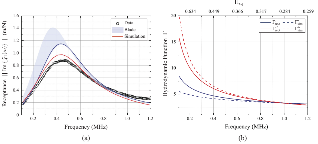
FIG. 5. Results for 50- \mu\text{m} NEMS beam in water. (a) Magnitude of the imaginary part of receptance \|\text{Im}\{\chi(\omega)\}\| , versus frequency for data, blade approximation, and simulation. The shading indicates the uncertainty cloud of the cylinder model which was obtained by evaluating the receptance for the beam density range 2600 \text{ kg/m}^3 \leq \rho_s \leq 3400 \text{ kg/m}^3 . (b) Real, \Gamma'(\omega) , and imaginary, \Gamma''(\omega) , part of hydrodynamic function versus frequency (lower axis) and dimensionless squeeze number (upper axis), \Pi_{sq} , for blade approximation and simulation.
