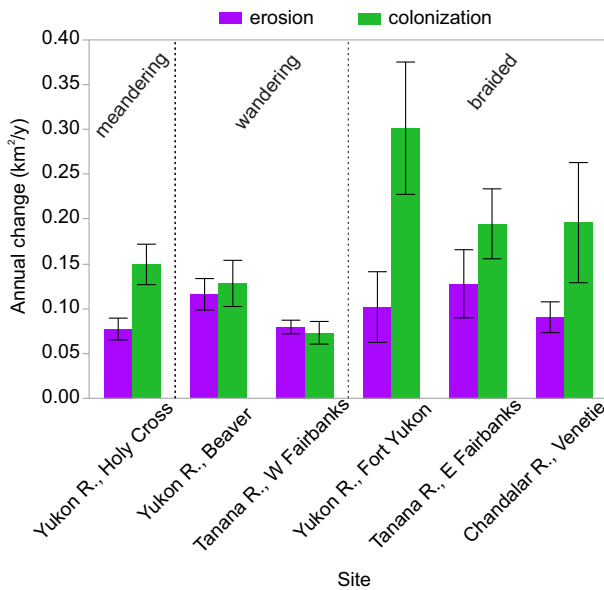
Fig. 5 Mean riverbank erosion rates and vegetation colonization rates by site. Error bars represent the 95% confidence interval
