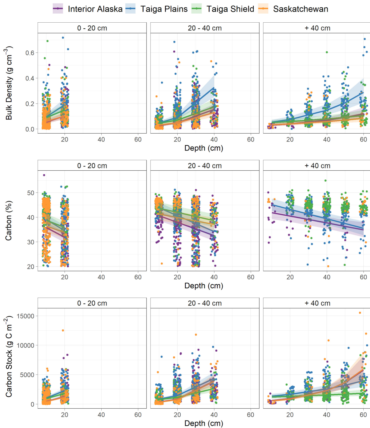
FIGURE 4 | Soil properties of bulk density ( \text{g cm}^{-3} ), carbon content (%) and carbon pool ( \text{g C m}^{-2} ) as a function of sample depth, total plot SOL thickness, and ecoregion. Lines represent significant ecoregion specific relationships between soil properties and depth in the soil profile and shading represents 95% confidence intervals. Note that points are jittered horizontally at each 10 cm depth increment (width = 2 cm). See Supplementary Table S4 for model results and Table 3 for Tukey-Kramer post-hoc pairwise comparisons of marginal mean intercepts and slopes compared across total SOL thickness categories within ecoregions and across ecoregions within total SOL thickness categories.
