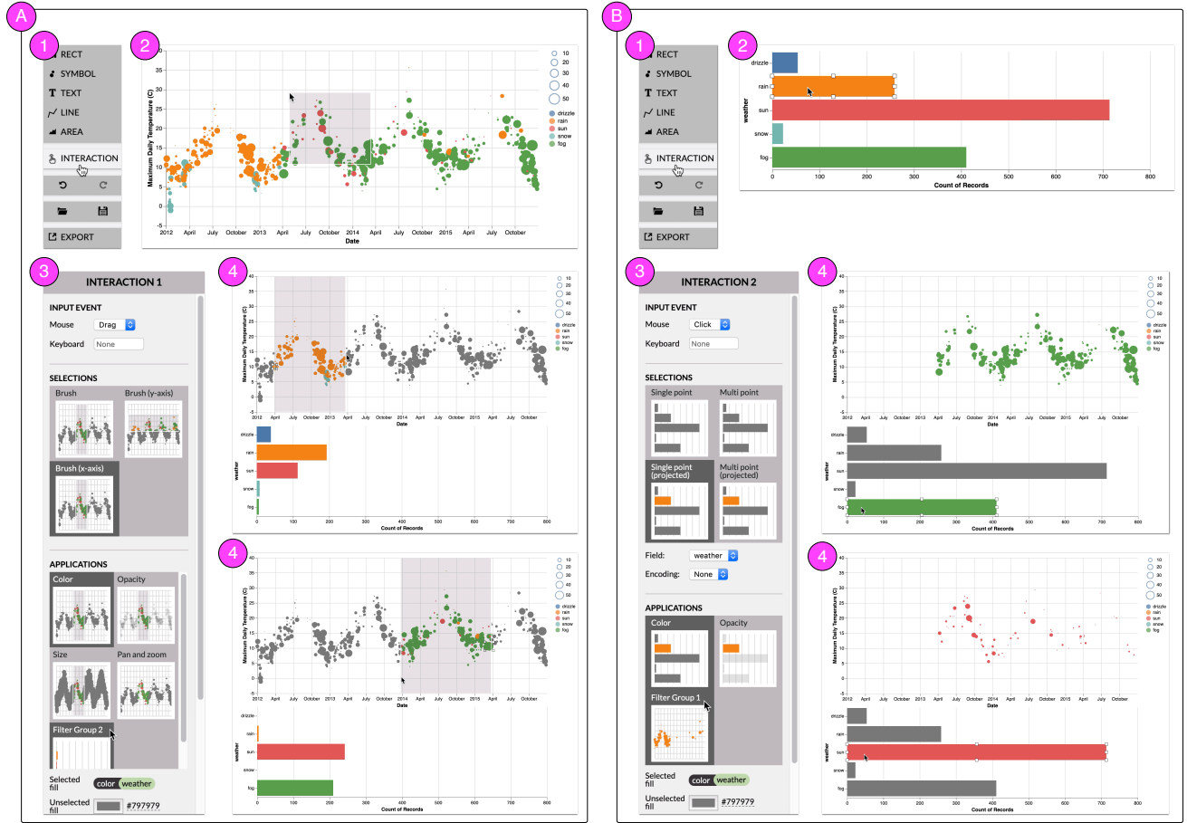
Fig. 2. The process of creating the interactive visualization in Fig. 1. (a) Demonstrating a horizontal brush that colors selected points in the scatterplot and re-aggregates the histogram. (b) Demonstrating a click interaction that colors the selected bar and filters the scatterplot via the weather field.
