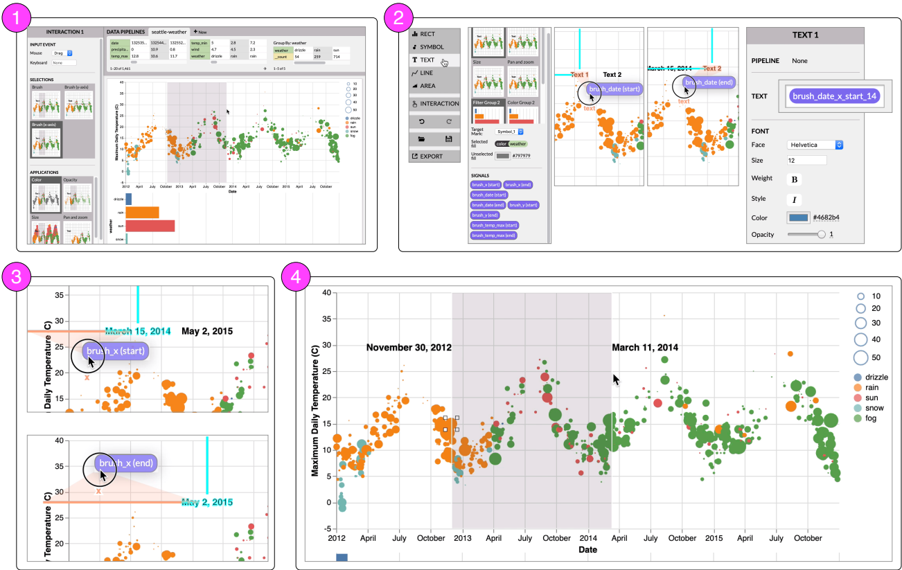
Fig. 3. Brush with labeled extents. (1) A brushing interaction authored via demonstrations (see Fig. 2) (2) Binding signals that represent the brush's start and end extents to the content of two text marks respectively. (3) Positioning the text marks by their horizontal position to the brush's start and end x-coordinates. (4) The completed design: an interval selection with labeled extents.
