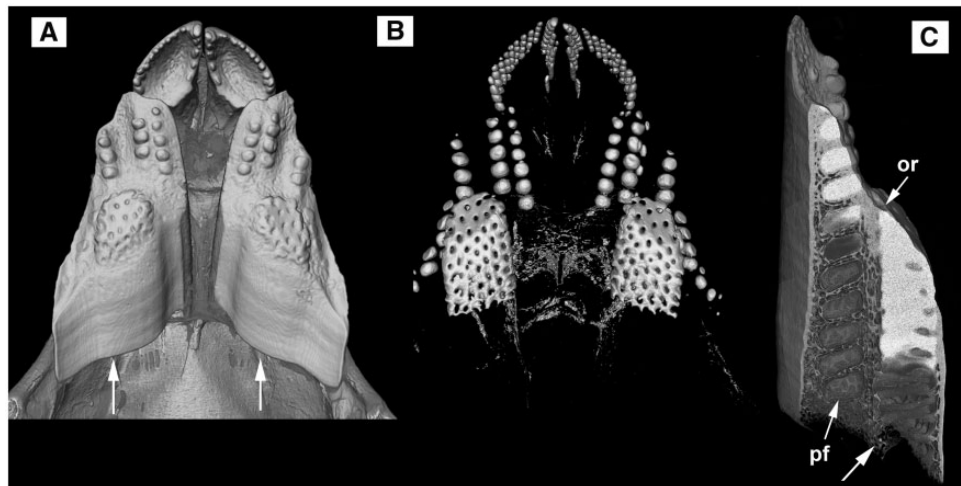
Fig. 4 Harriotta raleighana (Chimaeridae; Chimaeroidei; Holocephali), upper dentition, micro-CT scan. A) Skull and anterior and posterior upper jaw dental plate. B) Rendered scan to show mineralized dentine structures, including columns of ovoids and tritons. C) Virtual section through lower jaw dental plate showing mineralized ovoids and tritons, and surrounding trabecular dentine of lower mineral density. Tissue growth occurs at the aboral surface (opposite to the oral surface, or), including organized, preformed spaces within the trabecular dentine for ovoids and tritons. From Smith et al. (2019, figs. 2D and 16G and H).
