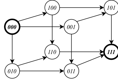
Figure 4: Bellman-Held-Karp computation graph with 3 cities. The graph is a 3 dimensional boolean hypercube, with starting point 000 and ending point 111.
