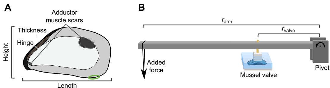
Fig. 1. Mussel morphology and experimental set-up. (A) Internal structures of a right valve of a California mussel. Length, height and hinge thickness were measured as the maximum extent along the defined axes. Width was measured as the widest extent perpendicular to height and length. The green oval indicates the approximate location of the hook used when measuring maximum closing force. The valve is oriented with anterior to the left and dorsal above. (B) During static fatigue testing, a force was applied to a mussel valve in a saltwater bath by adding a force at the end of a lever arm. The force applied to the shell was calculated according to Eqn 1, with r_{\text{valve}} and r_{\text{arm}} defined as the length of the radius arm from the pivot to the valve and to the applied force, respectively. This apparatus was adapted to test the constant opening force generated by the mussel hinge. Not to scale; the lever arm was proportionally longer and the mussel smaller than portrayed here.
