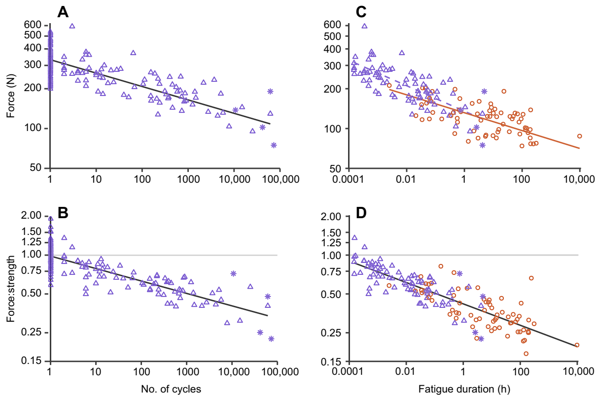
Fig. 4. Valves of mussel shells fatigue under cyclic and static loading. (A,B) The force required to break a valve decreased as a valve was loaded repeatedly. This was true for absolute force (A) and force relative to predicted strength (B). Multiple regressions are shown at average values for all morphological variables (Table 2). The light gray line in B represents a loading force equal to the predicted one-time strength. Purple asterisks indicate that a valve never broke and therefore represent a lower bound of the true number of cycles until breakage. These points were not included in the regression. N=156 complete, N=4 incomplete tests of individual valves. (C,D) Valves that were loaded cyclically (purple triangles) and statically (red circles) both experienced fatigue, whether considering absolute force (C) or force divided by predicted strength (D). Multiple regressions are shown at average values for all morphological variables (Table 2). Regressions for cyclic (purple dashed line) and static (red solid line) loading differed significantly when considering absolute force (C), but they did not differ when accounting for predicted strength (D) (Table 2). The light gray line in D represents a loading force equal to the predicted strength. Purple asterisks indicate that a valve never broke under cyclic loading and therefore represent a lower bound of the true time until breakage. These points were not included in the regression. Cyclic fatigue: N=77 complete, N=4 incomplete tests of individual valves; static fatigue: N=68 complete tests of individual valves.
