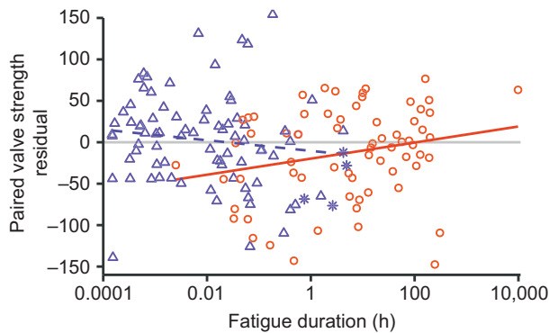
Fig. 5. Strength of counterparts of cyclically and statically loaded valves. Taking advantage of a shell's two-valve morphology, the partner valve of each fatigue-tested valve was strength tested to provide general information about the shell. In the static fatigue treatment (red circles, solid line), valves that broke after shorter durations also tended to have counterparts that were uncharacteristically weak for their size ( P < 0.05 ); for cyclically fatigued shells (purple triangles, dashed line), no such relationship existed [ P = 0.26 ; full model: F_{3,141} = 2.7 , P < 0.05 , R^2 = 0.05 ; model for cyclic loading: (strength residual) = 12.4 - 6.4 \times \log_{10}(\text{fatigue duration}) ; model for static loading: (strength residual) = -54.2 + 9.7 \times \log_{10}(\text{fatigue duration}) ]. Deviation from expected strength based on morphology was quantified as the valve's residual (actual–predicted strength) calculated from the strength model in Table 2. The light gray line represents a residual of 0, with negative y-values indicating uncharacteristically weak valves, and positive y-values indicating uncharacteristically strong valves. Purple asterisks indicate that the fatigue-tested valve never broke and therefore represent a lower bound of the true duration until breakage. These points were not included in the regression. Cyclic fatigue: N = 77 complete, N = 4 incomplete tests of individual valves; static fatigue: N = 68 complete tests of individual valves.
