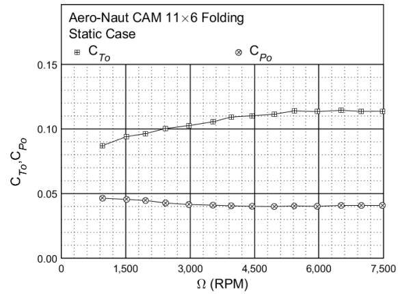
Figure 28: Static performance of the Aero-Naut CAM 11×6 folding propeller: thrust and power coefficient.
