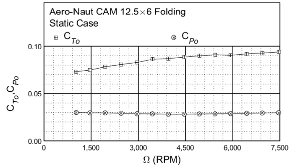
Figure 54: Static performance of the Aero-Naut CAM 12.5×6 folding propeller: thrust and power coefficient.
