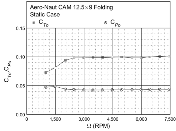
Figure 58: Static performance of the Aero-Naut CAM 12.5×9 folding propeller: thrust and power coefficient.
