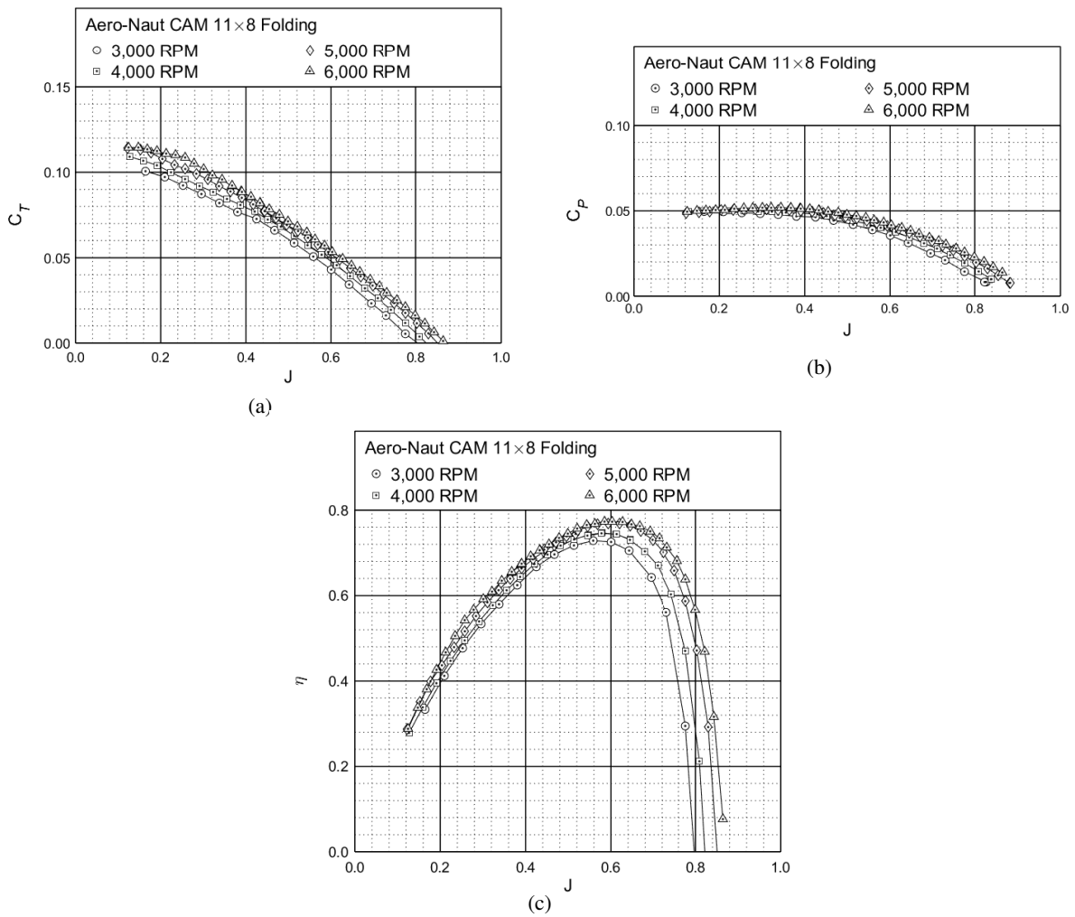
Figure 31: Performance of the Aero-Naut CAM 11×8 folding propeller: (a) thrust coefficient, (b) power coefficient, (c) efficiency.
