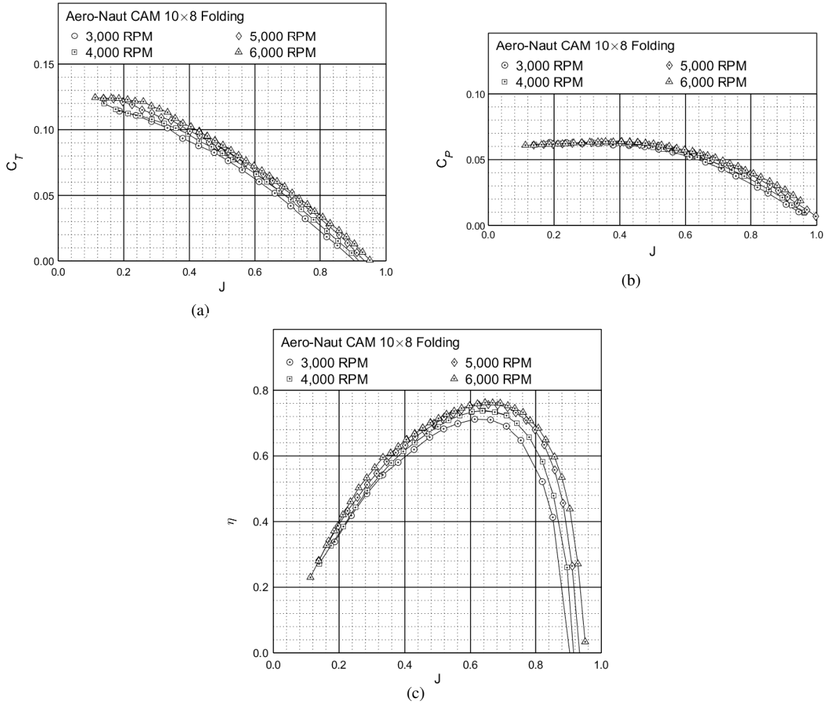
Figure 21: Performance of the Aero-Naut CAM 10×8 folding propeller: (a) thrust coefficient, (b) power coefficient, (c) efficiency.
