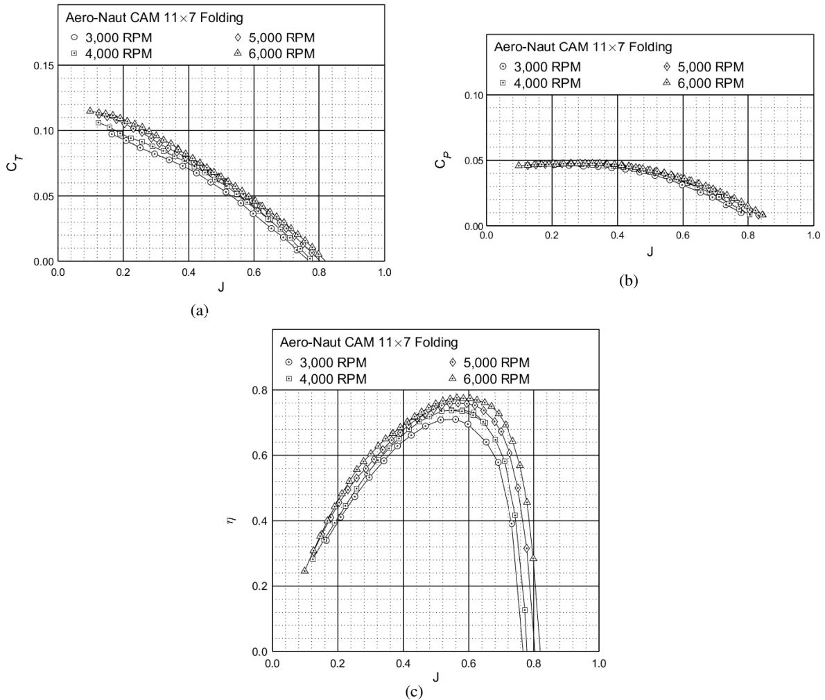
Figure 29: Performance of the Aero-Naut CAM 11×7 folding propeller: (a) thrust coefficient, (b) power coefficient, (c) efficiency.
