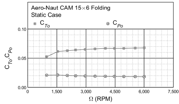
Figure 78: Static performance of the Aero-Naut CAM 15×6 folding propeller: thrust and power coefficient.
