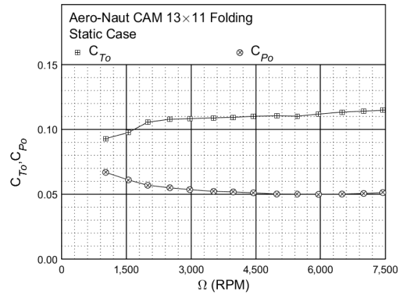
Figure 68: Static performance of the Aero-Naut CAM 13×11 folding propeller: thrust and power coefficient.
