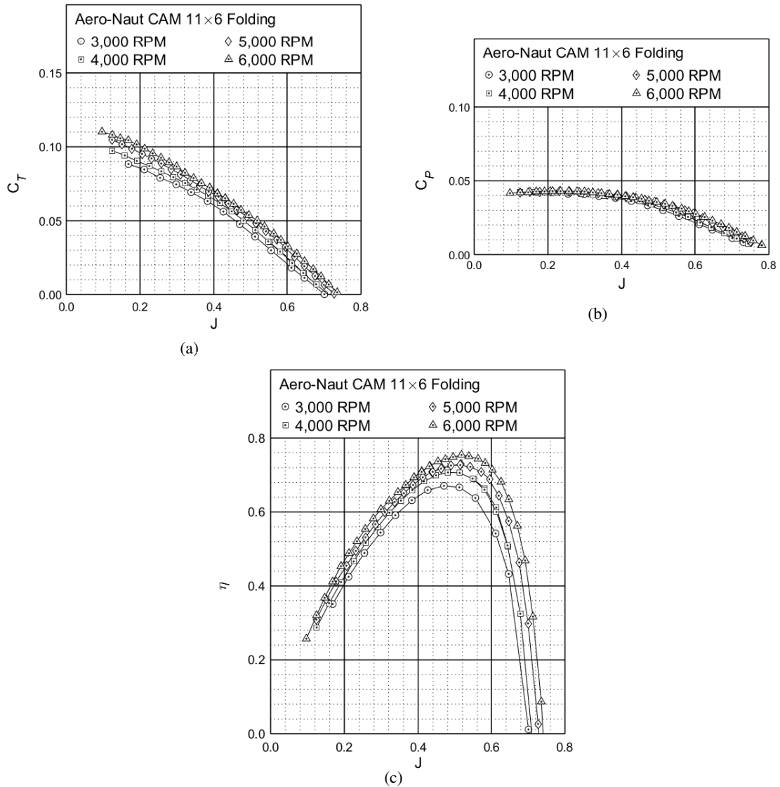
Figure 27: Performance of the Aero-Naut CAM 11×6 folding propeller: (a) thrust coefficient, (b) power coefficient, (c) efficiency.
