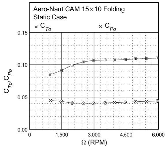
Figure 82: Static performance of the Aero-Naut CAM 15x10 folding propeller: thrust and power coefficient.
