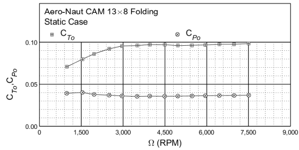
Figure 64: Static performance of the Aero-Naut CAM 13×8 folding propeller: thrust and power coefficient.
