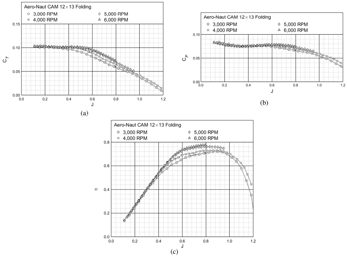
Figure 51: Performance of the Aero-Naut CAM 12×13 folding propeller: (a) thrust coefficient, (b) power coefficient, (c) efficiency.
