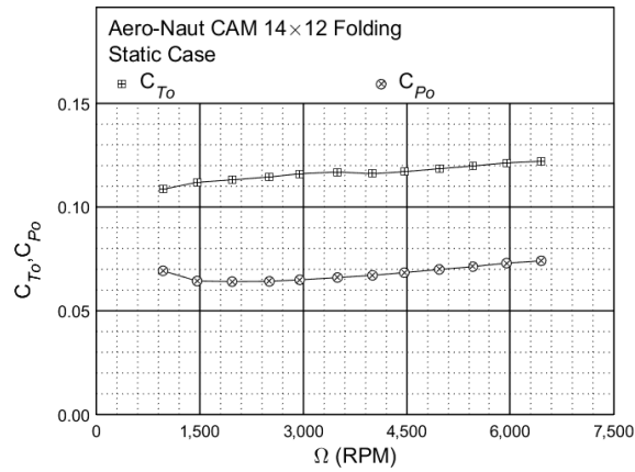
Figure 76: Static performance of the Aero-Naut CAM 14×12 folding propeller: thrust and power coefficient.
