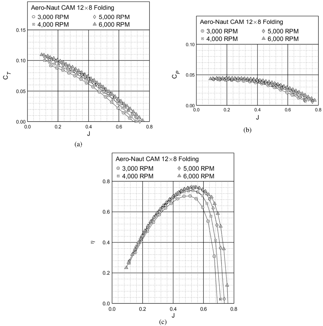
Figure 43: Performance of the Aero-Naut CAM 12×8 folding propeller: (a) thrust coefficient, (b) power coefficient, (c) efficiency.
