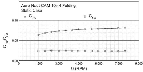
Figure 14: Static performance of the Aero-Naut CAM 10×4 folding propeller: thrust and power coefficient.
