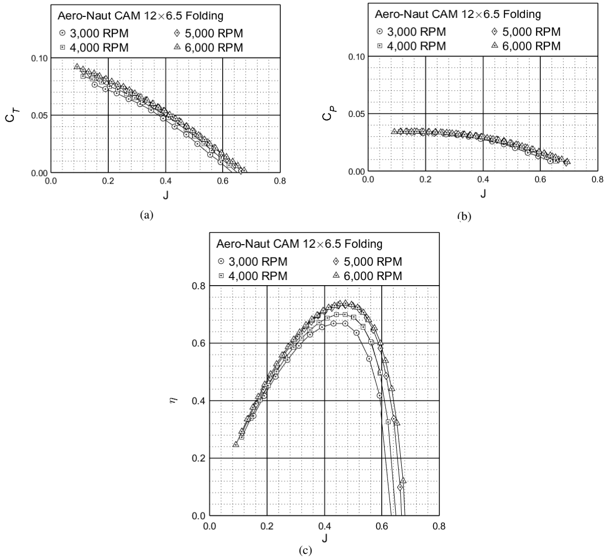
Figure 41: Performance of the Aero-Naut CAM 12×6.5 folding propeller: (a) thrust coefficient, (b) power coefficient, (c) efficiency.
