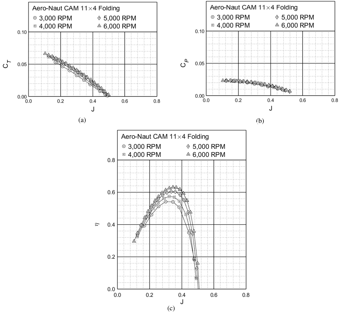
Figure 25: Performance of the Aero-Naut CAM 11×4 folding propeller: (a) thrust coefficient, (b) power coefficient, (c) efficiency.
