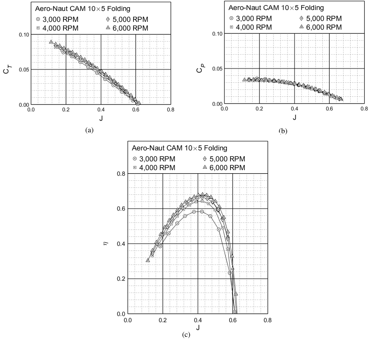
Figure 15: Performance of the Aero-Naut CAM 10×5 folding propeller: (a) thrust coefficient, (b) power coefficient, (c) efficiency.
