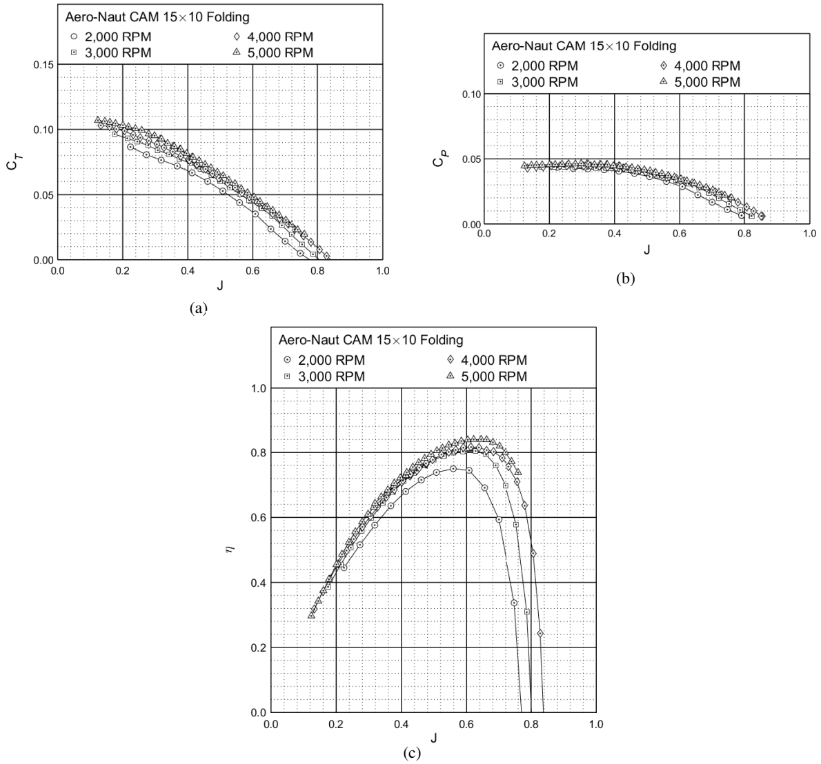
Figure 81: Performance of the Aero-Naut CAM 15x10 folding propeller: (a) thrust coefficient, (b) power coefficient, (c) efficiency.
