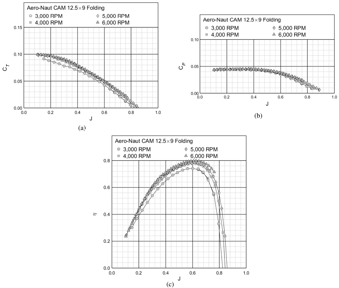
Figure 57: Performance of the Aero-Naut CAM 12.5×9 folding propeller: (a) thrust coefficient, (b) power coefficient, (c) efficiency.
