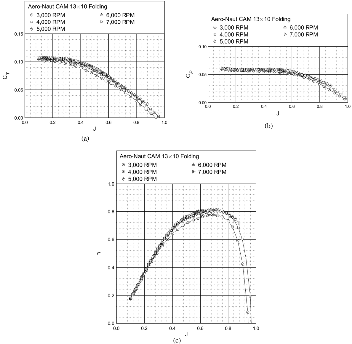
Figure 65: Performance of the Aero-Naut CAM 13×10 folding propeller: (a) thrust coefficient, (b) power coefficient, (c) efficiency.
