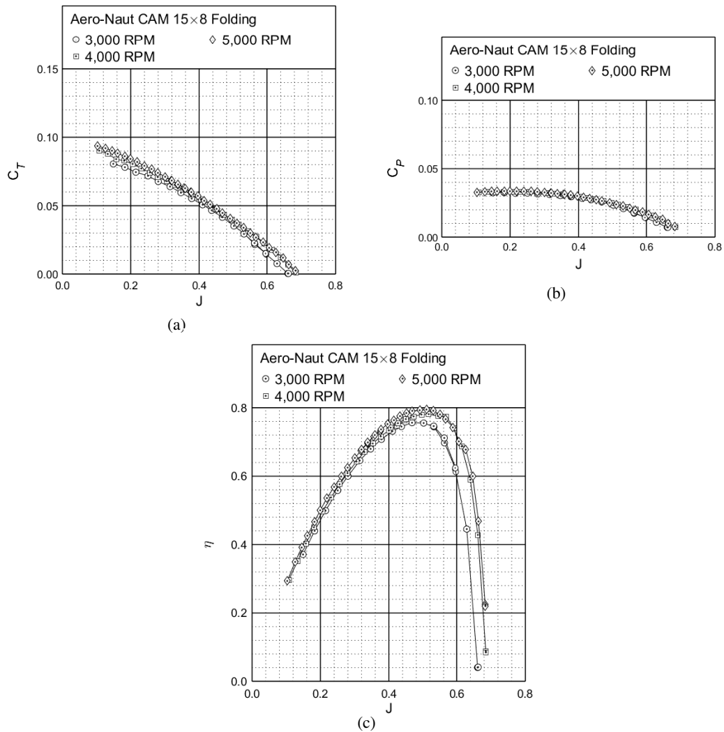
Figure 79: Performance of the Aero-Naut CAM 15×8 folding propeller: (a) thrust coefficient, (b) power coefficient, (c) efficiency.
