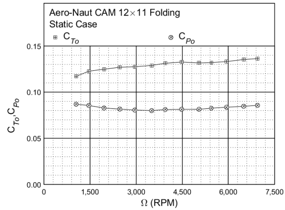
Figure 50: Static performance of the Aero-Naut CAM 12×11 folding propeller: thrust and power coefficient.
