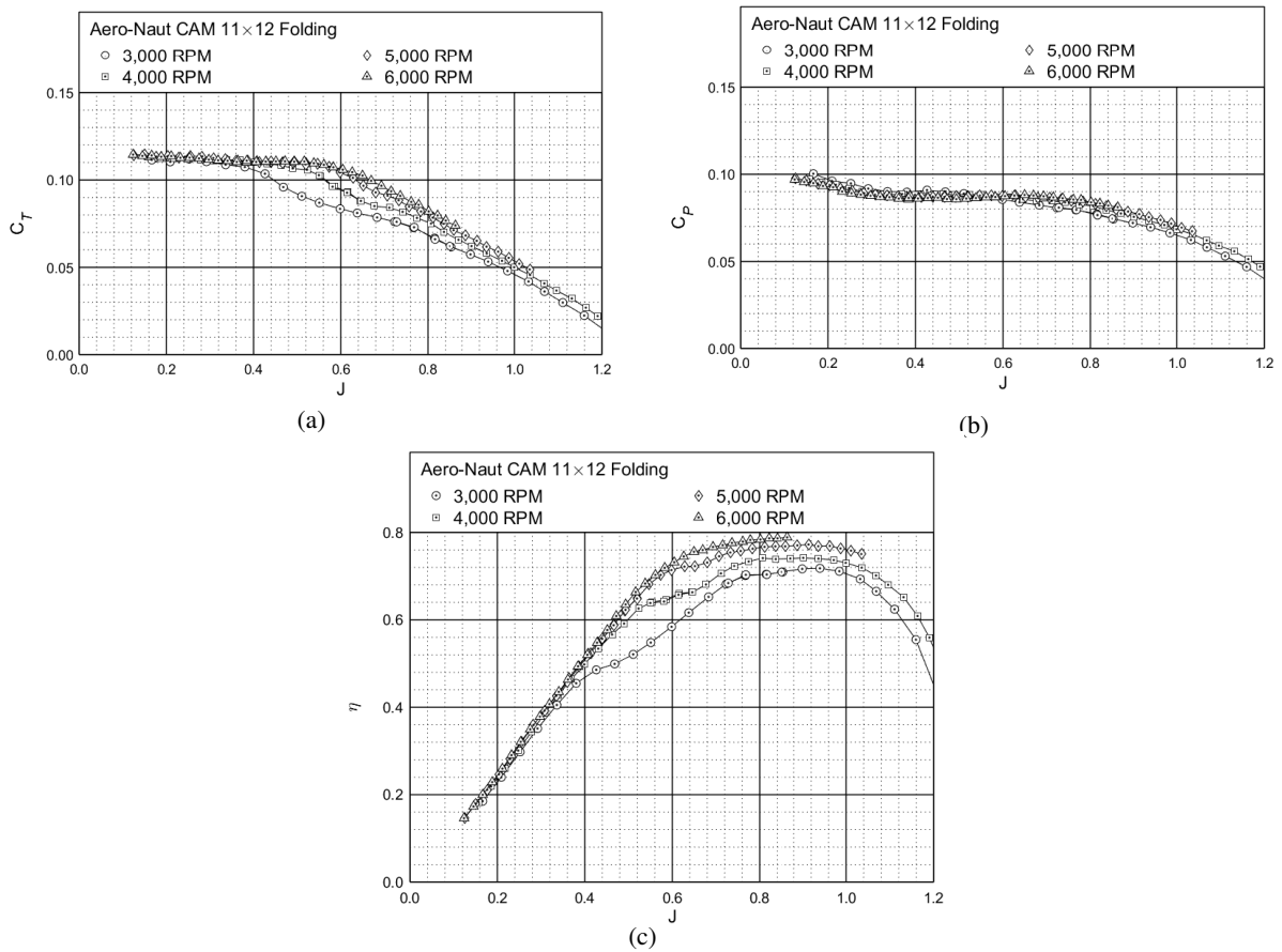
Figure 35: Performance of the Aero-Naut CAM 11×12 folding propeller: (a) thrust coefficient, (b) power coefficient, (c) efficiency.
