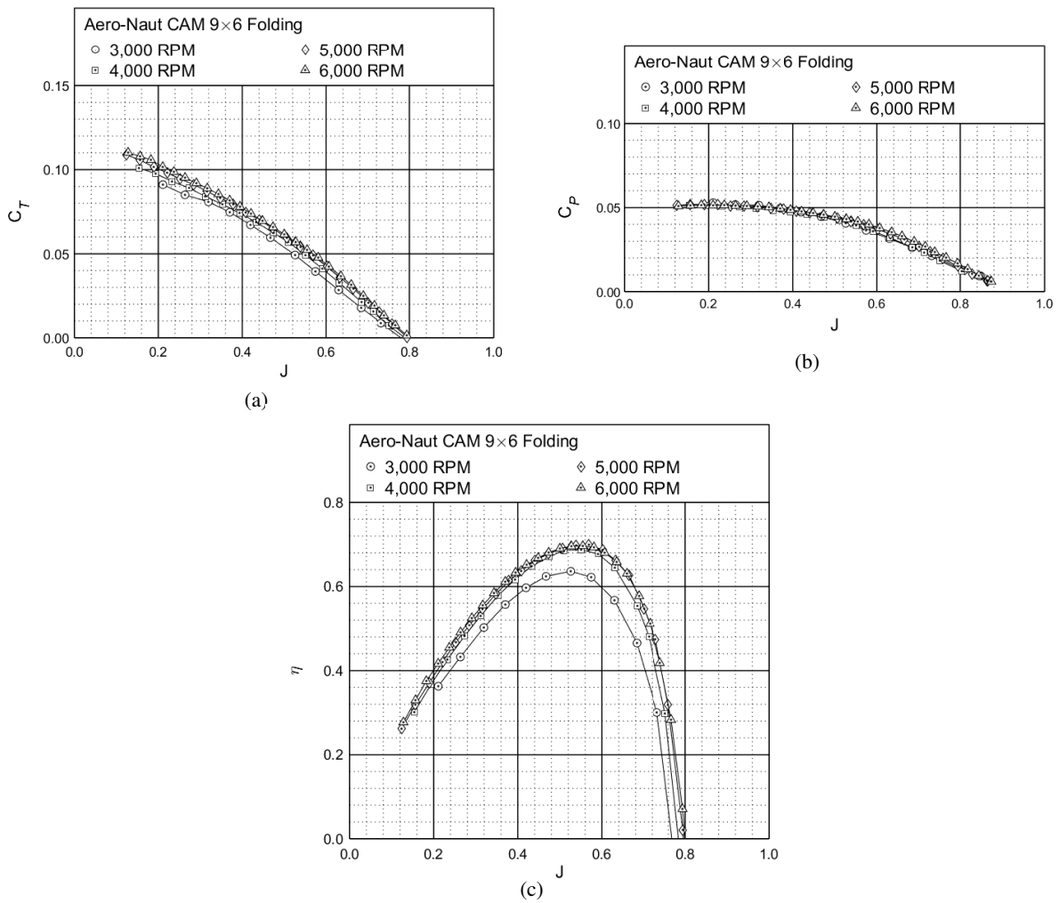
Figure 9: Performance of the Aero-Naut CAM 9×6 folding propeller: (a) thrust coefficient, (b) power coefficient, (c) efficiency.
