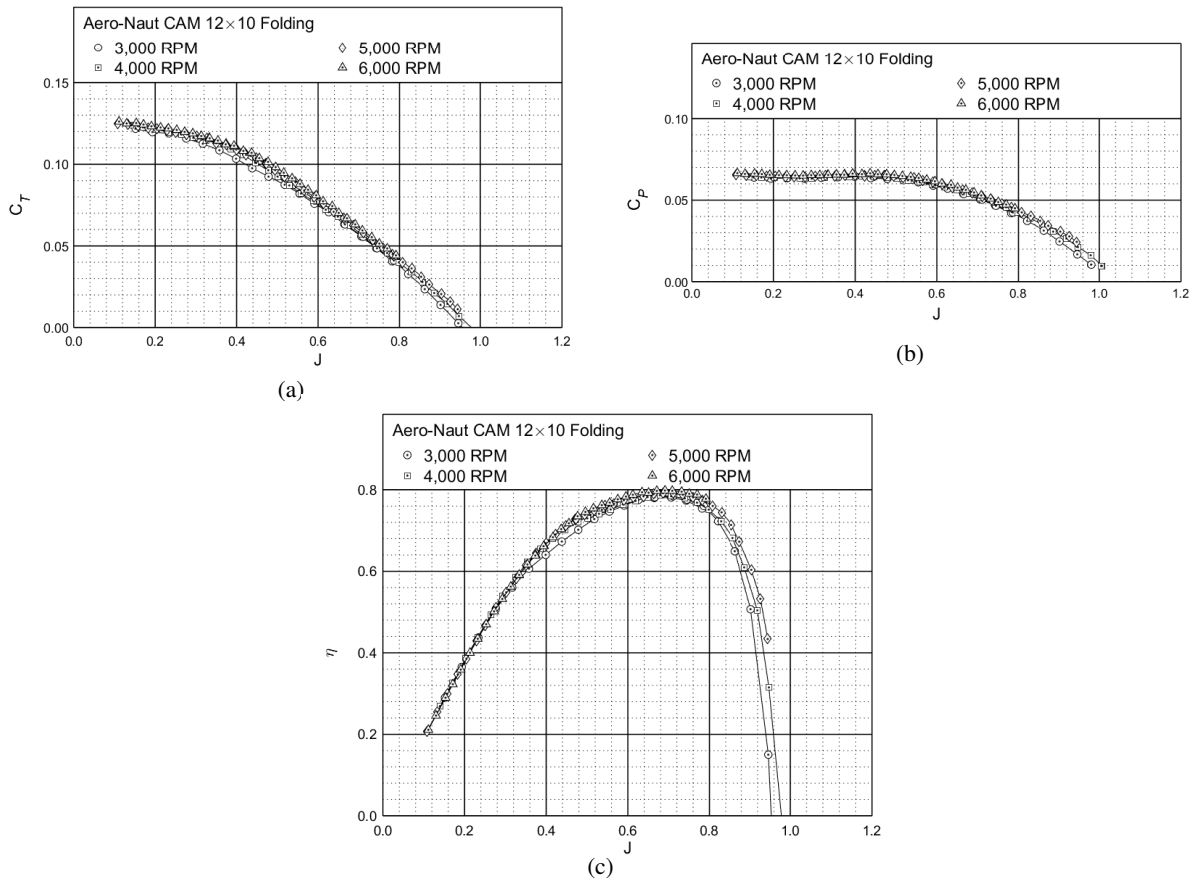
Figure 47: Performance of the Aero-Naut CAM 12x10 folding propeller: (a) thrust coefficient, (b) power coefficient, (c) efficiency.
