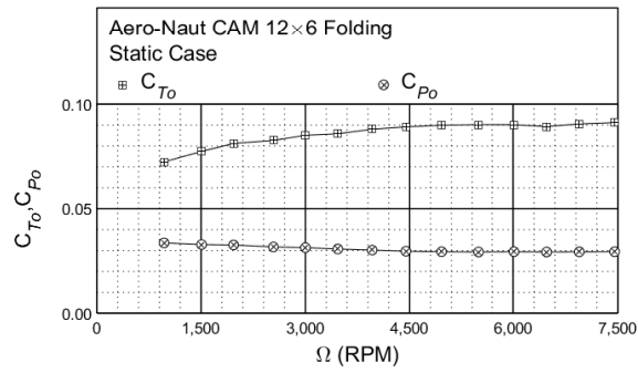
Figure 40: Static performance of the Aero-Naut CAM 12×6 folding propeller: thrust and power coefficient.
