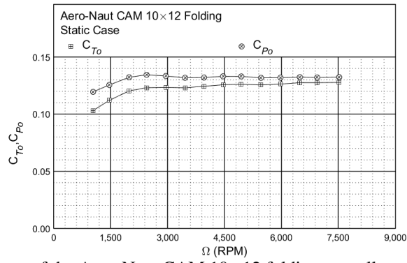
Figure 24: Static performance of the Aero-Naut CAM 10×12 folding propeller: thrust and power coefficient.
