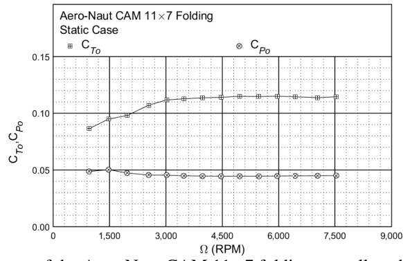
Figure 30: Static performance of the Aero-Naut CAM 11×7 folding propeller: thrust and power coefficient.
