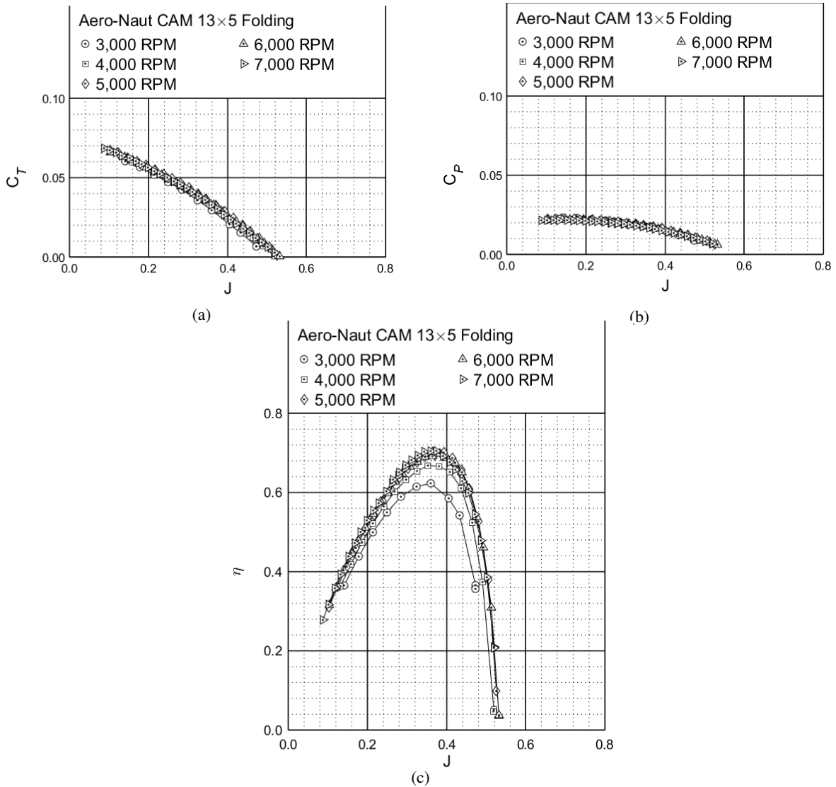
Figure 59: Performance of the Aero-Naut CAM 13×5 folding propeller: (a) thrust coefficient, (b) power coefficient, (c) efficiency.
