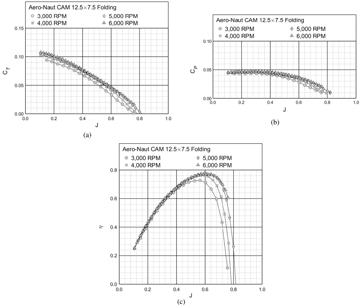
Figure 55: Performance of the Aero-Naut CAM 12.5×7.5 folding propeller: (a) thrust coefficient, (b) power coefficient, (c) efficiency.
