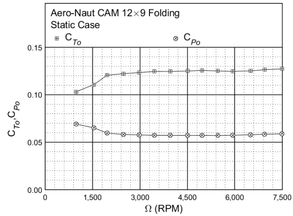
Figure 46: Static performance of the Aero-Naut CAM 12x9 folding propeller: thrust and power coefficient.
