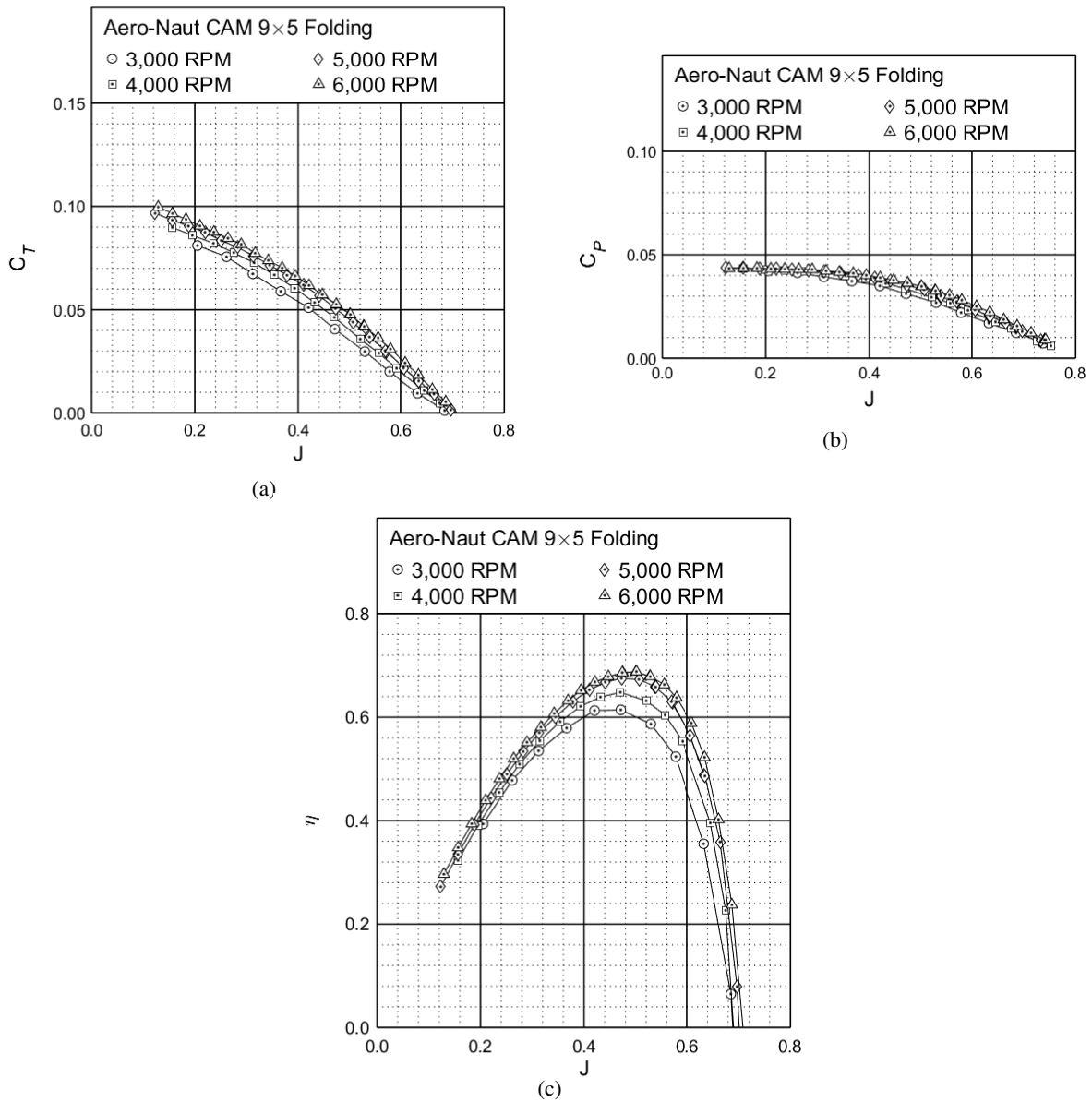
Figure 7: Performance of the Aero-Naut CAM 9×5 folding propeller: (a) thrust coefficient, (b) power coefficient, (c) efficiency.
