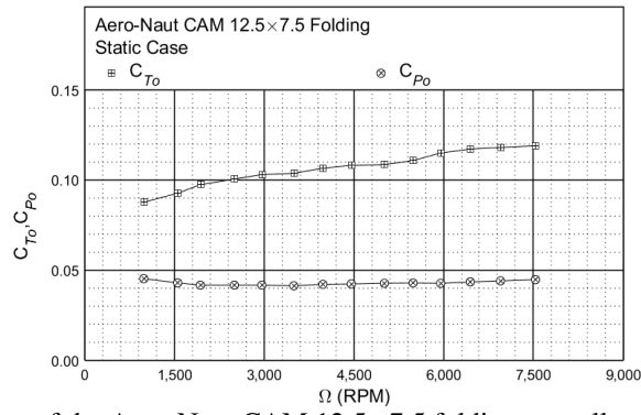
Figure 56: Static performance of the Aero-Naut CAM 12.5×7.5 folding propeller: thrust and power coefficient.
