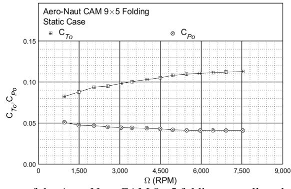
Figure 8: Static performance of the Aero-Naut CAM 9×5 folding propeller: thrust and power coefficient.
