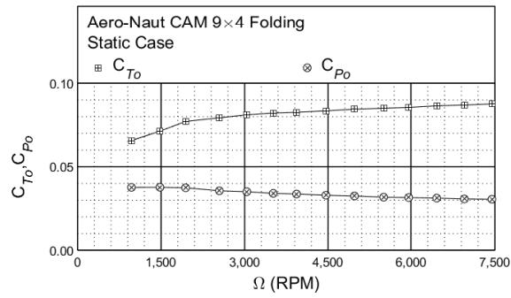
Figure 6: Static performance of the Aero-Naut CAM 9×4 folding propeller: thrust and power coefficient.
