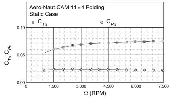
Figure 26: Static performance of the Aero-Naut CAM 11×4 folding propeller: thrust and power coefficient.
