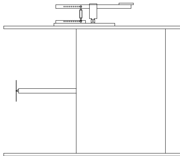
Figure 4: Propeller balance enclosed in fairing.
