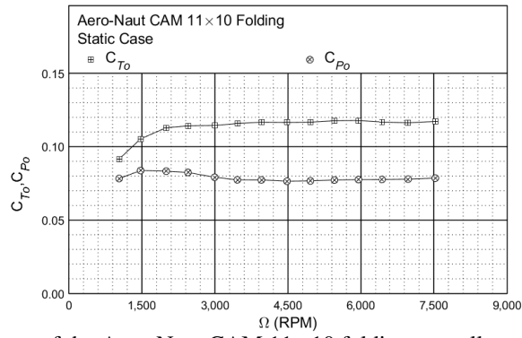
Figure 34: Static performance of the Aero-Naut CAM 11×10 folding propeller: thrust and power coefficient.
