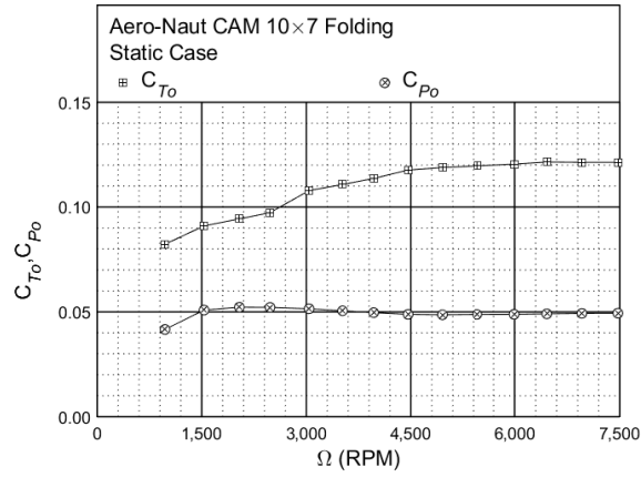
Figure 20: Static performance of the Aero-Naut CAM 10×7 folding propeller: thrust and power coefficient.
