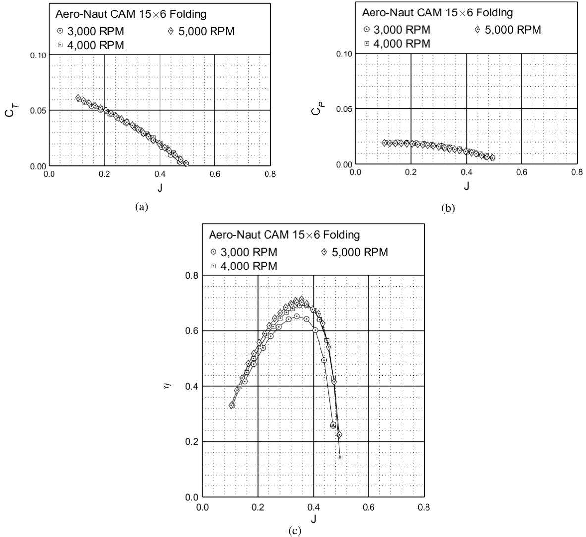
Figure 77: Performance of the Aero-Naut CAM 15×6 folding propeller: (a) thrust coefficient, (b) power coefficient, (c) efficiency.
