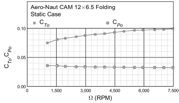
Figure 42: Static performance of the Aero-Naut CAM 12×6.5 folding propeller: thrust and power coefficient.
