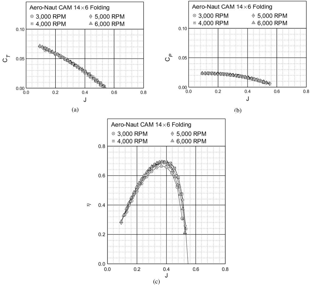
Figure 69: Performance of the Aero-Naut CAM 14×6 folding propeller: (a) thrust coefficient, (b) power coefficient, (c) efficiency.
