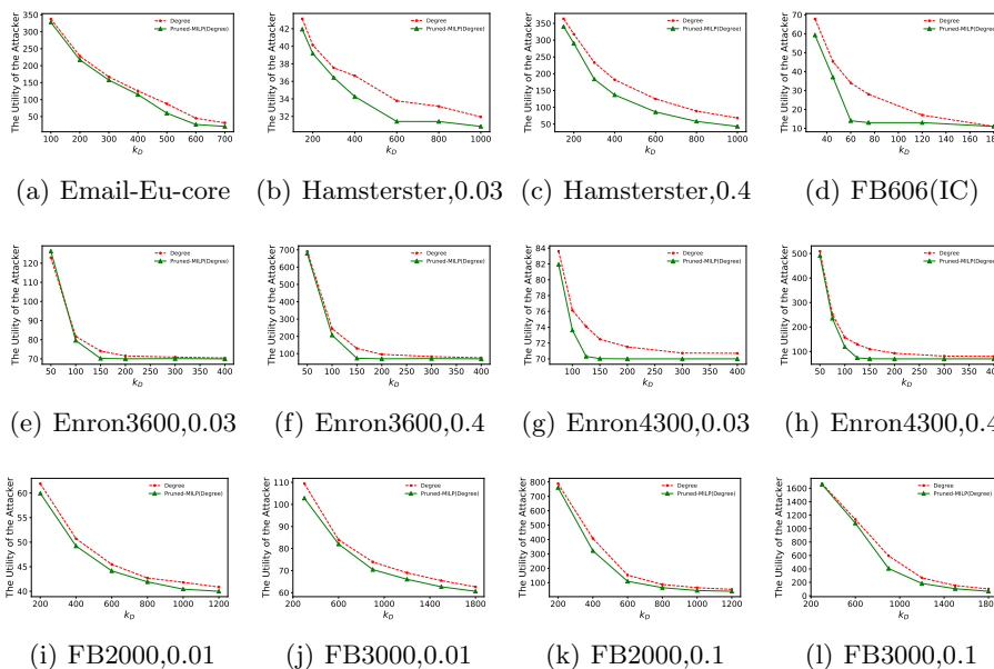
Fig. 4. The performance of PRUNED-MILP on real-world networks against IM attackers.
