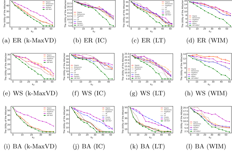
Fig. 2. The performance of DEF-MILP on synthetic networks against several attacks.
