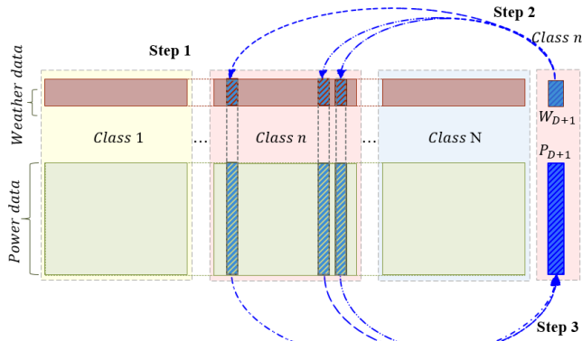
FIGURE 2. Structure of the proposed cSBFM.
