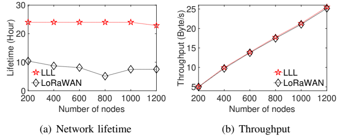
Fig. 5. Network lifetime and throughput under varying number of nodes
