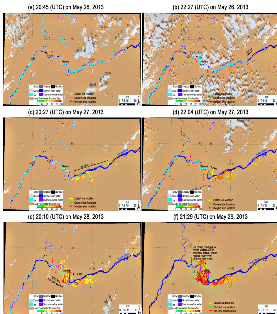
Figure 4. The flood detection maps at 20:45 UTC (a) and 22:27 UTC (b) on May 26; and at 20:27 UTC (c) and 22:04 UTC (d) on May 27, 20:10 UTC on May 28 (e) and 21:29 UTC on May 29 (f), 2013. Yellow arrow displays the latest ice location, green arrow indicates current ice location, and red arrow marks the ice jam location.
