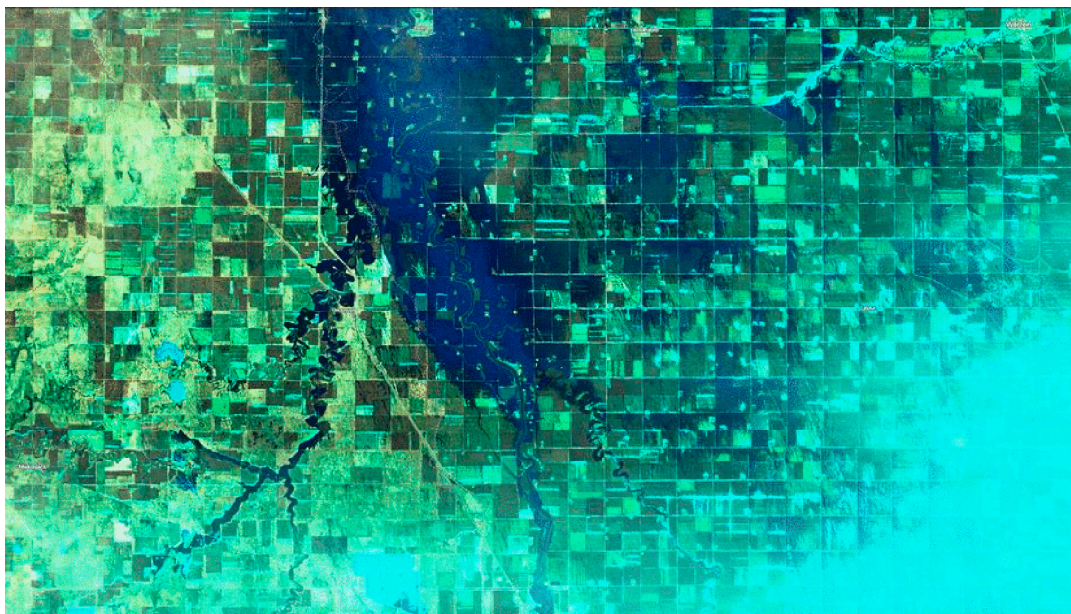
Figure 7. Sentinel-2 Short wave infrared composite (SWIR) imagery on 10 April 2020.
