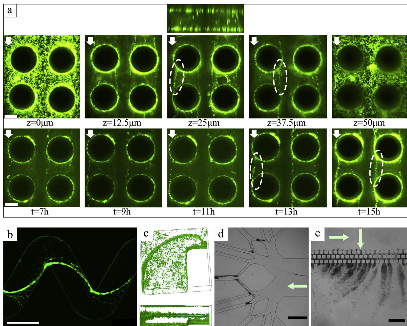
Fig. 10. Laminar flow streamers. (a) Streamer formation in a porous microfluidic device. First row: confocal images of streamers at five different z -locations of the channel, Z = 0 , Z = 12.5 , Z = 25 , Z = 37.5 , Z = 50\mu\text{m} after 15 h of experiment. Confocal sidebar view shown on top. Second row: time evolution of streamers at the flow rate of 8\text{ml h}^{-1} . White arrows show the direction of the flow, and the scale bar represents 20\mu\text{m} . Dashed outlines highlight some of the streamers. Adapted from [157,179]. (b) Confocal microscopy image of streamers formed in a zig-zag channel, scale bar represents 250\mu\text{m} . (c) Three-dimensional view of channel and of its cross-section with streamer forming at bend. (d) Streamer fouling of a branched network with green arrow indicating flow direction, scale bar represents 500\mu\text{m} . (e) Streamer fouling of a staggered-channel filtration device where green arrows indicate pseudo-cross-flow direction, scale bar represents 500\mu\text{m} [167]. Panels (b), (c), and (d) previously unpublished.
