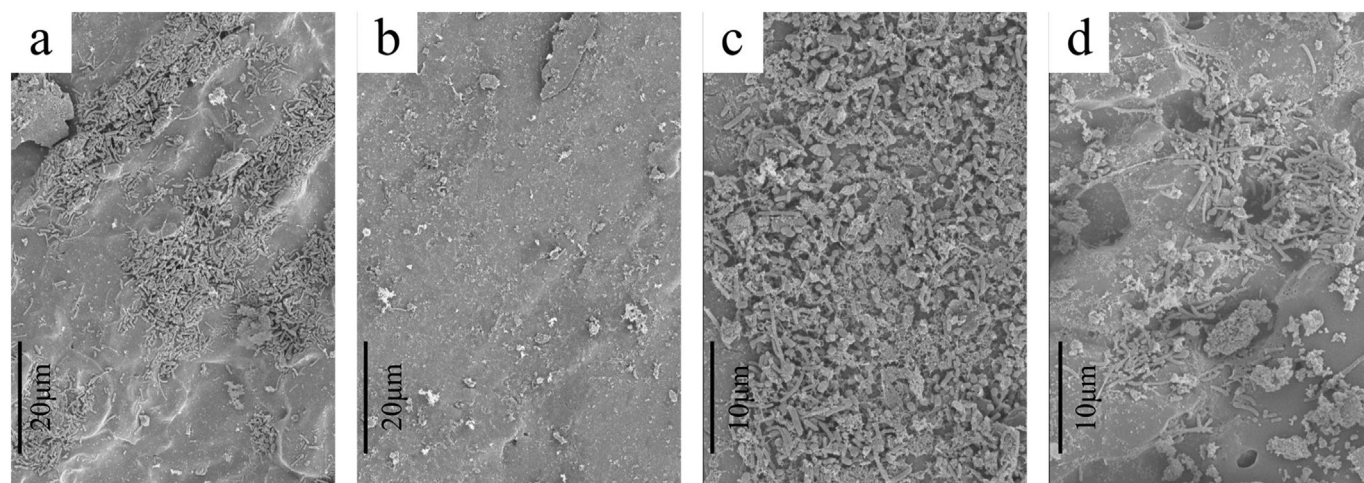
Fig. 11. L. innocua biofilms developed under turbulent flows. (a) \text{Re} = 9500 , 1 day. (b) \text{Re} = 16,500 , 1 day. (c) \text{Re} = 9500 , 7 days. (d) \text{Re} = 16,500 , 7 days. Figure adapted from [187].
