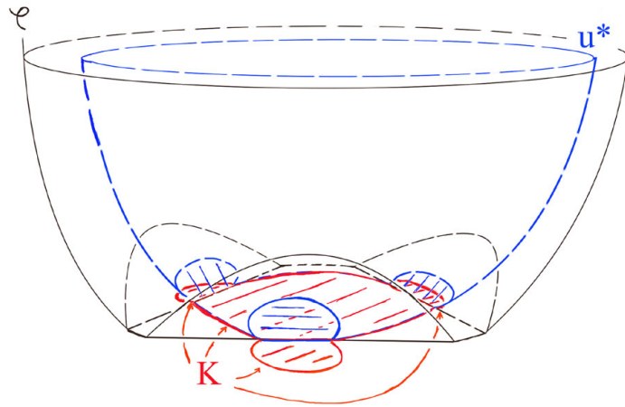
Fig. 4 The obstacle \varphi , the solution u^* , and the contact set K when \Gamma is a Y-shape
