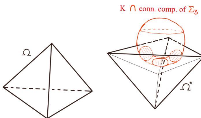
Fig. 2 A connected component of K \cap \Sigma_3 , in the case that \Omega and \Omega^* are tetrahedra in \mathbb{R}^3
