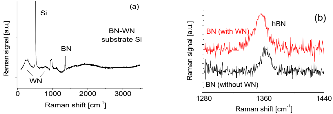
Figure 2. (a) Raman scattering spectrum of BN-WN nanocomposite, and (b) comparison of Raman spectra from BN-WN and BN materials.
