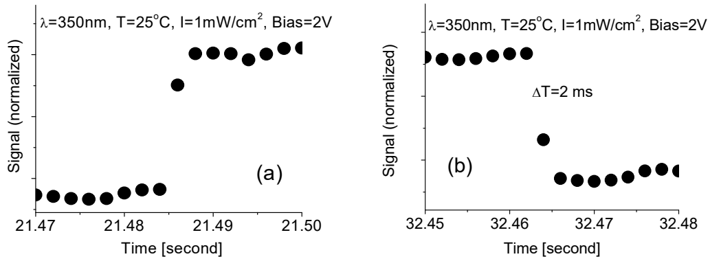
Figure 7. The time response of the DUV-PD exposed to 350nm light radiation at intensity of 1 mW/cm 2 , room temperature, and 2 V bias voltage.
