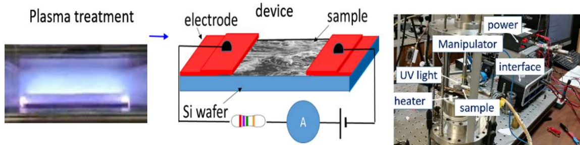
Figure 3. Process flow for nanocomposites based DUV-PD fabrication.
