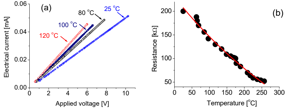
Figure 4. Current–voltage (I–V) properties of the DUV-PD.
