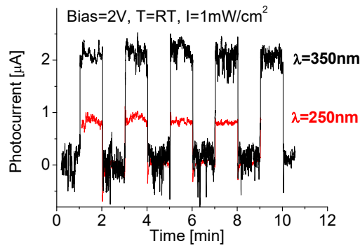
Figure 6. Responses of the device during cyclic tests with 2 minutes period at RT exposed to 250nm, and 350 nm UV radiations. RT: room temperature; \lambda : wavelength ; B: bias voltage.
