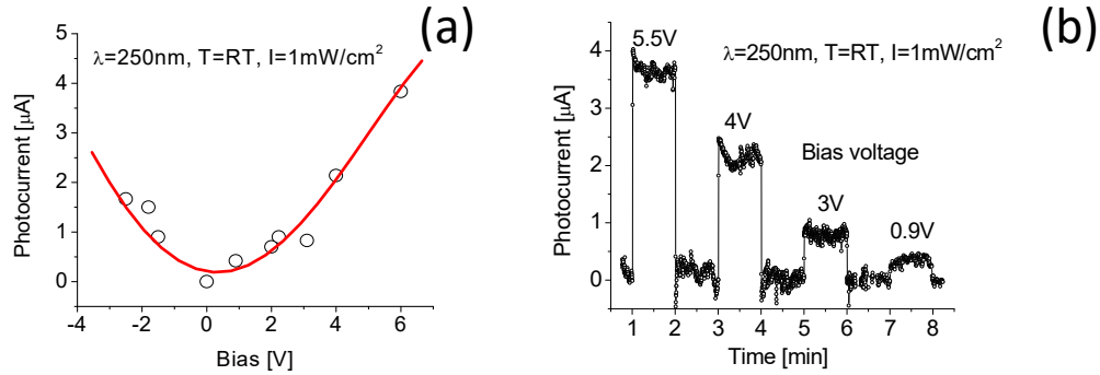
Figure 5. (a) The response of the DUV-PD as a function of the bias voltage magnitude, (b) time-dependent responses at different applied bias voltages with a fixed 250nm light radiation intensity and operating temperature.
