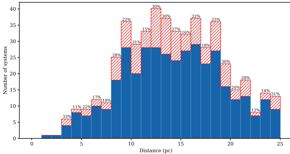
Figure 7. Number of systems in 1 pc shells outward from the Sun. Blue bars indicate single stars, red hatched bars are the multiples unresolved in Gaia DR2, and black labels indicate the multiplicity in each 1 pc bin based on known unresolved multiples as a fraction of each bin’s total. For bins with \geq 13 systems, the multiplicity is similar to that observed in volume-complete surveys such as Winters et al. (2019), which reported 27% multiplicity. Although the dropoff of systems past \sim 13 pc indicates that our survey is not volume-complete past that distance, the average multiplicity for those bins is 26%; therefore, our incompleteness is not biased toward single stars or multiples.
