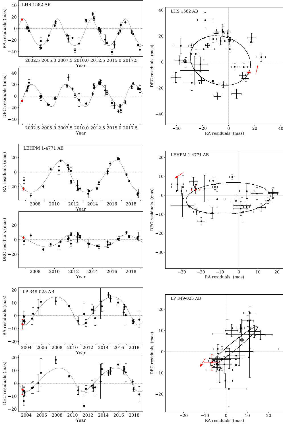
Figure 2. Astrometric residuals, after proper motion and parallax have been removed, for three nearby red dwarf systems showing perturbations indicative of orbiting companions. In each panel, the solid line represents the orbit fit to that system’s photocentric motion, for which the best-fit elements are given in Table 3. The first epoch is marked with a red point, and the red arrow indicates the direction of motion. In the right column, north is up, and east is to the right. Top to bottom: LHS 1582 AB ( P_{\text{orb}} = 5.23 yr), LEHPM 1-4771 AB (5.79 yr), and LP 349-025 AB (7.37 yr).
