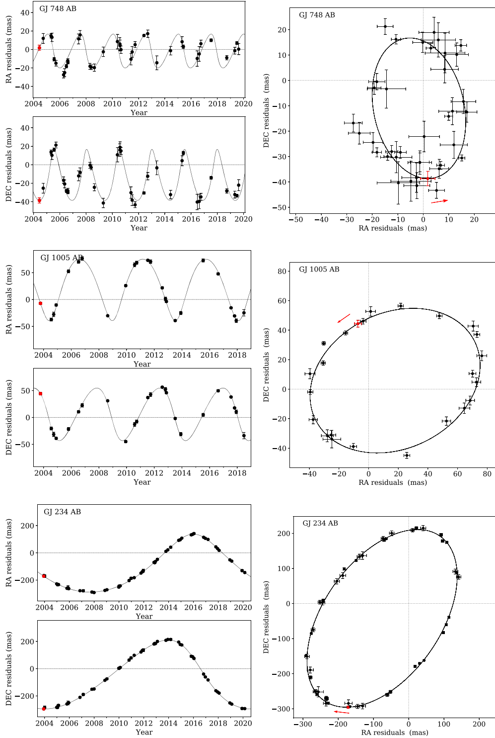
Figure 1. Astrometric residuals, after proper motion and parallax have been removed, for three nearby red dwarf systems showing perturbations indicative of orbiting companions. In each panel, the solid line represents the orbit fit to that system’s photocentric motion, for which the best-fit elements are given in Table 3. The first epoch is marked with a red point, and the red arrow indicates the direction of motion. In the right column, north is up, and east is to the right. These systems have well-known solutions in the literature, making them calibration systems for our observations and fitting routine. Top to bottom: GJ 748 AB ( P_{\text{orb}} = 2.49 yr), GJ 1005 AB (4.56 yr), and GJ 234 AB (11.16 yr).
