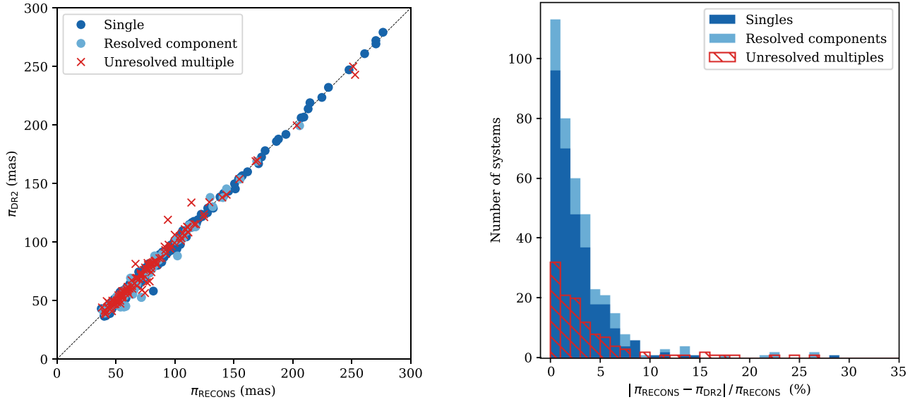
Figure 4. Parallax comparisons of RECONS astrometry to Gaia DR2 using M dwarfs within 25 pc, divided by their multiplicity status. Unresolved binaries or multistar systems are indicated with red symbols (left panel) and hatched bars (right panel), resolved components of multistar systems are light blue dots and bars, and presumed single stars are dark blue dots and bars. Left panel: RECONS parallax vs. DR2 parallax, with the dashed black line indicating the position of perfect agreement between those quantities. Right panel: difference (absolute value) between RECONS and DR2 parallax values, scaled by the corresponding RECONS parallaxes and expressed as percentages of those values. The singles and resolved components have been combined into a single histogram here, but the bars are colored to indicate the fraction belonging to each subset.
