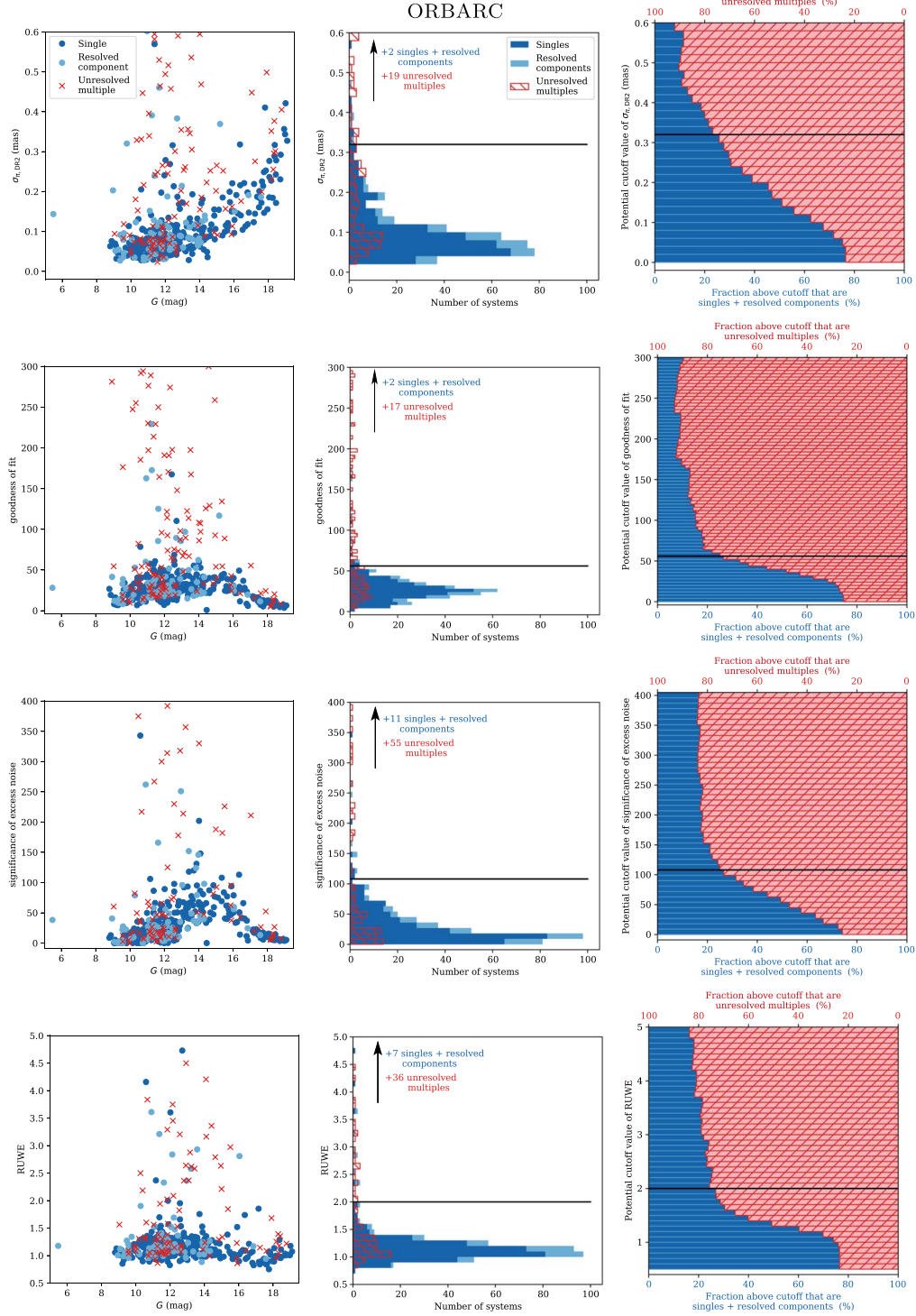
Figure 5. Astrometric fit parameters in DR2 that are useful for selecting potential unresolved multiples. In all panels, the color scheme is the same as in Figure 4. Left column: parameters for single systems, resolved components, and unresolved multiples in Gaia DR2, plotted against their Gaia G magnitudes. The unresolved multiples tend to have higher values of these fit parameters independent of their G magnitude, indicating their poor astrometric fits in DR2. Middle column: distributions of these parameters for systems in the left column, separated again by multiplicity status. Systems with values outside these plots are noted with the arrow and text in each panel. Although both distributions are peaked at low values of each parameter, the distribution of unresolved multiples extends to higher values. Right column: potential cutoff values for each parameter, showing the fraction of systems above each cutoff belonging to singles and resolved components (blue) and unresolved multiples (red). The cutoff values above which 75% of our systems are unresolved multiples (Section 7.3) are indicated with a horizontal black line.
