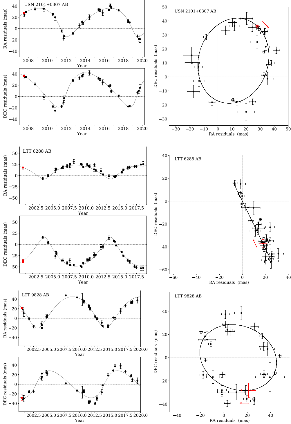
Figure 3. Astrometric residuals, after proper motion and parallax have been removed, for three nearby red dwarf systems showing perturbations indicative of orbiting companions. In each panel, the solid line represents the orbit fit to that system’s photocentric motion, for which the best-fit elements are given in Table 3. The first epoch is marked with a red point, and the red arrow indicates the direction of motion. In the right column, north is up, and east is to the right. Top to bottom: USN 2101+0307 AB ( P_{\text{orb}} = 7.53 yr), LTT 6288 AB (10.10 yr), and LTT 9828 AB (11.58 yr).
