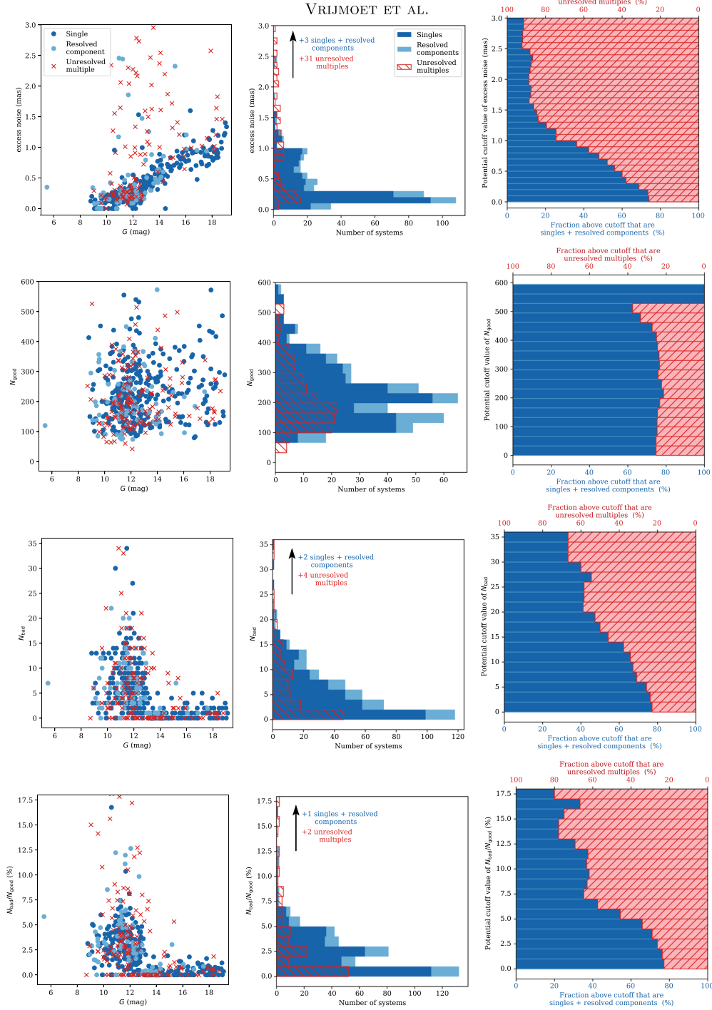
Figure 6. Four quantities in DR2 that are less useful for choosing potential unresolved multiples. The color schemes and columns are the same as for Figure 5, and any systems with values exceeding these ranges are noted with an arrow and text in each panel. For these quantities, the distributions of single and unresolved systems do not differ as significantly as those in Figure 5, making them less useful for identifying potential unresolved systems. Excess noise ( astrometric_excess_noise ) does show a distinction between singles and multiples, but it is less useful than the very similar astrometric_excess_noise_sig because it strongly depends on G magnitude (faint singles have values similar to brighter unresolved multiples).
