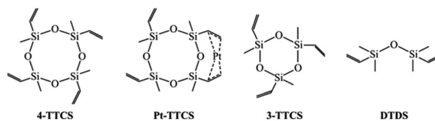
Fig. 1 Molecular structure of preceramic silicon oligomers.
