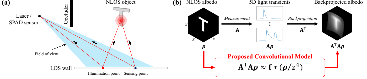
Figure 1. Overview of our convolutional model for NLOS imaging. (a) We capture transient measurements of light interacting with the NLOS scene through reflections on a relay LOS surface. (b) The measurement model \mathbf{A} maps the volumetric albedo \rho of the NLOS scene to 5D light transients, and the backprojection operation \mathbf{A}^\top maps 5D light transients to the backprojected albedo. We enable efficient and robust NLOS imaging by showing that the end-to-end mapping, modeled as the Gram operator \mathbf{A}^\top \mathbf{A} , is approximately convolutional.
