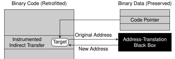
Figure 2. Abstraction of address translation mechanisms in binary rewriting.
