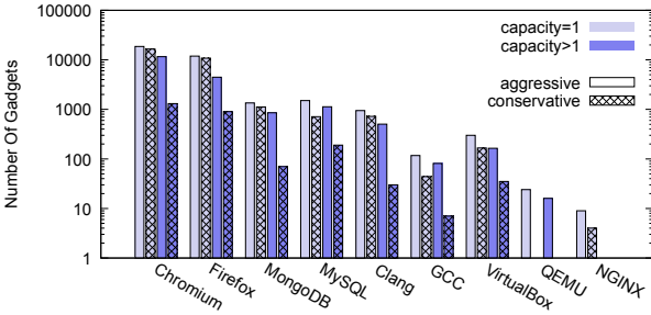
Figure 6. Distribution of RR* gadgets with trivial and non-trivial capacities. See Section 7.1 for definitions of aggressive and conservative assessment.
