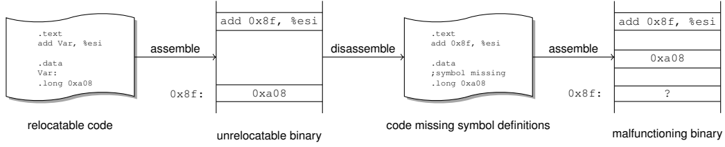
Figure 1. The relocation problem in binary rewriting.
