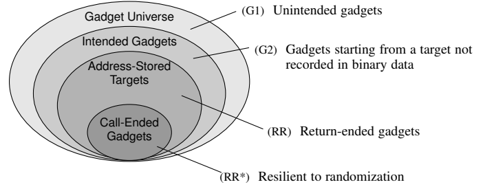
Figure 4. Gadget classification in code-reuse attacks. G1, G2, and RR refer to the differences between the enclosing and enclosed sets, respectively.
