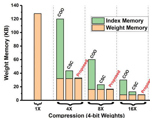
Figure 1: Comparison of index and 512 \times 512 weight memory for 4-bit weights with 4 \times , 8 \times , and 16 \times compression.
