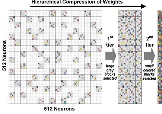
Figure 2: Proposed HCGS-based structured compression.
