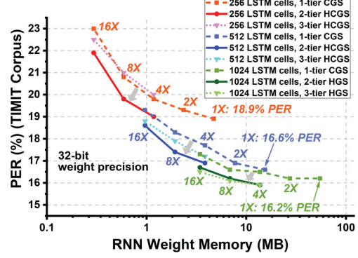
Figure 3: PER (TIMIT) comparison between single-tier CGS and multi-tier HCGS schemes.
