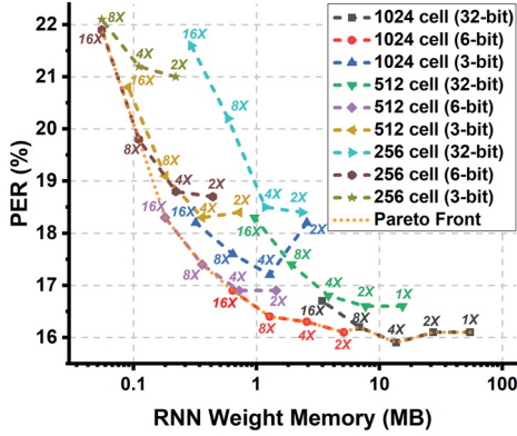
Figure 4: PER vs. RNN weight memory results for various 2-layer LSTMs for TIMIT.
