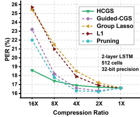
Figure 6: PER (TIMIT) comparison between HCGS and learned sparsity methods.
