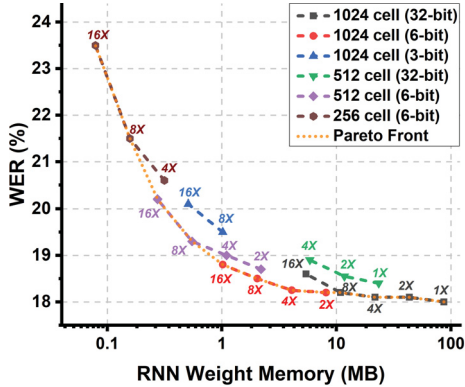
Figure 5: WER vs. RNN weight memory results for various 3-layer LSTMs for TED-LIUM.
