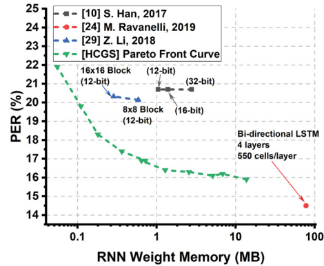
Figure 7: PER and memory comparison with prior LSTM works.
