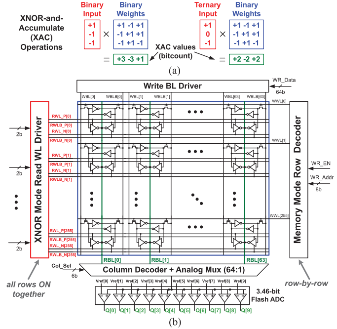
Fig. 1. (a) XAC operation illustration. (b) Proposed XNOR-SRAM macro architecture.
