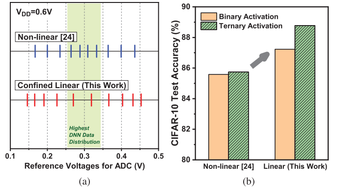
Fig. 7. Comparison of non-linear quantization [24] and confined linear quantization (this work). (a) Comparison of V_{ref} s for ADC. (b) CIFAR-10 accuracy improvement.
