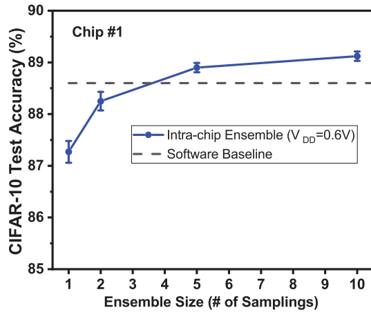
Fig. 20. Binary DNN accuracy improves with ensemble hardware exploiting intra-die variation.
