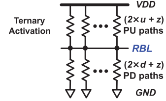
Fig. 4. PU/PD paths for V_{RBL} with ternary activations.
