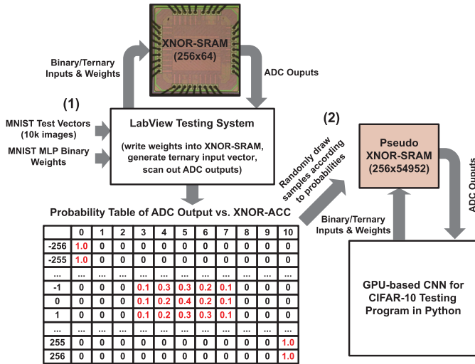
Fig. 18. Measurement-based simulation framework for CIFAR-10 accuracy evaluation using XNOR-SRAM macros.
