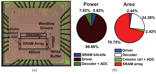
Fig. 8. (a) 65-nm XNOR-SRAM prototype chip micrograph. (b) Power and area breakdown.
