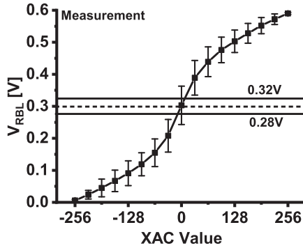
Fig. 13. Measured transfer function and variability.
