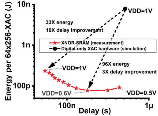
Fig. 12. Energy and delay comparison with digital baseline.
