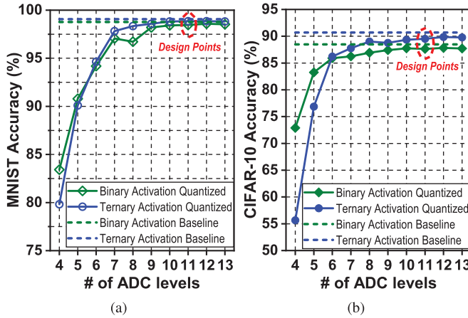
Fig. 6. (a) Accuracy of the MLP trained for MNIST and (b) accuracy of the CNN for CIFAR-10 as a function of ADC levels.
