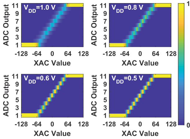
Fig. 15. Measured ADC output probability distribution as a function of XAC value at V_{DD} of 1.0, 0.8, 0.6, and 0.5 V.
