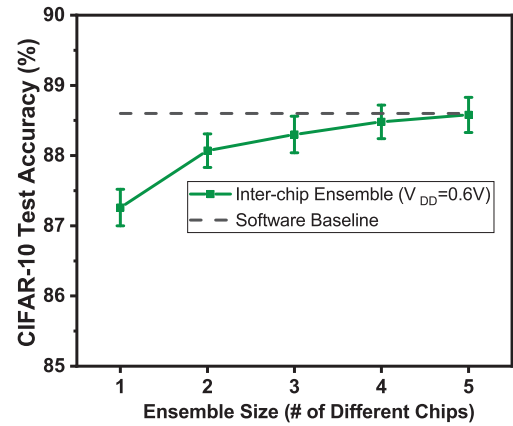
Fig. 21. Binary DNN accuracy improves with ensemble hardware exploiting intra-die variation from five different chips.
