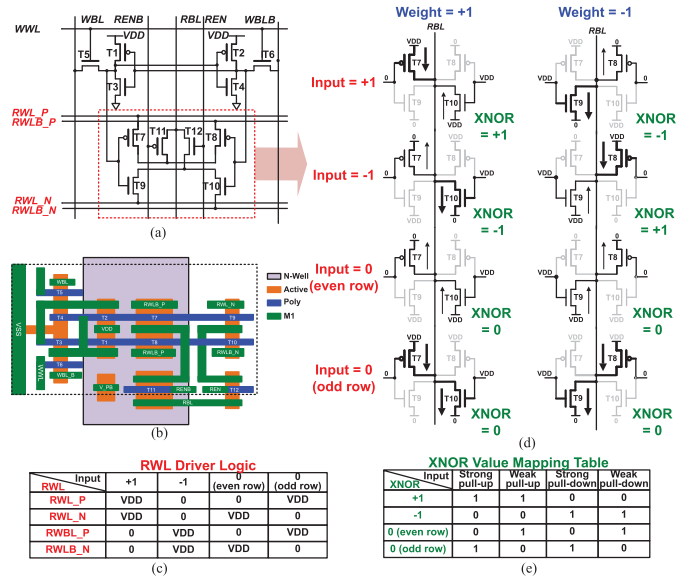
Fig. 2. XNOR-SRAM bitcell design and XNOR-ACC operation with ternary inputs/activations and binary weights. Bitwise ternary-XNOR output from each bitcell forms pull-up (PU)/pull-down (PD) paths on the RBL voltage, which represents the XNOR-ACC value.
