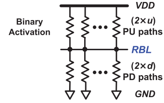
Fig. 3. PU/PD paths for V_{RBL} with binary activations.
