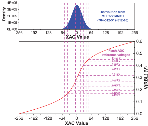
Fig. 5. XAC is mapped to V_{RBL} . The confined linear quantization scheme is shown, along with the corresponding ten reference voltages ( V_{ref} ) for the 11-level flash ADC.
