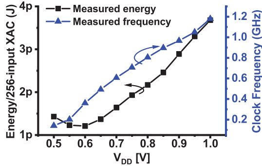
Fig. 10. Energy and frequency scaling with supply voltage.
