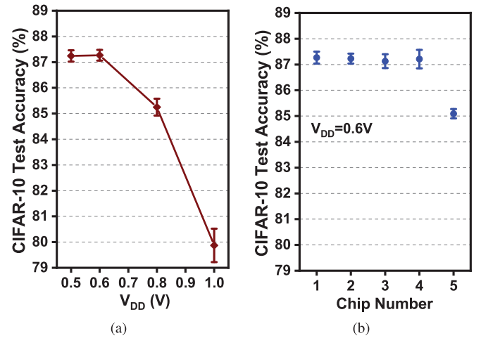
Fig. 19. Accuracy characterization of binary CNN for CIFAR-10. (a) Accuracy for chip #1 across different supply voltages. (b) Accuracy distribution for five different chips at 0.6 V.
