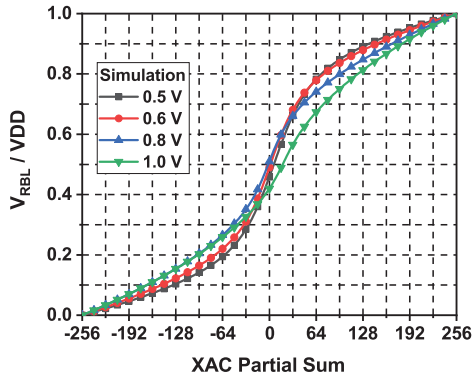
Fig. 16. Normalized transfer function at different values of V_{DD} .
