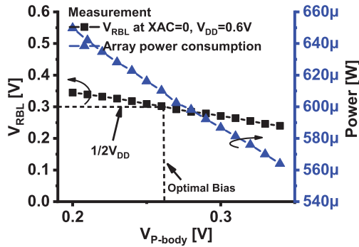
Fig. 14. Body bias tuning for PMOS/NMOS mismatch.
