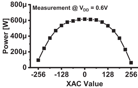
Fig. 9. Data-dependent XNOR-SRAM power.
