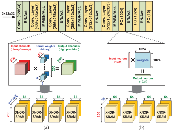
Fig. 17. Mapping (a) convolution layers and (b) FC layers of deep CNNs onto XNOR-SRAM arrays.
