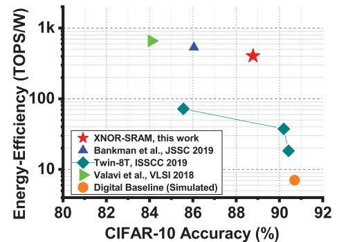
Fig. 22. Energy efficiency (TOPS/W) and CIFAR-10 accuracy comparison against in-/near-memory computing literature.
