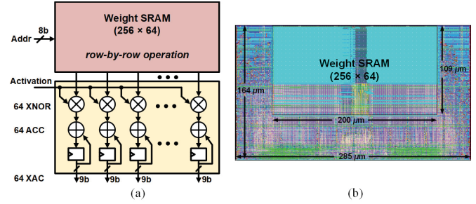
Fig. 11. Digital baseline design for XAC accelerator. (a) Block diagram. (b) Layout in 65-nm CMOS.
