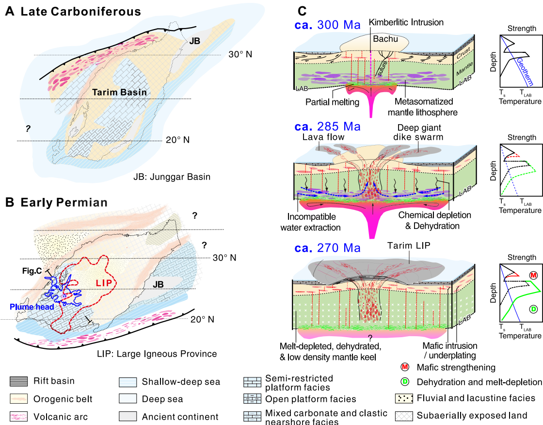
Figure 3. Model of the Tarim Permian mantle plume. (A–B) Paleogeography (Chen et al., 2006; Li et al., 2014) with plume head imaged from this study. (C) Block models of plume evolution with corresponding schematic lithospheric strength profiles and geotherm. The plume impinged on previously deformed continental lithosphere beneath the Bachu Uplift, followed by large igneous province (LIP) volcanism. Plume process modified crustal strength, with mafic intrusions and underplating, and the mantle via mantle dehydration and melt depletion. Mantle lithosphere was thickened and strengthened, constructing Tarim as a strong low-heat-flow continent. Geotherm connects the surface temperature ( T_s ) to fixed lithosphere-asthenosphere boundary (LAB) temperature ( T_{LAB} ); see details in the Supplemental Material [see footnote 1]).
