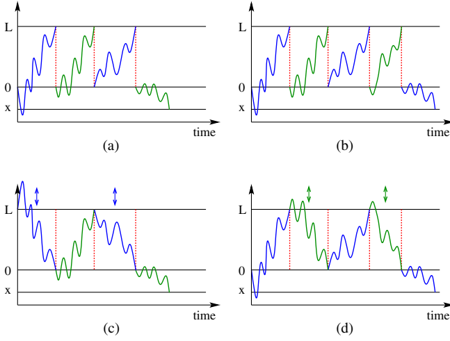
FIG. 2. Schematic of diffusion with first-passage resetting. Shown are paths from (0,0) to (x,t) with (a) an odd number or (b) an even number of reset events. We transform either the odd-numbered or the even-numbered pieces of the original path through the reflection x(t) \rightarrow L - x(t) to yield free diffusion from either (c) (L,0) to (x,t) or (d) (0,0) to (x,t) . Summing over all numbers of reset events gives Eq. (5b).
