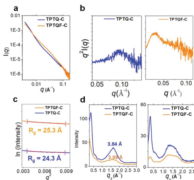
Fig. 3 (a) SAXS scattering intensity, I(q) of TPTQ-C (blue) and TPTQF-C (orange) versus scattering vector q in THF solution ( 5 \text{ mg mL}^{-1} ). (b) Kratky plots, q^2 \times I(q) vs. q showing the folded peaks in small q -range. (c) Fitting \ln[I(q)] - q^2 to Guinier relationship to calculate the radius of gyration, R_g . (d) GIWAXS profile along q_z (out-of-plane) and q_y (in-plane) in thin-films.
