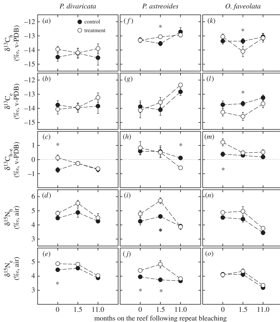
Figure 2. Average stable carbon isotopes of the animal host ( \delta^{13}\text{C}_h ) and endosymbiont ( \delta^{13}\text{C}_e ), \delta^{13}\text{C}_{h-e} and the stable nitrogen isotopes of the animal host ( \delta^{15}\text{N}_h ) and endosymbiont ( \delta^{15}\text{N}_e ) of (a–e) Porites divaricata , (f–j) Porites astreoides and (k–o) Orbicella faveolata after 0, 1.5 and 11 months on the reef following repeat bleaching. For \delta^{13}\text{C}_{h-e} , heterotrophic C is preferentially incorporated into tissues when the difference is less than 0, whereas photosynthetic C is preferentially incorporated when the difference is greater than or equal to 0. Averages are shown \pm 1 s.e. Asterisks indicate significant differences between treatment and control corals within a time point and species. Sample size per average ranges from 3 to 9. Statistical results shown in the electronic supplementary material, table S3.
