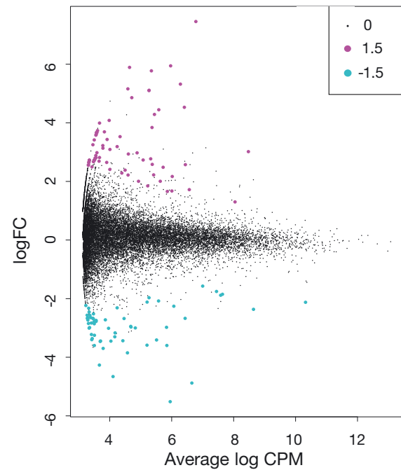
Fig. 3. Fitted model mean-difference plot showing expression changes between tolerant and susceptible Acropora colonies ( n = 18 per group). The \log_2 fold-change (FC) for each gene is plotted against the average abundance in \log_2 counts per million (CPM). Pink (blue) points show genes that are significantly upregulated (downregulated) in tolerant colonies relative to susceptible colonies. Significant differentially expressed genes were determined using the 'glmTreat' function in R to specify both a \log_2 FC cut-off of 1.5 as well as a false discovery rate of 5 %
