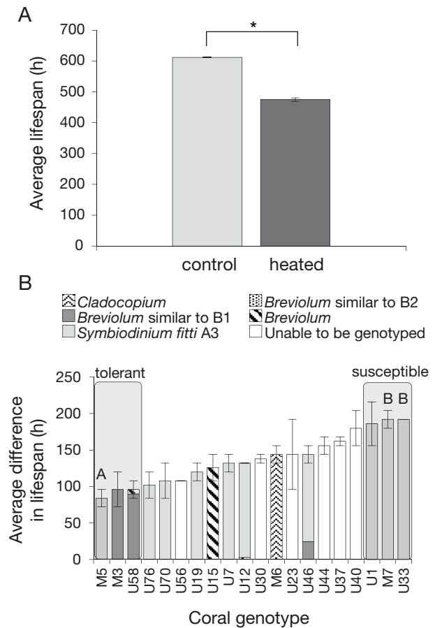
Fig. 1. (A) Average lifespan for Acropora cervicornis coral fragments maintained at either ambient (control: n = 60 ) or elevated temperatures (heated: n = 40 ). Significant differences ( p < 0.05 ) are denoted by an asterisk (*) and error bars show SE. All control fragments survived for the duration of the experiment, so there was no difference in lifespan among the control fragments (SE = 0). (B) Average difference in lifespan between heated and control fragments over 26 d for 20 A. cervicornis genotypes ( n = 2 per genotype). Significantly different genotypes ( p < 0.05 ) are indicated by different letters as determined by a Tukey's HSD post hoc test. Error bars show SE. The boxes at either end of the x-axis indicate the 3 most thermal tolerant and the 3 most thermal susceptible genotypes that were selected for comparisons of gene expression. Patterns of each bar indicate the proportion of cp23S reads attributed to different Symbiodiniaceae operational taxonomic units (OTUs) within each coral colony. Representatives were assigned to OTUs using NCBI BLAST. Variants of the same taxa were combined per coral genotype (see Table S2 for complete list of variants per genotype and total cp23S reads). The cp23S region could not be amplified for genotypes U23, U30, U37, U40, U44, and U56 ('unable to be genotyped'). Note: Breviolum similar to B2 and Cladocopium make up less than 5% of the total reads for genotypes M3, U12, and U1. While Cladocopium cp23S reads make up 100% of the reads from M6, only 9 reads could be successfully identified compared to >1000 reads for all other samples, and this sample was therefore removed from further Symbiodiniaceae analyses
