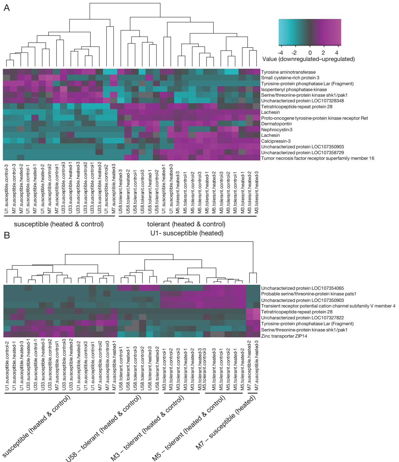
Fig. 6. Heat map across all samples using the (A) significant differentially expressed (DE) genes between tolerant and susceptible Acropora genotypes in the control treatment only ( n = 9 per group), and (B) significant DE genes between tolerant and susceptible genotypes in the heated treatment only ( n = 9 per group). Colors range from pink (significantly upregulated in tolerant colonies relative to susceptible colonies) to blue (significantly downregulated in tolerant colonies) and are based on the log counts per million. Significant DE genes were determined using the 'glmTreat' function in R to specify both a \log_2 fold-change cut-off of 1.5 as well as a false discover rate of 5%. Genes are ordered from top to bottom by ascending p-value: 8.10 \times 10^{-8} to 4.46 \times 10^{-5} (A); 4.11 \times 10^{-7} to 2.58 \times 10^{-5} (B)
