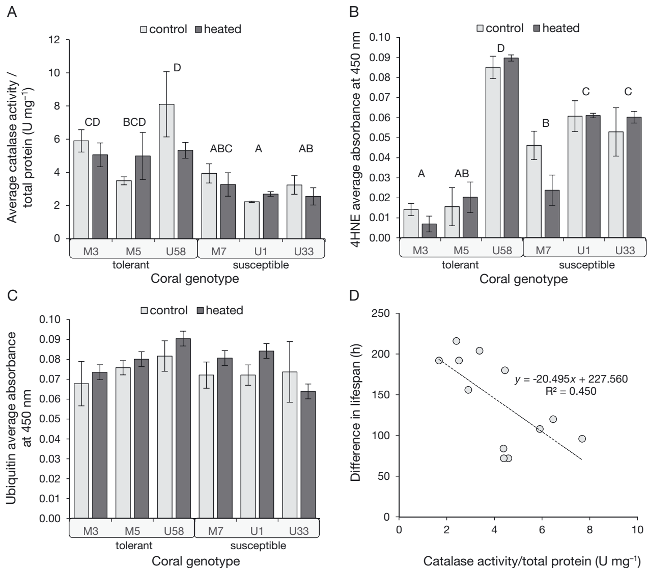
Fig. 7. Differences in average (A) catalase activity, (B) 4HNE concentration as measured by relative absorbance, and (C) ubiquitin concentration as measured by relative absorbance for the 3 most thermal tolerant and 3 most susceptible Acropora genotypes ( n = 3 per bar). Different letters indicate significant pairwise differences between genotypes based on Tukey's HSD post hoc test. Error bars show standard error. (D) Model I linear regression showing the relationship of difference in lifespan of the 3 most tolerant and the 3 least tolerant genotypes to catalase activity in the heated treatment ( n = 12 )
