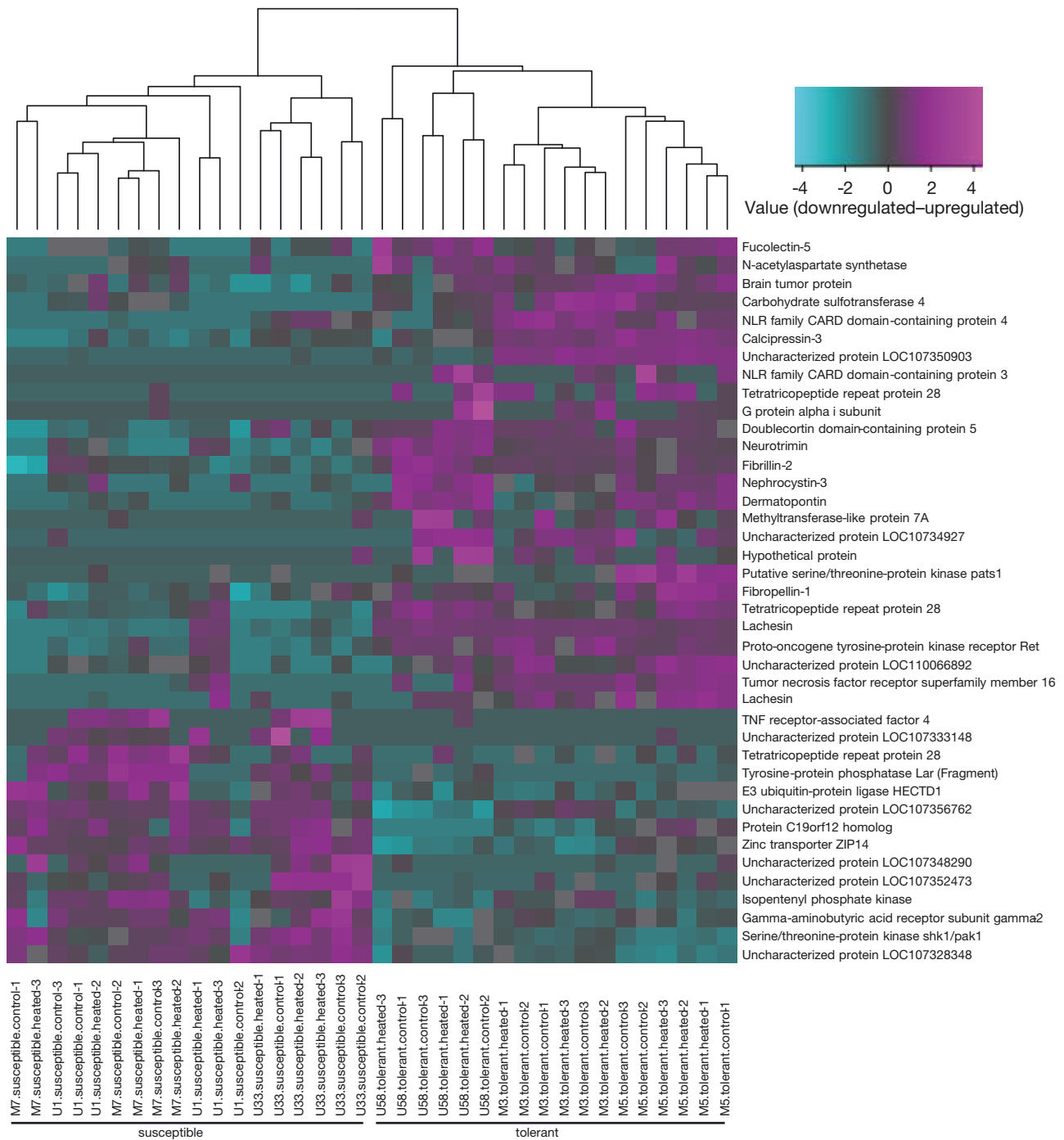
Fig. 5. Heat map across all samples using the 40 significant differentially expressed (DE) genes between tolerant and susceptible Acropora genotypes ( n = 18 per group) that were the most consistent among genotypes within tolerant and susceptible groupings. Colors range from pink (significantly upregulated in tolerant colonies relative to susceptible colonies) to blue (significantly downregulated in tolerant colonies) and are based on the log counts per million. Significant DE genes were determined using the 'glmTreat' function in R to specify both a \log_2 fold-change cut-off of 1.5 as well as a false discovery rate of 5%. Consistent genes were determined by taking each DE gene and comparing the average control and heated reads per kilobase of transcript, per million mapped reads (RPKM) for each genotype to the average RPKM for that gene for tolerant or susceptible colonies and seeing whether they matched expectations (based on the 'glmTreat' results) for either upregulation or downregulation. Genes are ordered from top to bottom by ascending p-value ( 3.41 \times 10^{-10} to 3.71 \times 10^{-4} )
