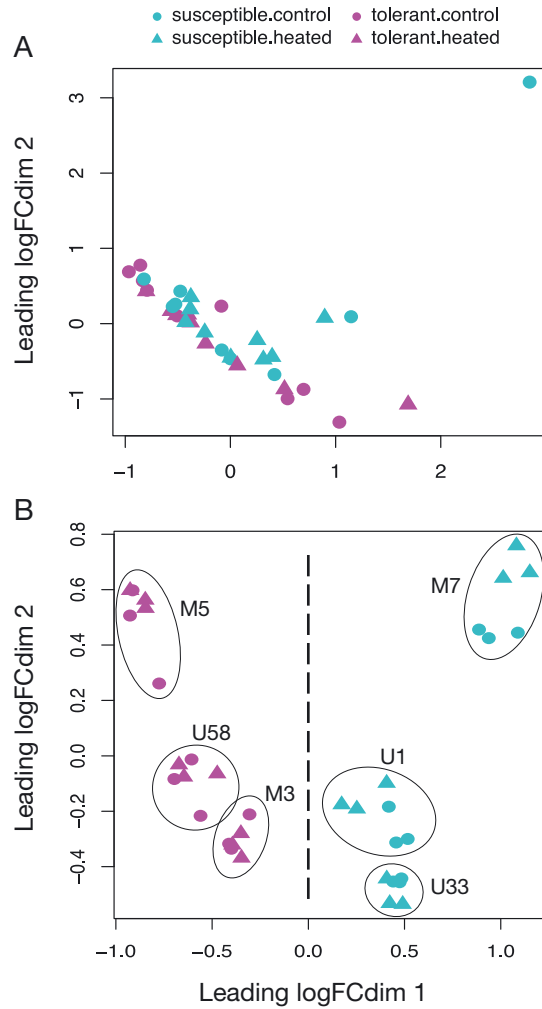
Fig. 2. Multidimensional scaling plot showing: (A) the overall differences between mRNA expression profiles of susceptible Acropora colonies at ambient temperature ( 28 \pm 1^\circ\text{C} ), susceptible colonies at elevated temperature ( 32 \pm 1^\circ\text{C} ), tolerant colonies at ambient temperature, and tolerant colonies at elevated temperature ( n = 9 per group), and (B) the differences in the mRNA expression profiles of the 129 significantly differentially expressed (DE) genes between tolerant and susceptible colonies among the same 4 groups. Significant DE genes were determined using the 'glmTreat' function in R to specify both a \log_2 fold-change (FC) of 1.5 as well as a false discovery rate of 5 %
