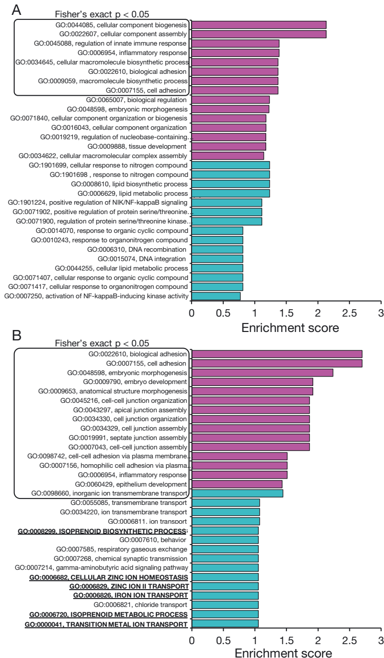
Fig. 4. (A) Gene ontology (GO) term enrichment analysis for the 93 significant differentially expressed (DE) genes among tolerant and susceptible Acropora genotypes ( n = 18 per group) that had GO term annotations. (B) GO term enrichment analysis for the 30 DE genes that had GO term annotation and were significant between tolerant and susceptible genotypes ( n = 18 per group) but were also considered consistent in expression among the genotypes within tolerance groups. (A,B) For GO term enrichment analysis, biological process ontology was used. The enrichment score for each GO term was determined by taking the -\log_{10} of the p-value from the Fisher's exact test using the classic algorithm in 'topGO.' The top 15 enriched GO terms in genes that were significantly upregulated in tolerant colonies relative to susceptible colonies (pink), as well as in genes that were significantly downregulated in tolerant colonies (blue) are shown. A box is used around GO terms that were significantly enriched in these gene sets based on the Fisher's exact test ( p < 0.05 ). Terms in bold and underlined are GO terms that were also significantly enriched in significant DE genes downregulated in either tolerant vs. susceptible colonies in the heated treatment (cellular zinc homeostasis, zinc II ion transport, iron ion transport, transition metal ion transport) or tolerant vs. susceptible colonies in the control treatment (isoprenoid biosynthetic process, isoprenoid metabolic process)
