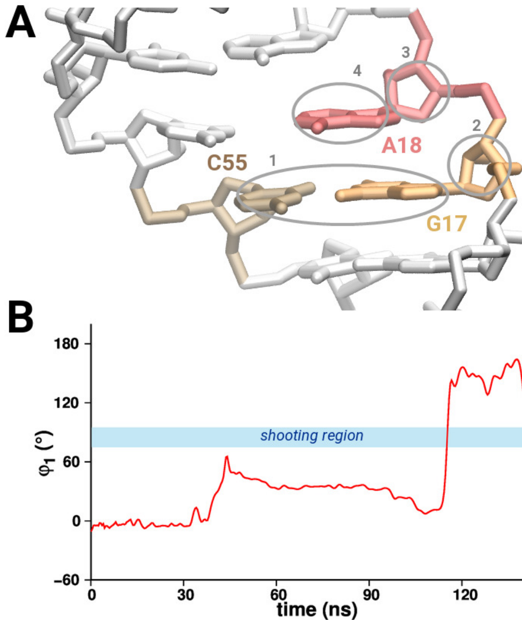
Figure 2: Details on the primary order parameter. (A) The OP is defined by the center of mass of each of the following four groups: the nitrogenous bases of C55 and G17 (labeled 1), sugar moiety attached to G17 (labeled 2), sugar moiety attached to A18 (labeled 3), and the nitrogenous base of A18 (labeled 4). Each key nucleotide is also uniquely colored and labeled. (B) Shown is a time trace of the primary OP in the seed trajectory (red). A cyan rectangle highlights the shooting region. See also Figure S2.
