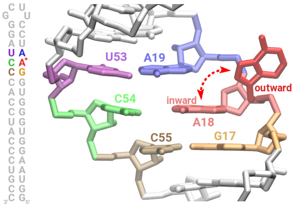
Figure 1: Sequence and structural details of bases involved in conformational transitions. ( left ) Secondary structure of dsRNA with key nucleotides highlighted. The nucleobase studied in this work is marked with an asterisk. ( right ) A side-view of the three-dimensional structure of dsRNA where each key nucleotide is highlighted in a unique color and labeled. Specifically, A18 is shown both in the flipped in and out conformations. The solvated simulation domain is shown in Figure S1.
