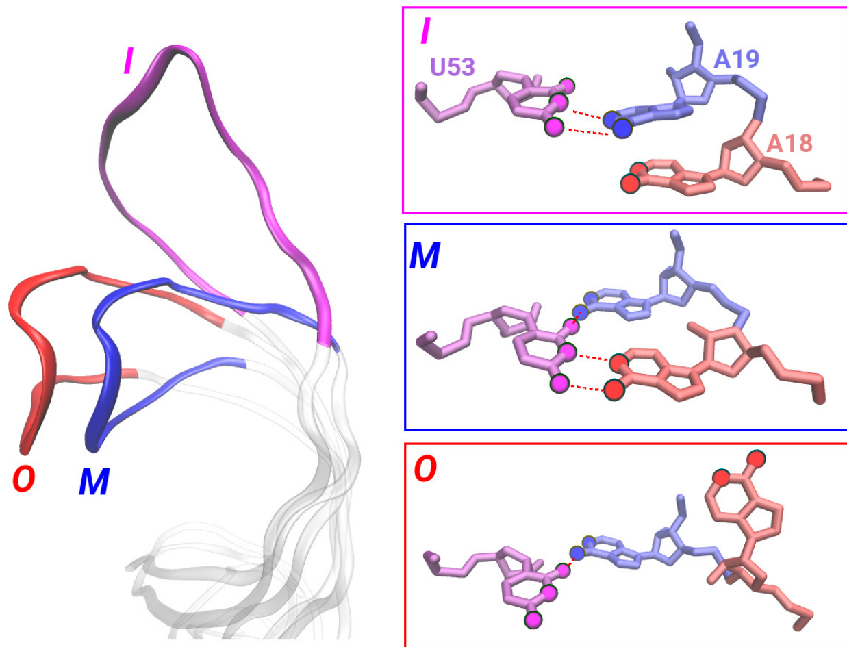
Figure 5: Global and local conformational dynamics in dsRNA. ( left ) Snapshot of global conformational changes in the RNA stem loop derived from shooting trajectories at three different states: I (magenta), M (blue), and O (red). ( right ) Snapshots of the flipping site in three different states. Each key nucleotide and atoms that participate in hydrogen bonding (marked by dotted red lines) are uniquely colored.
