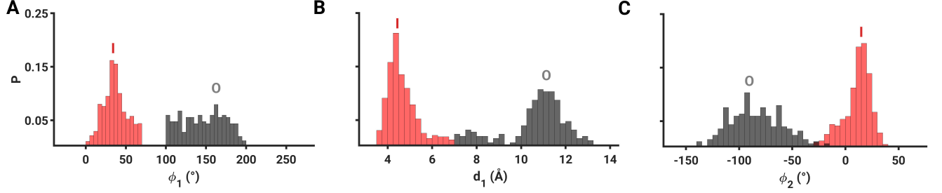
Figure 3: Population distributions of CVs at terminal points. Shown are the distributions of CVs at terminal points of transition paths for the inward (red) and outward (gray) states. (A) The pseudo-dihedral angle ( \phi_1 ) that describes the position of A18 relative to G17. (B) The distance ( d_1 ) between the centers of mass of G17 and A18. (C) The pseudo-dihedral angle ( \phi_2 ) that describes the position of A18 relative to A19. See also Figure S3.
