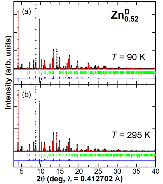
FIG. 1. Rietveld refinements of synchrotron PXRD data of deuterated Zn 0.52 D at (a) T = 90 K and (b) T = 295 K in space group P6_3/mmc . Observed (black), calculated (red), and difference (blue) plots are shown, and Bragg reflections are indicated by green tick marks. The Bragg reflections of a LiF impurity phase are marked with orange tick marks.
