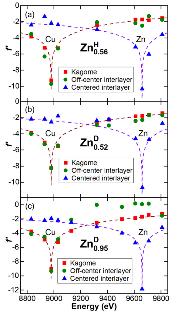
FIG. 3. Anomalous dispersion factor f' as a function of incident energy for the kagome, off-center interlayer ( C_{2v} ), and centered interlayer ( D_{3h} ) sites in (a) protonated \text{Zn}_{0.56}^{\text{H}} , (b) deuterated \text{Zn}_{0.52}^{\text{D}} , and (c) deuterated \text{Zn}_{0.95}^{\text{D}} . The theoretical values for Cu and Zn are shown as maroon and purple dashed lines, respectively.
