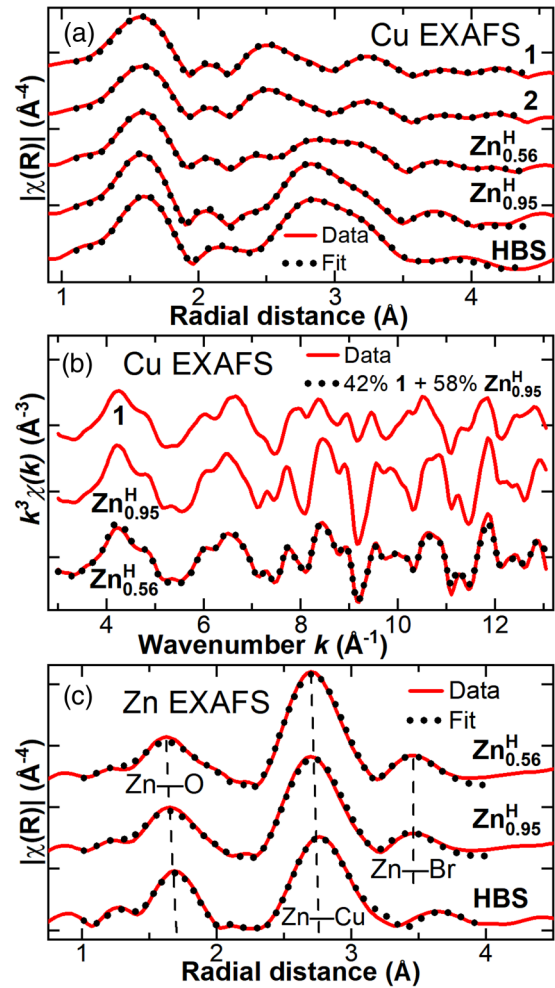
FIG. 2. (a) Real-space Cu K -edge EXAFS data and fits of barlowite 1, barlowite 2, \text{Zn}_{0.56}^{\text{H}} , \text{Zn}_{0.95}^{\text{H}} , and herbertsmithite (HBS) showing the magnitude of the Fourier-transformed EXAFS ( \chi(R) ) measured at T = 10 K. (b) Linear component fit of normalized \text{Zn}_{0.56}^{\text{H}} Cu EXAFS data of barlowite 1 and \text{Zn}_{0.95}^{\text{H}} . (c) Real-space Zn K -edge EXAFS data and fits to \text{Zn}_{0.56}^{\text{H}} , \text{Zn}_{0.95}^{\text{H}} , and herbertsmithite (HBS) measured at T = 10 K. The three paths for Zn-substituted barlowite are shown as dashed lines. Vertical offsets have been applied to separate the spectra.
