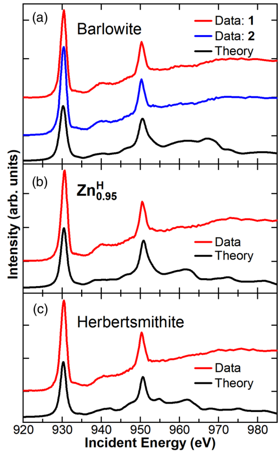
FIG. 5. Comparison of room temperature experimental Cu L -edge XANES spectra with simulations for (a) barlowite 1 and 2, (b) \text{Zn}_{0.95}^{\text{H}} , and (c) herbertsmithite. Vertical offsets have been applied to separate the spectra. To match the experimental spectra, the calculated spectra were broadened with a 0.6 eV Gaussian and a 0.8 eV Lorentzian broadening.
