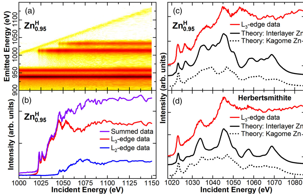
FIG. 6. (a) Zn L -edge RIXS plane of \text{Zn}_{0.95}^{\text{H}} showing the L_{\alpha} fluorescence with emitted energy of 1012 eV and the L_{\beta} fluorescence with emitted energy of 1035 eV, corresponding to the L_3 and L_2 edges, respectively. Fluorescence from the Cu L_{\alpha} and L_{\beta} lines are visible between 920 and 960 eV, and the elastic scattering is visible as a diagonal line. A log scale has been used on the color map to emphasize the faint elastic line. (b) Zn L -edge XANES data of \text{Zn}_{0.95}^{\text{H}} measured at T = 300 K. The TES detector allows the L_2 -edge and L_3 -edge data to be separated; they are shown along with the summed data. Zn L_3 -edge XANES data of (c) \text{Zn}_{0.95}^{\text{H}} and (d) herbertsmithite measured at T = 300 K, along with simulations based on the experimentally determined crystal structure (“interlayer Zn”) and simulations where Zn occupies one of the kagome sites while Cu occupies the respective interlayer site in each structure (“kagome Zn”; see discussion in the text). In (c) and (d), vertical offsets have been applied to separate the spectra. The calculated Zn spectra were broadened by convolution with a 0.8-eV Gaussian broadening, and the nonexcitonic portion had an additional 0.8-eV Lorentzian broadening.
