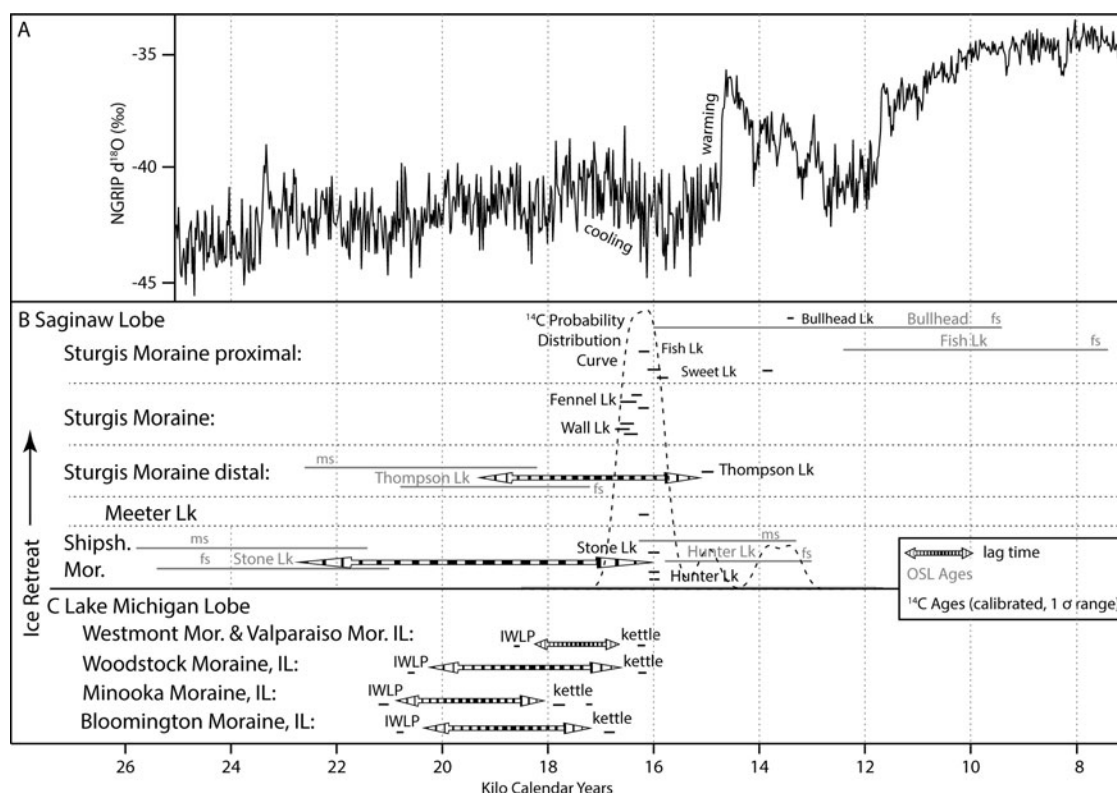
Figure 7. Summary of ages from the study area and those discussed from the Lake Michigan Lobe. (A) Climate proxy data ( \delta^{18}O ) from NGRIP, indicating that any climate amelioration within the study area at ~16.5 cal ka BP does not coincide with warming in Greenland. Data from Rasmussen et al. (2014). Age distributions for (B) Saginaw Lobe and (C) Lake Michigan Lobe. Dashed black line is the probability distribution plot of all radiocarbon ages for Saginaw Lobe from this study. In (B) the offset between optically stimulated luminescence (OSL) and radiocarbon ages for Stone and Thompson lakes represents lag time between deglaciation and lake formation. Younger OSL ages from Bullhead, Hunter, and Fish Lake record younger fluvial or lacustrine sediment. In (C) the lag time in Illinois is recorded by the difference in age between oldest organics in the ice walled lake plain (IWLP) and kettle lakes associated with the same moraine.
