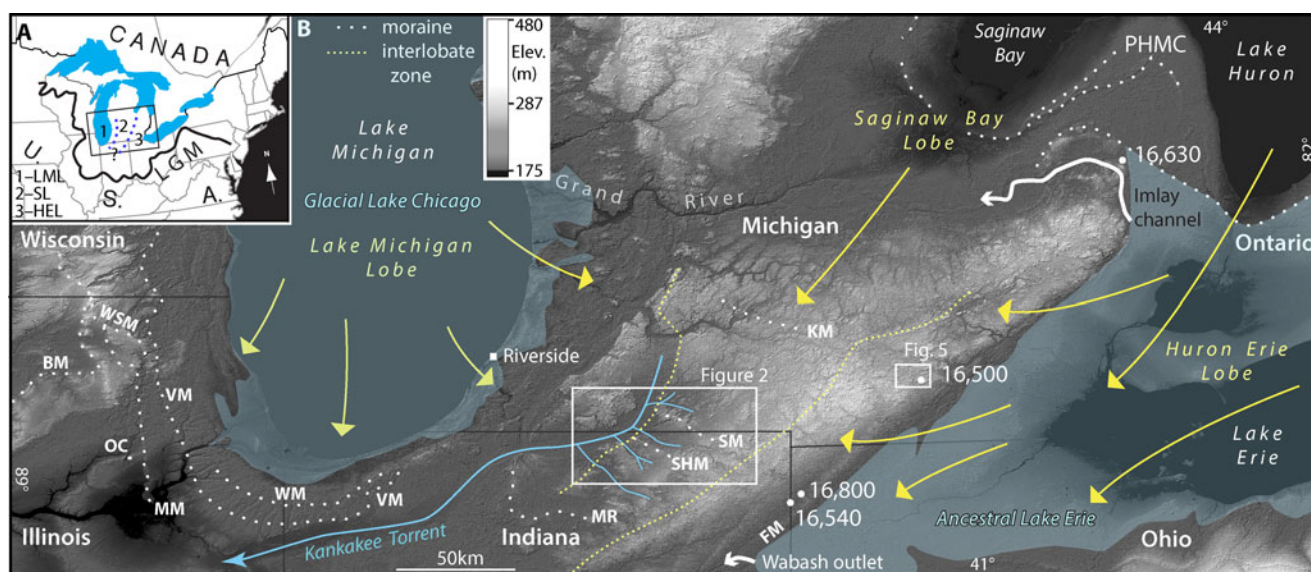
Figure 1. Regional maps of the study area. (A) Location map showing the last glacial maximum (LGM) extent of the Laurentide Ice Sheet. HEL, Huron-Erie Lobe; SL, Saginaw Lobe; LML, Lake Michigan Lobe. (B) Digital elevation model (DEM) map showing relationships between the Lake Michigan, Saginaw Bay, and Huron-Erie lobes (yellow arrows) that converged onto the higher relief area indicated by light gray tones of the study area in Figure 2. Distribution of specific radiocarbon ages (median cal ka BP) are indicated with white dots from Dyke (2004) and Glover et al. (2011). Long, thick, white arrow is the drainage route through the Imlay Channel across the Thumb of Michigan routing water from ancestral Lake Erie through the Grand River to glacial Lake Chicago within the Lake Michigan basin. Ancestral Lake Erie shown at Maumee stage and glacial Lake Chicago at the Glenwood stage. BM, Bloomington Moraine; OC, Oswego Channel; MM, Minooka Moraine; VM, Valparaiso Moraine; WM, Woodstock Moraine; WSM, Westmont Moraine; MR, Maxinkuckee Moraine; SHM, Shipshewana Moraine; SM, Sturgis Moraine; KM, Kalamazoo Moraine; FM, Fort Wayne Moraine; PHMC, Port Huron Moraine complex. (For interpretation of the references to color in this figure legend, the reader is referred to the web version of this article.)
