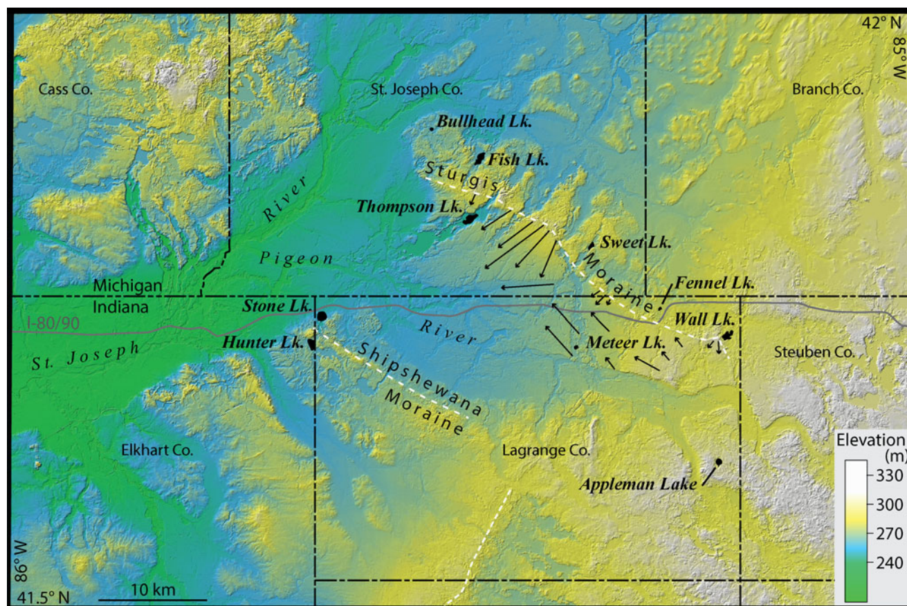
Figure 2. (color online) Location of the Shipshewana and Sturgis moraines and lakes cored on a regional digital elevation model. Black arrows are flow directions on fans recording former ice-margin positions.
