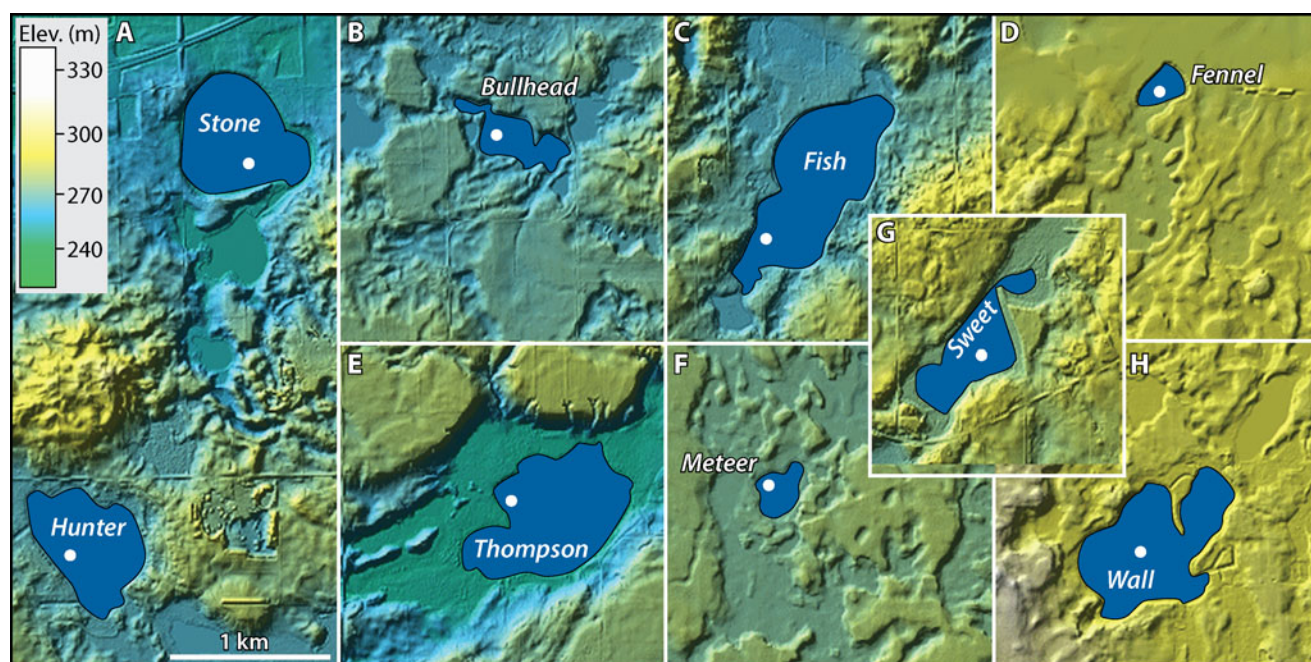
Figure 3. (color online) Closeup DEMs of kettle and tunnel channel lakes cored (white dots). Individual lakes are (A) Stone (upper), Hunter (lower), (B) Bullhead, (C) Fish, (D) Fennell, (E) Thompson, (F) Meteor, (G) Sweet, (H) Wall. Scale, north at the top, and hypsometric tinting in (A) is the same for all panels. See Figure 2 for location of lakes.
