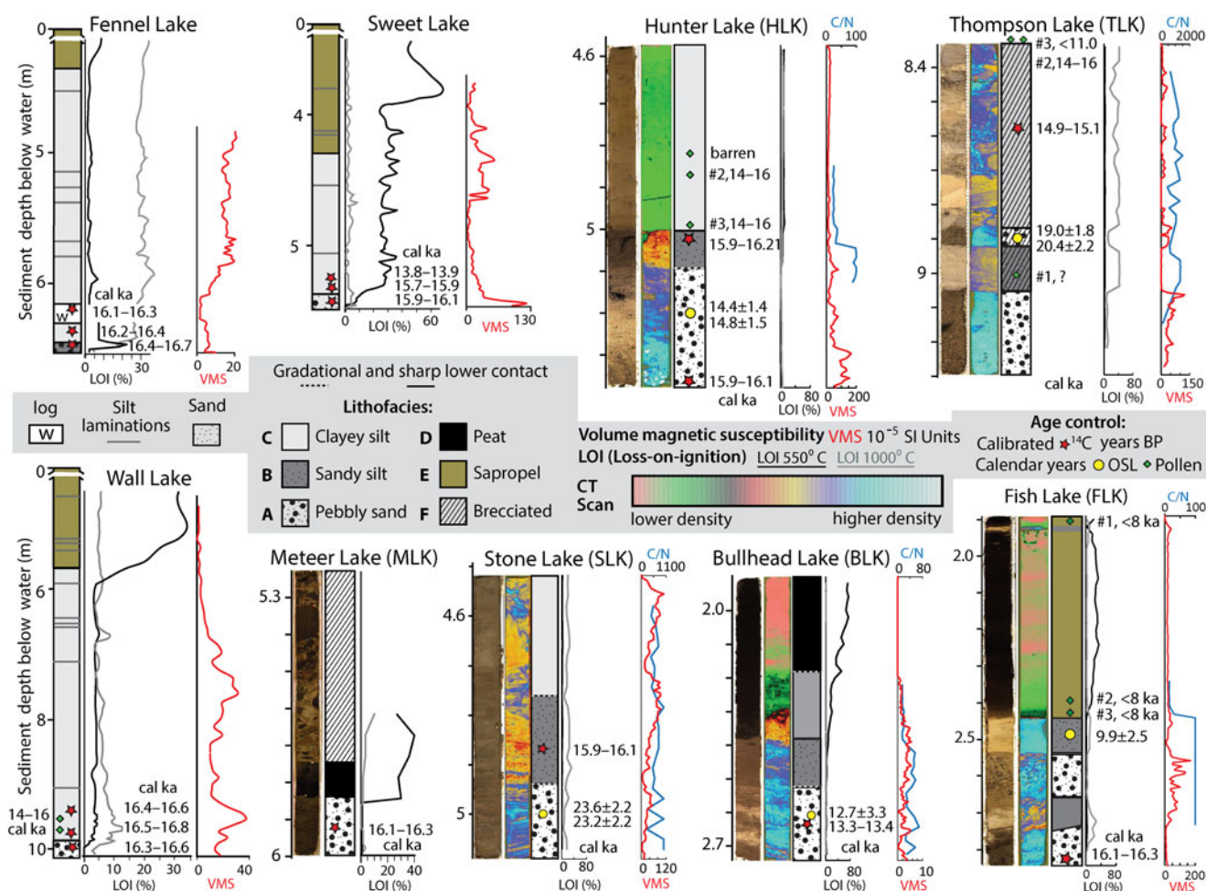
Figure 4. (color online) Lithostratigraphic facies, proxy data, and chronology of the nine cores. Core locations shown on Figures 2, 3, and in Table 1.
