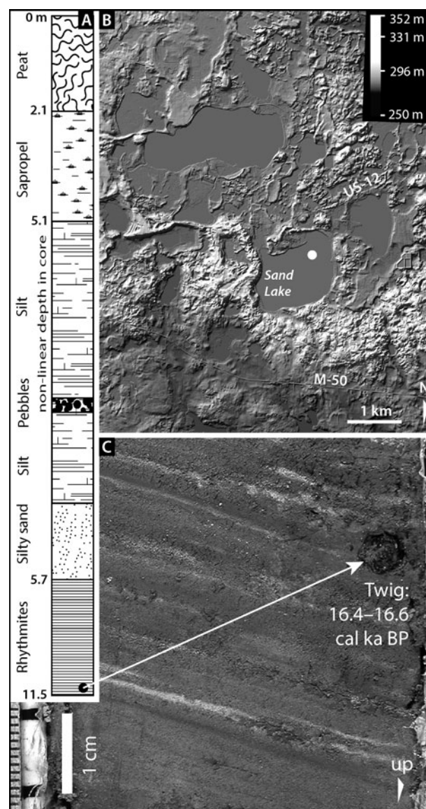
Figure 5. Geomorphology and sediment core from Sand Lake, Lenawee Co., Michigan (Fig. 1, Table 1). (A) Sediment core lithology, note non-linear depth scale. (B) Digital elevation model of Sand Lake, with core site indicated by white circle. (C) Rhythmically laminated sand, silt, and clay with radiocarbon dated twig identified. Approximately 1000 rhythmites were counted above the twig.
