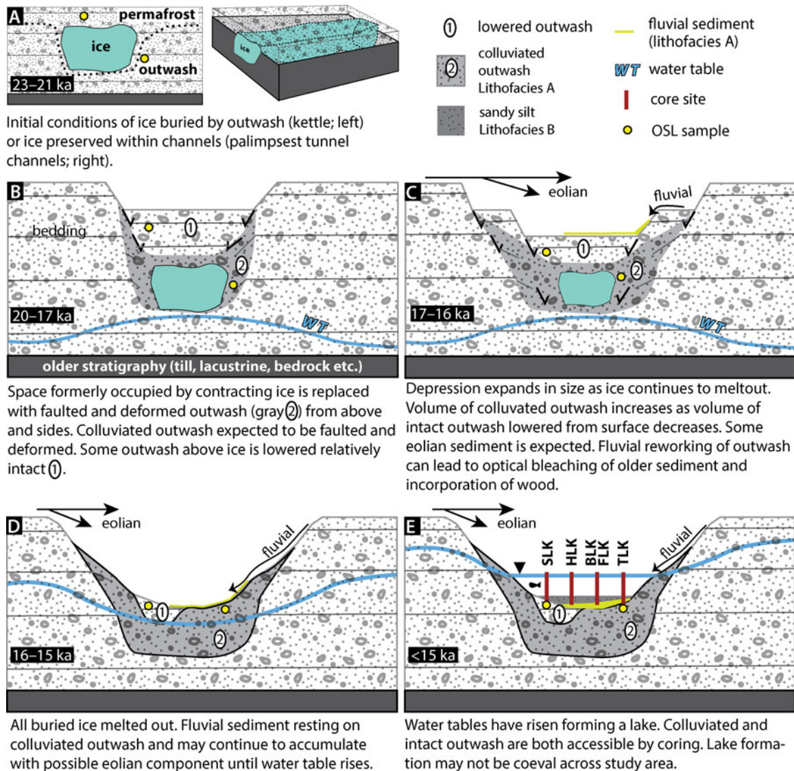
Figure 6. Model of buried ice melt-out to form kettles or depressions within palimpsest tunnel channels. For the example shown, the time sequence is for a kettle. The old ( 23.6 \pm 2.2 and 20.4 \pm 2.2 ka) optically stimulated luminescence (OSL) ages require sunlight exposure (resetting) of sand at that time recording deglaciation (panel A). During ice-block melt-out the sand may be faulted or deformed (colluviated outwash) or passively be lowered into a position on which lacustrine sediment eventually accumulates. Yellow dots are the two oldest OSL samples in outwash that can be traced through the kettle's evolution. Preservation of OSL signal can occur when sediment is not fully reset during this process (cores SLK and TLK), but when outwash is adequately exposed and reset, there is evidence of younger wood fragments being mixed into it through fluvial or mass-wasting processes (cores HLK, BLK, and FLK). Color version of figure is online. (For interpretation of the references to color in this figure legend, the reader is referred to the web version of this article.)
