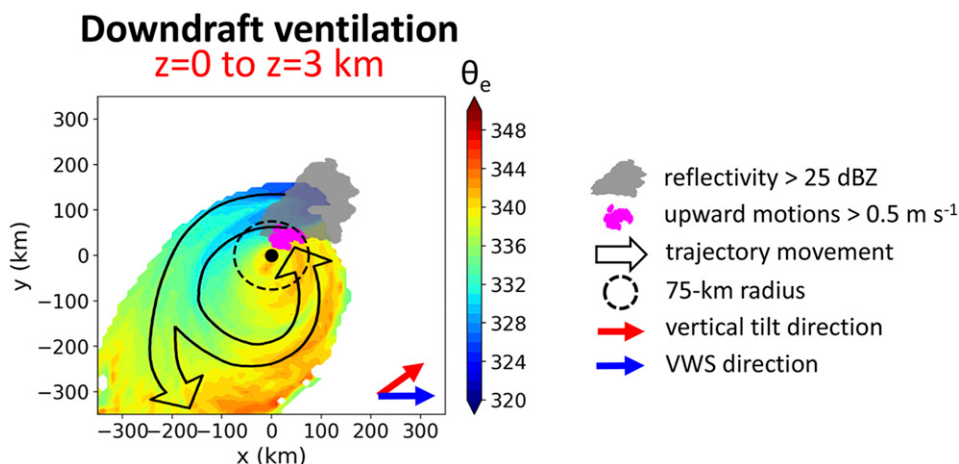
FIG. 17. Conceptual model of downdraft ventilation based on the RH50S10 experiment showing the average equivalent potential temperature of trajectories initialized in downdraft ventilation regions (K, colored shading), reflectivity greater than 25 dBZ (gray shading), upward motion greater than 0.5 \text{ m s}^{-1} (magenta dots), parcel movement (black arrows), the inner 75 km (dashed circle), the vertical tilt direction from the surface to 6 km (red arrow), and the VWS direction (blue arrow). The reflectivity and vertical velocity are time averaged during the bifurcation time period.
