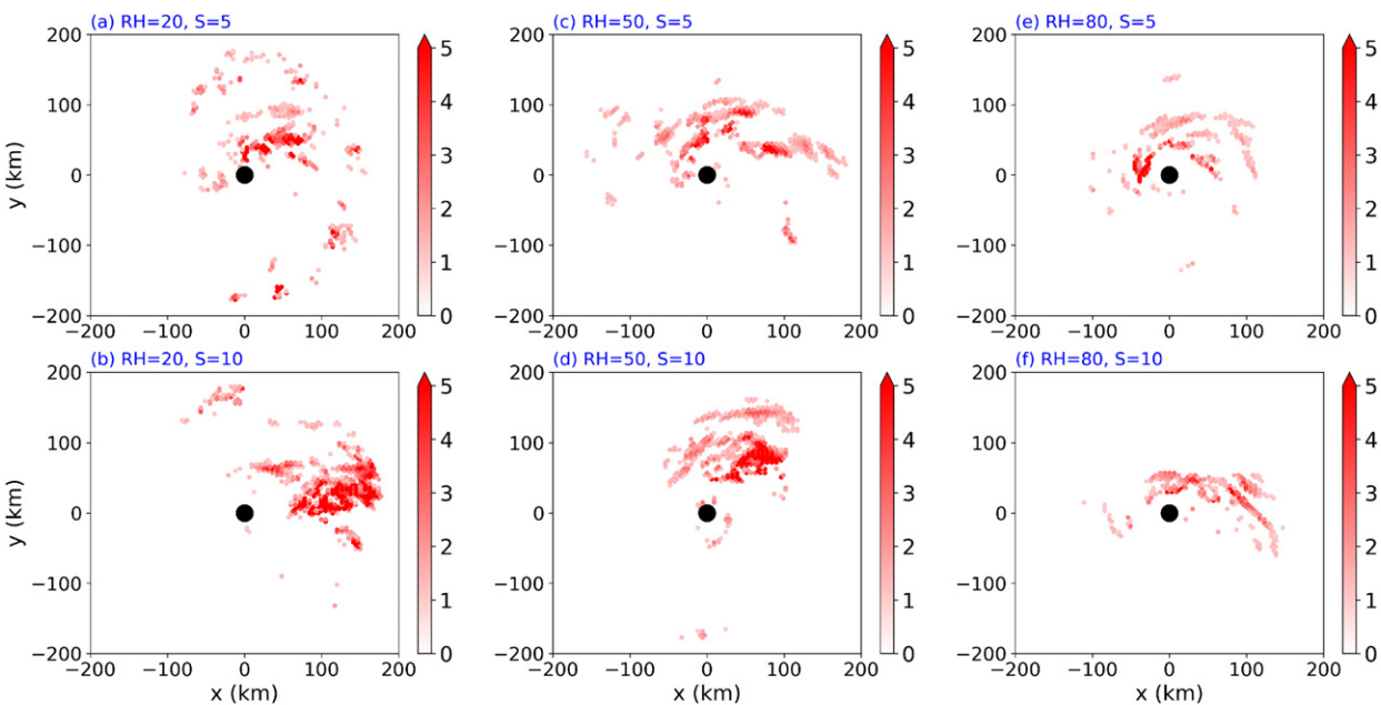
FIG. 11. Trajectory initialization locations (red dots) in downdraft ventilation ( \text{kg K m}^{-2} \text{s}^{-1} ) for the S05 and S10 experiments in the bivariate parameter space. Trajectories were initialized at the beginning of each bifurcation time period, at a height of 1 km, within the inner 180 km, and for an initial downdraft ventilation magnitude of at least 1 \text{ kg K m}^{-2} \text{s}^{-1} . Every two trajectory initialization locations are plotted. The black dot in each panel represents the center of the TC at the lowest model level.
