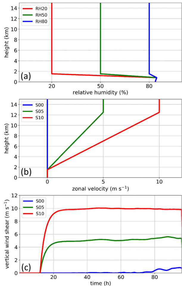
FIG. 1. (a) Vertical profile of relative humidity for RH magnitudes of 20% (red), 50% (green), and 80% (blue). (b) Vertical profile of the zonal wind for VWS magnitudes of 0 (blue), 5 (green), and 10 (red) \text{m s}^{-1} . (c) Time series of the VWS magnitude. The large-scale wind profiles are nudged toward the VWS magnitudes in (b) starting at 12 h, with a relaxation time scale of 3 h.
