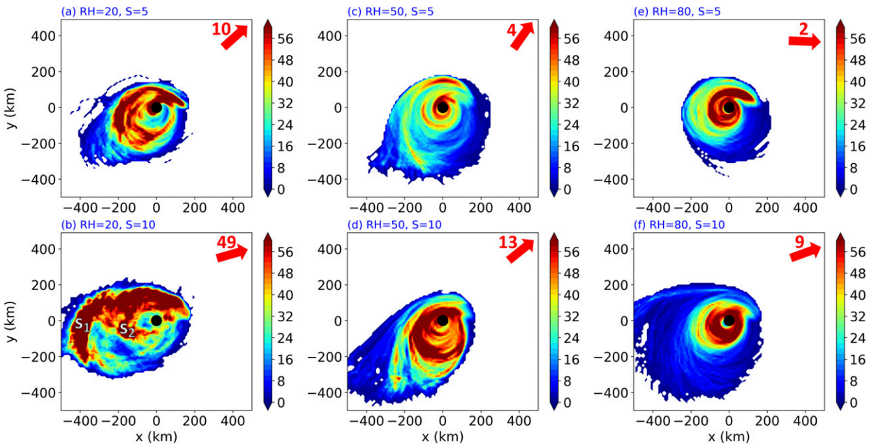
FIG. 7. Number of radial ventilation trajectories ( \times 10^{-2} ) from Fig. 6 passing through a location below a height of 3 km during the 24-h integration. The number has been normalized by the total number of trajectories initialized listed in Table 1.
