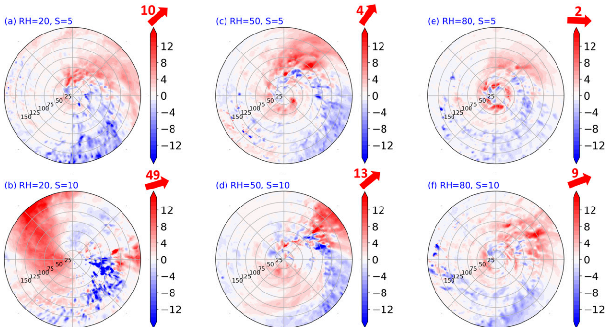
FIG. 2. As in Fig. 1, but at a height of 3 km. The S00 experiments are not shown. Recall that the VWS direction is westerly for all experiments.
