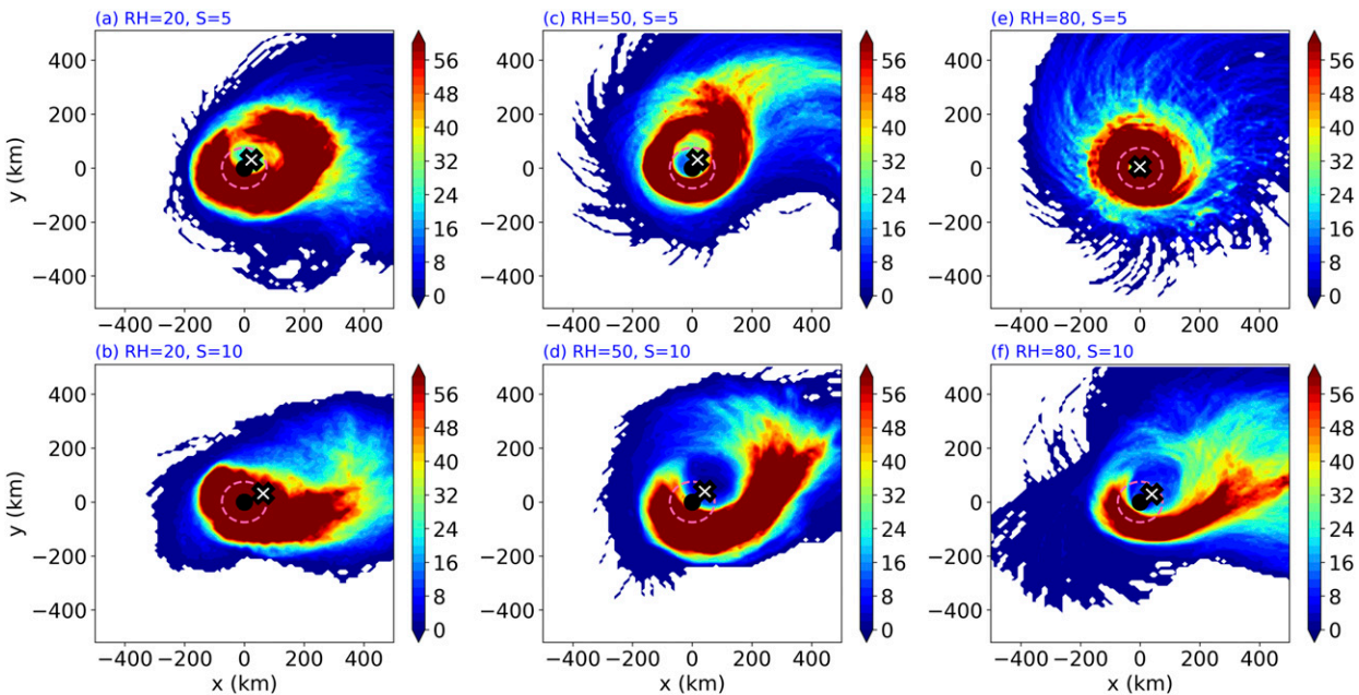
FIG. 10. Number of radial ventilation trajectories ( \times 10^{-2} ) from Fig. 9 passing through a location above 2 km during the 24-h integration. The number has been normalized by the total number of trajectories initialized listed in Table 2. The white \times in each panel represents the TC center averaged between heights of 5 and 9 km. The dashed pink circle represents the inner core with respect to the low-level center.
