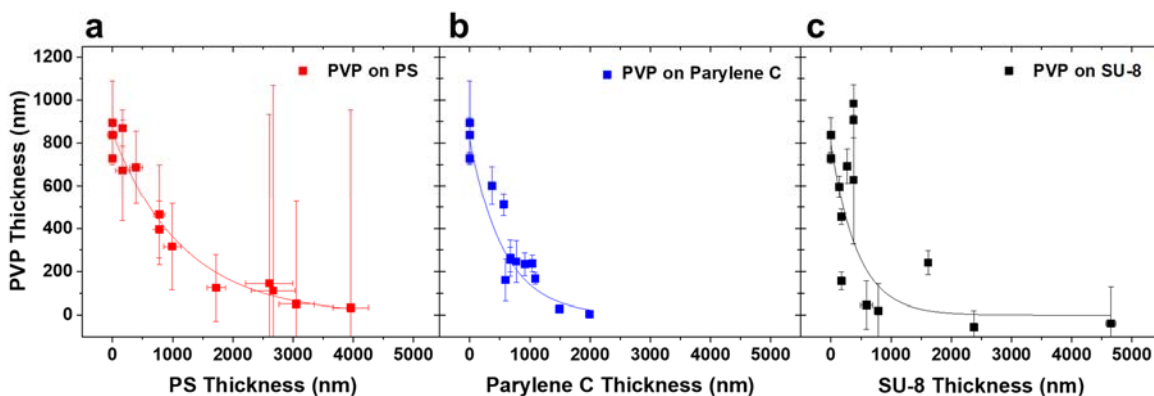
Figure 1. (a) 1 wt% PVP sprayed at 0.1 mL/hr for 60 min in the humidity and temperature control chamber at 27°C with different thicknesses of PS-on-Si substrates. At the larger PS thicknesses, the amount of PVP deposited is very thin, so it becomes difficult to distinguish from the roughness of the PS sample leading to large deviations in the apparent measured thickness. The red trace shows an exponential decay fit of y = 846.9 \text{ nm} \cdot e^{(-x/1174.8 \text{ nm})} , R^2 = 0.96 . (b) 1 wt% PVP sprayed at 0.1 mL/hr for 60 min on Parylene C-on-Si substrates at varying thickness. Due to the conformal nature of vapor deposition, the horizontal error bars are not visible. The blue trace is an exponential decay fit of y = 815.6 \text{ nm} \cdot e^{(-x/567.4 \text{ nm})} , R^2 = 0.98 . (c) 1 wt% PVP sprayed at 0.1 mL/hr for 60 min on SU-8-on-Si substrates with different thicknesses. The black trace is an exponential decay fit of y = 796.0 \text{ nm} \cdot e^{(-x/440.6 \text{ nm})} , R^2 = 0.60 . Confidence ranges are listed in Table S1.
