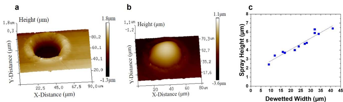
Figure 2. (a, b) 3D maps of a 90 mW, 0.25 NA laser dewetted PS feature before (a) and after (b) spray with PVP. (c) The height of the sprayed PVP feature after smoothing in ethanol vapor determined from AFM profiles. The linear fit has an equation y = 0.13x + 1.55 \text{ μm} , R^2 = 0.93 .
