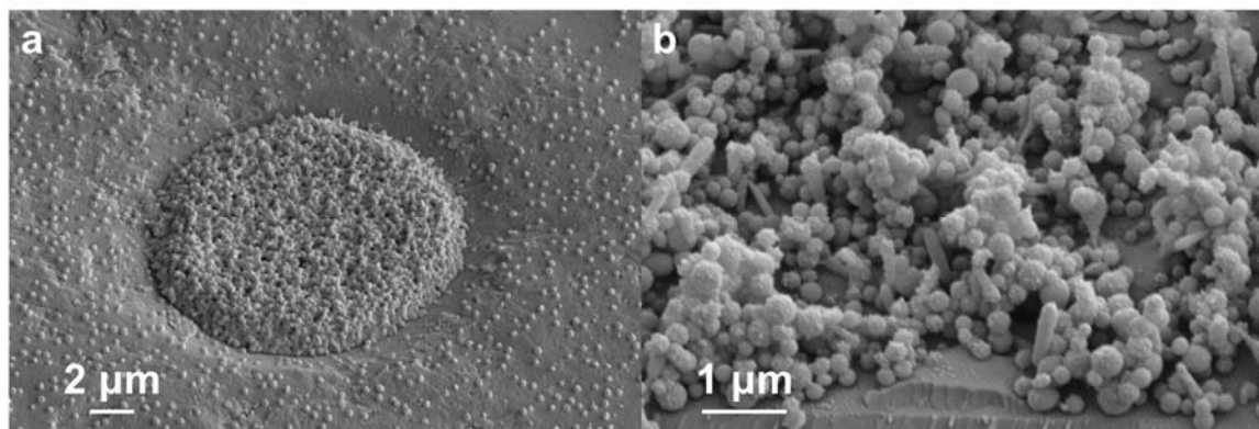
Figure 3. (a) Tilted scanning electron microscope (SEM) image of a FLaSk dewetted feature on PS created with 50 mW, 0.25 NA laser and sprayed with PVP. (b) Tilted SEM image of 0.25 wt% 10K PVP in 80 vol% ethanol to 20 vol% water sprayed at 0.5 mL/hr for 20 min.
