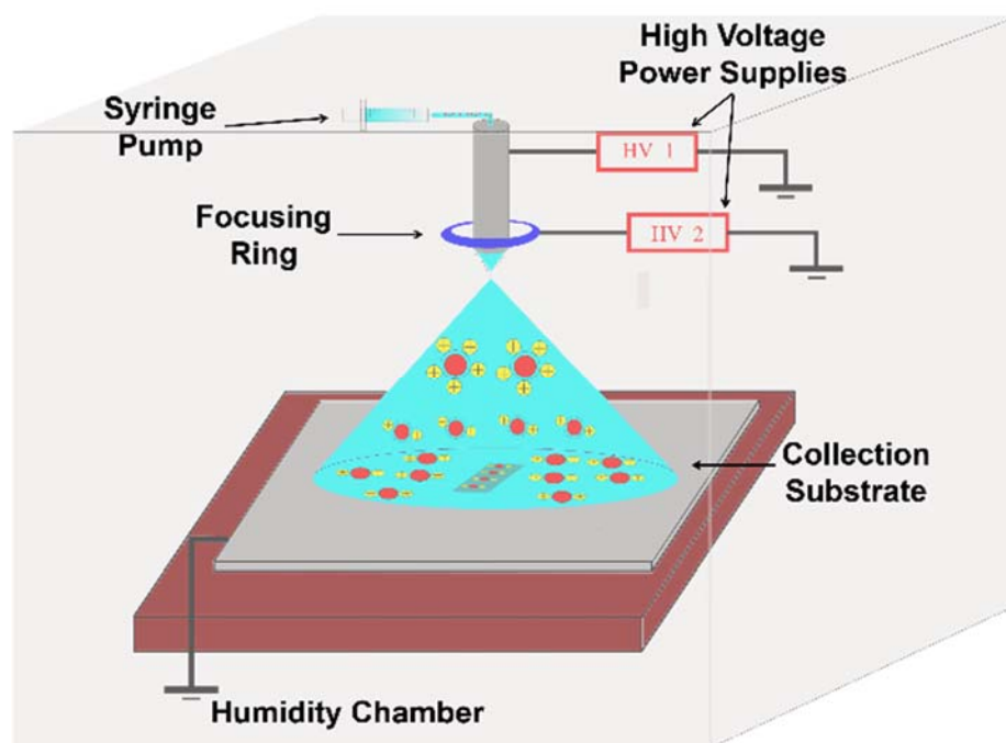
Figure 6. Schematic diagram of electrospray deposition setup.
