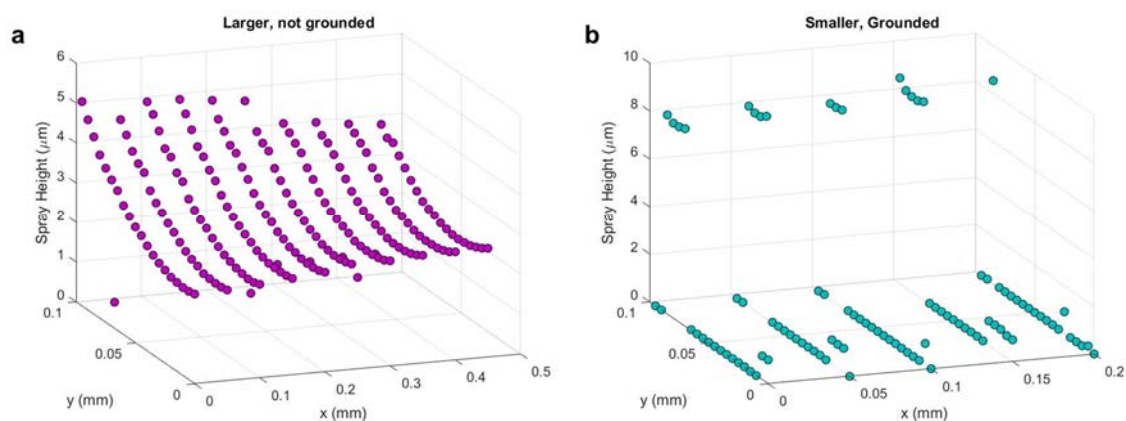
Figure 5. (a, b) Average thickness of sprayed PVP film on FLaSk dewetted SU-8 on Ti/Pt electrodes as seen in Fig. 4.
