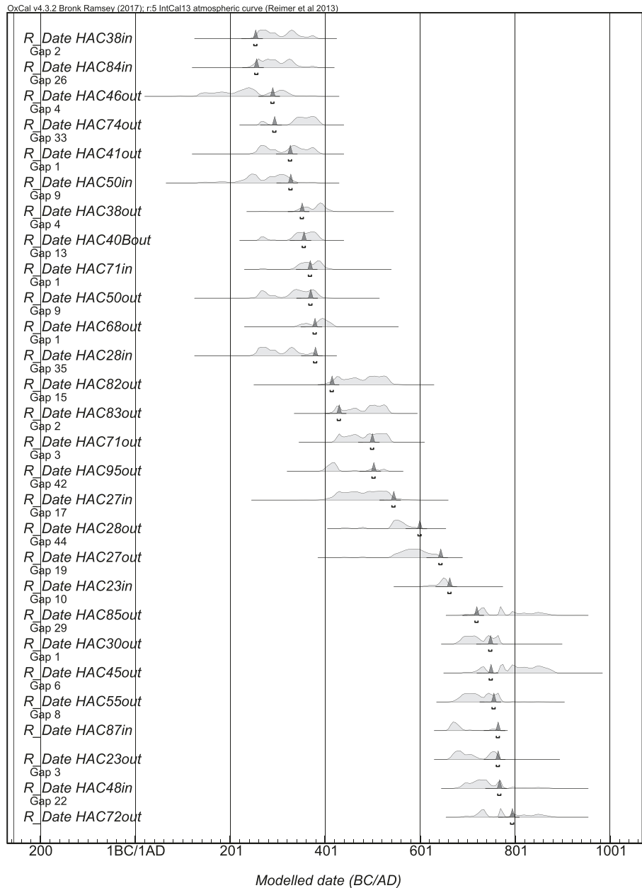
Fig. 5. Conventional modelled radiocarbon dates for the cross-dated Hundred Acre Cove samples using OxCal (Ramsey, 2017). Left column contains the sample IDs above the number of cross-dated years between the next consecutively dated sample. The light grey range shows the probability distribution of the sample's calibrated date based only off its radiocarbon age. The dark grey range is the improved \pm 10 year range modelled by comparing the full series of dates in the chronology against the IntCal13 calibration curve.
