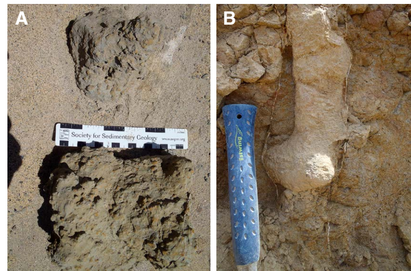
Figure 13. Terrestrial trace fossil bioturbation, fossiliferous terrestrial sequence (FTS), El Disecado Member, El Gallo Formation, Baja California, México. (A) Small traces referable to colonial arthropods such as termites (Hasiotis and Bown, 1992). (B) Large burrows referable to the crayfish ichnogenus Camborygina sp. (Hasiotis and Mitchell, 1993). Smaller traces tend to be oriented variably in space; larger trace fossils uniformly oriented vertically. In A, upper part of scale in inches; lower in cm. In B, blue handle is 19 cm in length.
